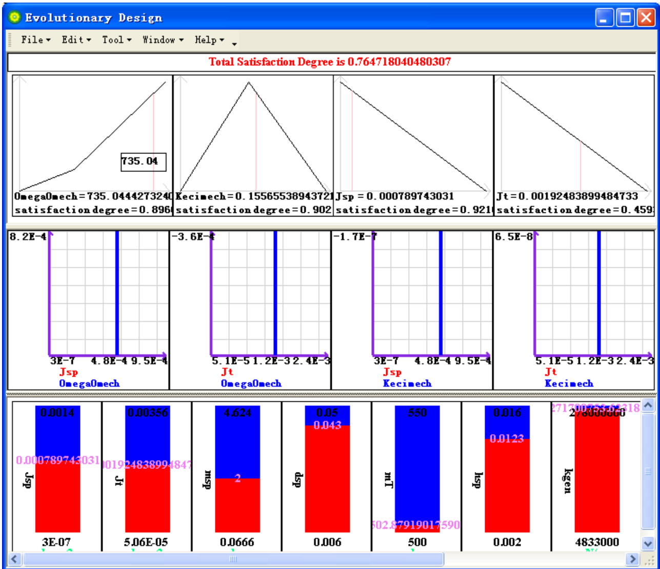
Fig.9 Analysis of sensitivities between goal variables and specification variables in transmission module
