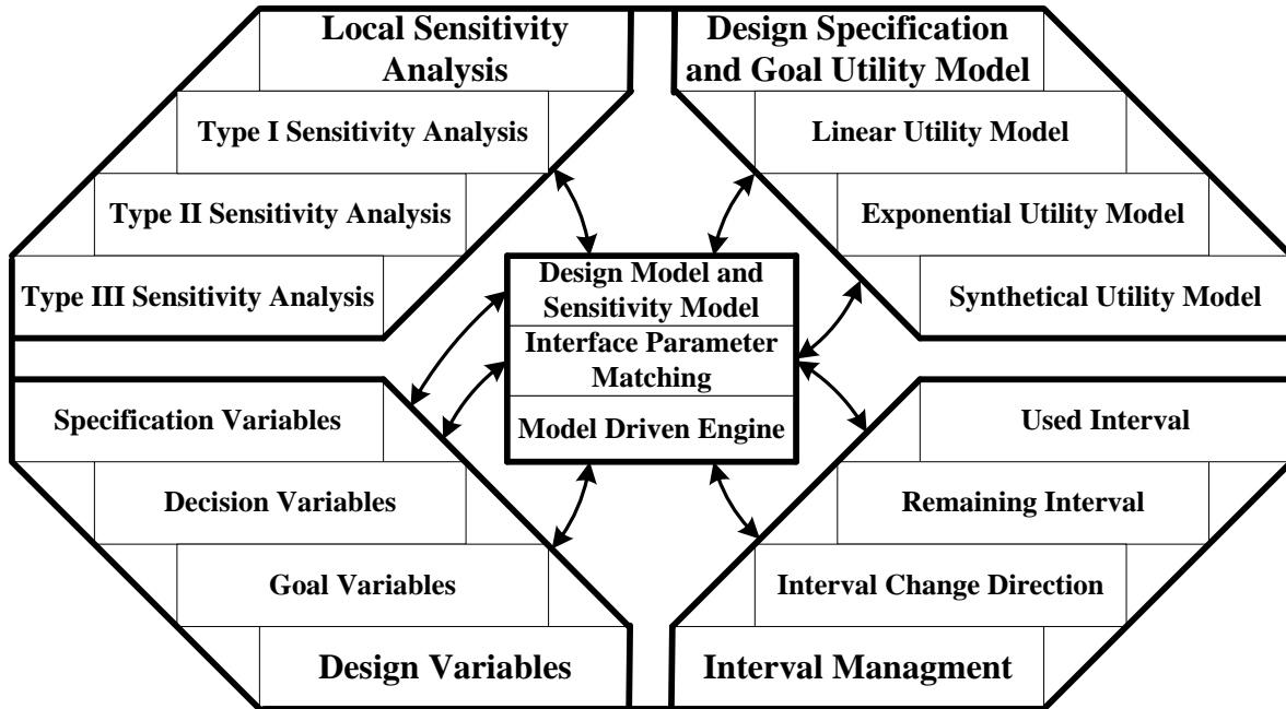
Fig.5 Architecture based on interval and sensitivity analysis for propagation parameter design
