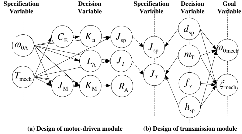
Fig.6 Decomposed design tasks for speed design of feeding servo system
