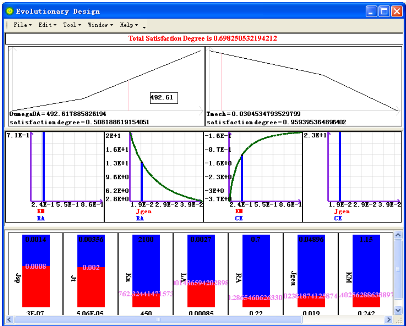
Fig.10 Analysis of sensitivities between decision parameters in motor-driven module
