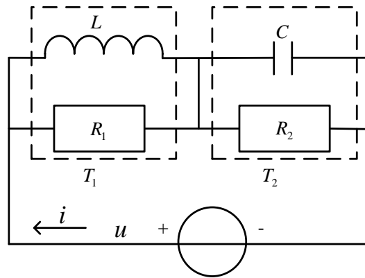
Fig.1 A simple design case of concurrent coupling
