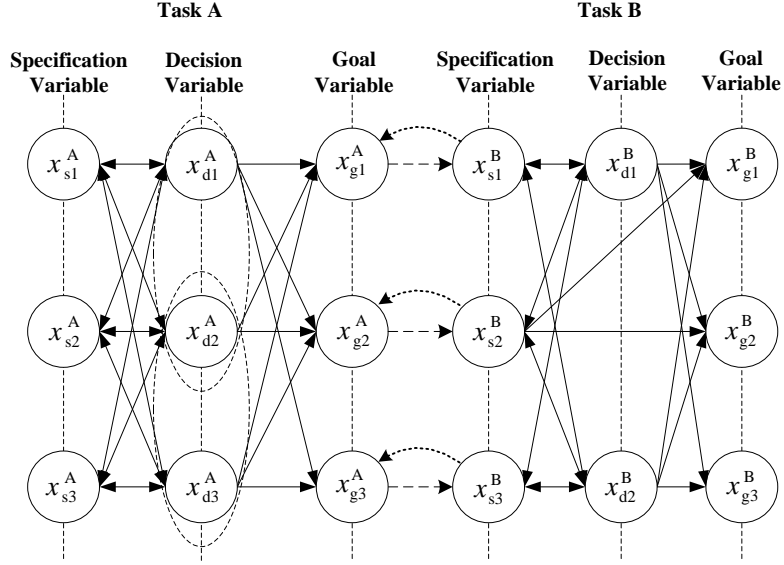
Fig.3 Decision and dependence model for coupled design tasks caused by parameter propagation
