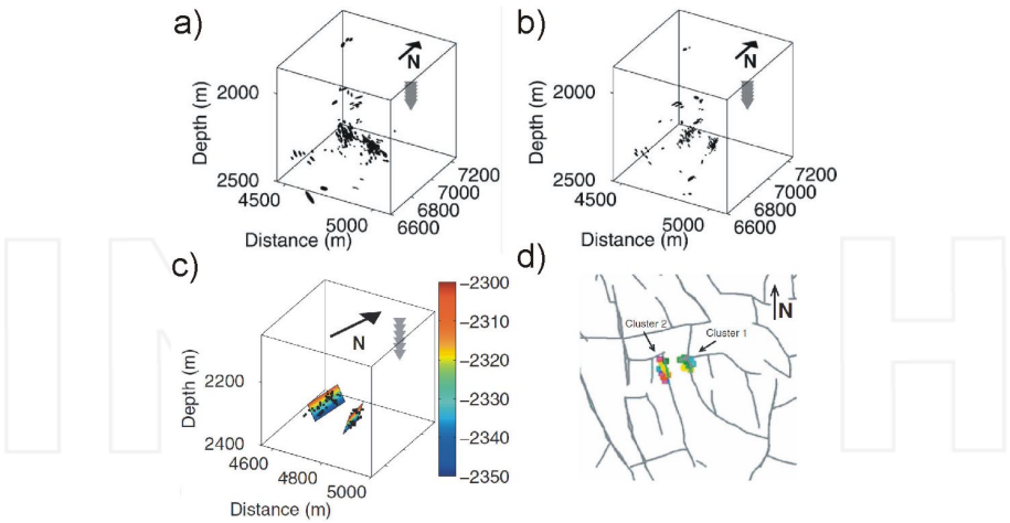
Figure 3. Microseismic events contain a wealth of information that can be used to determine planes of weakness along which fluid migration could occur. (a) Original source locations; (b) new source locations after application of a high-resolution relocation technique; (c) multiplets extracted and best fault plane solutions depicted in two major clusters; (d) obtained fault planes overlain onto the top-reservoir fault map interpreted from 3D surface seismic data (after De Meersman et al., 2009).
