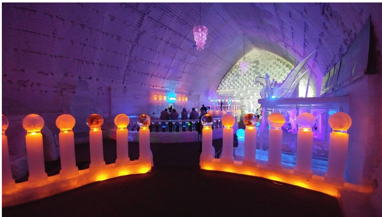
Figure A.11. The Ice Museum at Chena Hot Springs, kept cold year-round with a geothermally powered absorption chiller.
