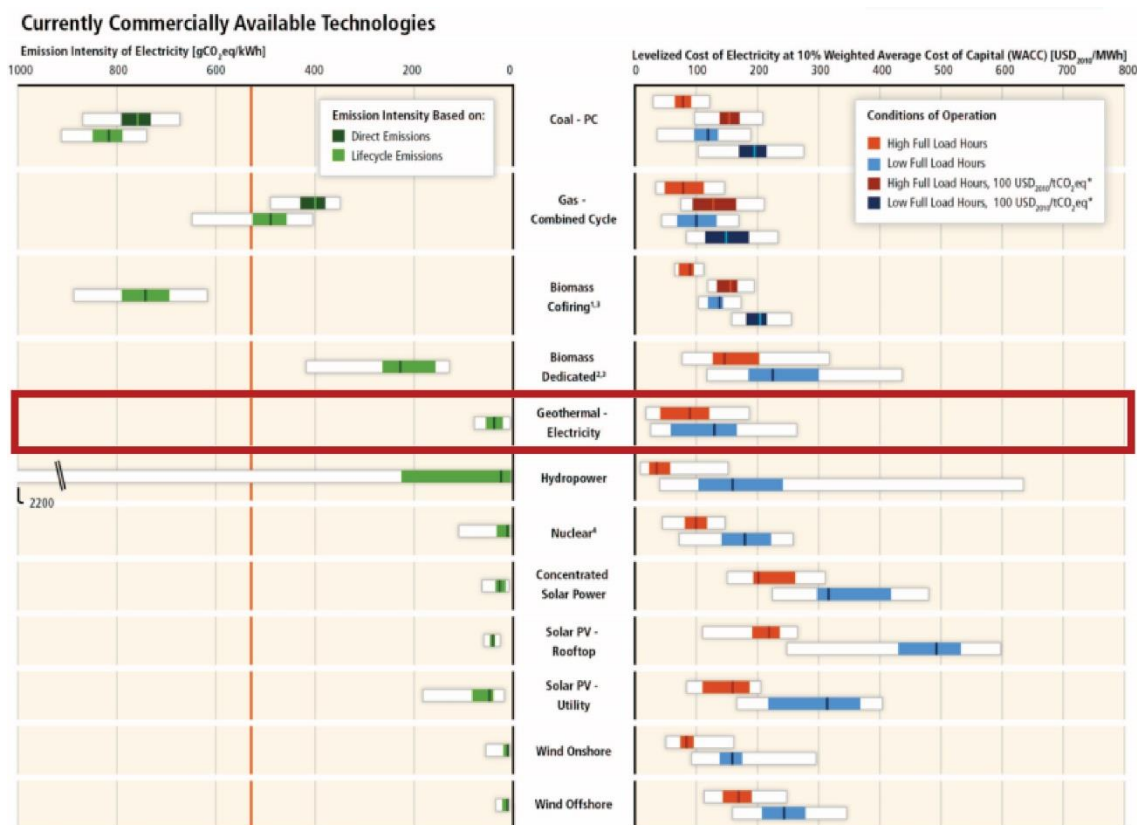
Figure 1.3. Lifecycle Emission Intensity and Levelized Cost of Electricity for several commercially available electricity generation technologies. Geothermal electricity produces very minor emissions (less than 75 gCO 2 eq/kWh) as compared to other baseload power sources. Geothermal electricity is, on average, cheaper than other renewable energy sources, and competitive with electrical generation with fossil fuels. Figure adapted from IPCC (2014b).
