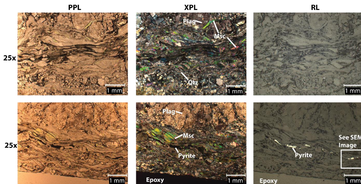
Figure 3.9. Photomicrographs of two perspectives of sample 113 under PPL, XPL, and RL at 25x magnification. Sample location is shown in Figure 3.1. In row 2, note the stringer of opaque (black) material under PPL and XPL that is highly reflective under RL. The white box in RL shows and area that was imaged with the SEM (Figure 3.10), which confirms it is pyrite. Abbreviations: Plag – plagioclase, Msc – Muscovite, Qtz – Quartz.
