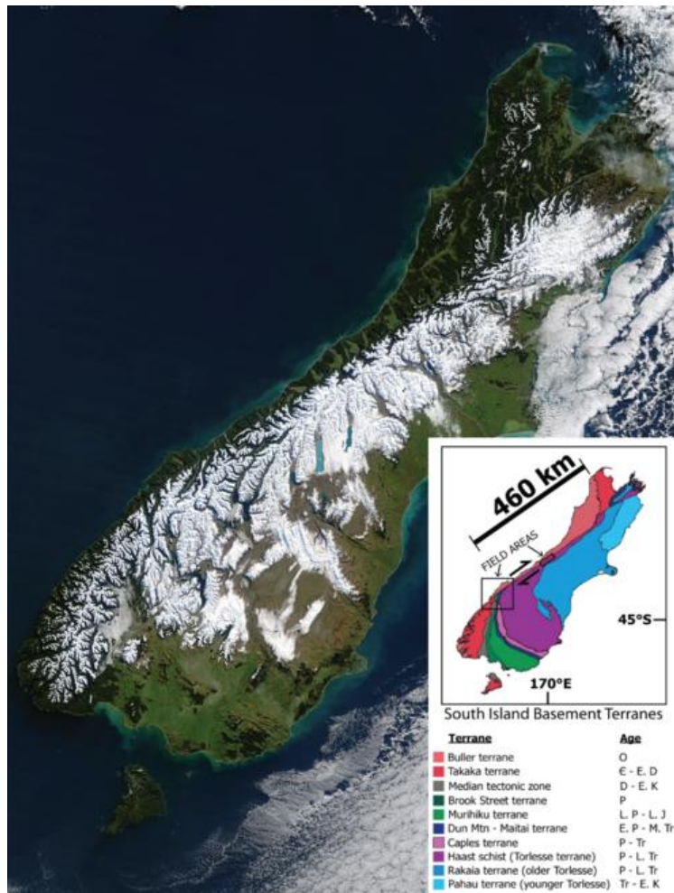
Figure A.59. The snowline after a major 2003 blizzard clearly delineates the Alpine Fault along the west coast thanks to rapid tectonic uplift on the eastern side of the fault (Source: NASA Earth Observatory). Inset shows the major basement rock terranes of NZ (Barth, 2013). The Dun Mountain - Maitai terrane (dark blue) is a key piercing point, offset by ~460km.
