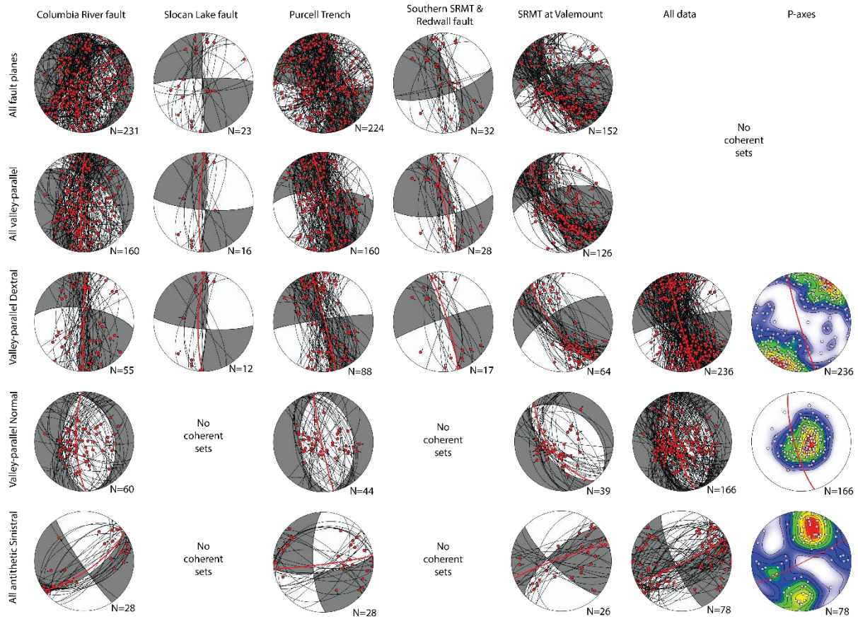
Figure 2.7. Equal angle lower-hemisphere beachball plots showing distinct subdomains of structural measurements for each collected in each major fault zone (columns 1-5), and for the entire dataset (columns 6). Column 7 shows contoured P-axes for the three largest kinematic populations; red indicates the densest cluster of P-axes. Row 1 shows all unfiltered fault planes, row 2 shows all valley-parallel ( <30^\circ to the regional trend) fault planes, rows 3 and 4 show all valley-parallel dextral and normal faults respectively. Row 5 shows all sinistral faults oriented at high angles ( >30^\circ ) to the valley, representing possible R' shears.
