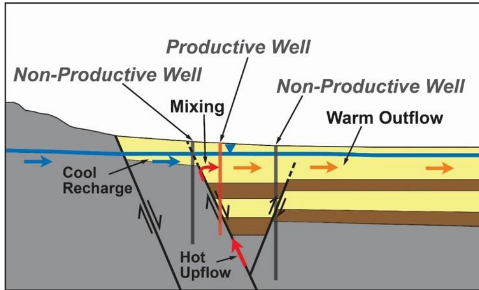
Figure A.34. Conceptual model of a blind geothermal system. Note how the cool recharge suppresses any surface manifestation of the hydrothermal system. Source: Richards and Blackwell (2002)
