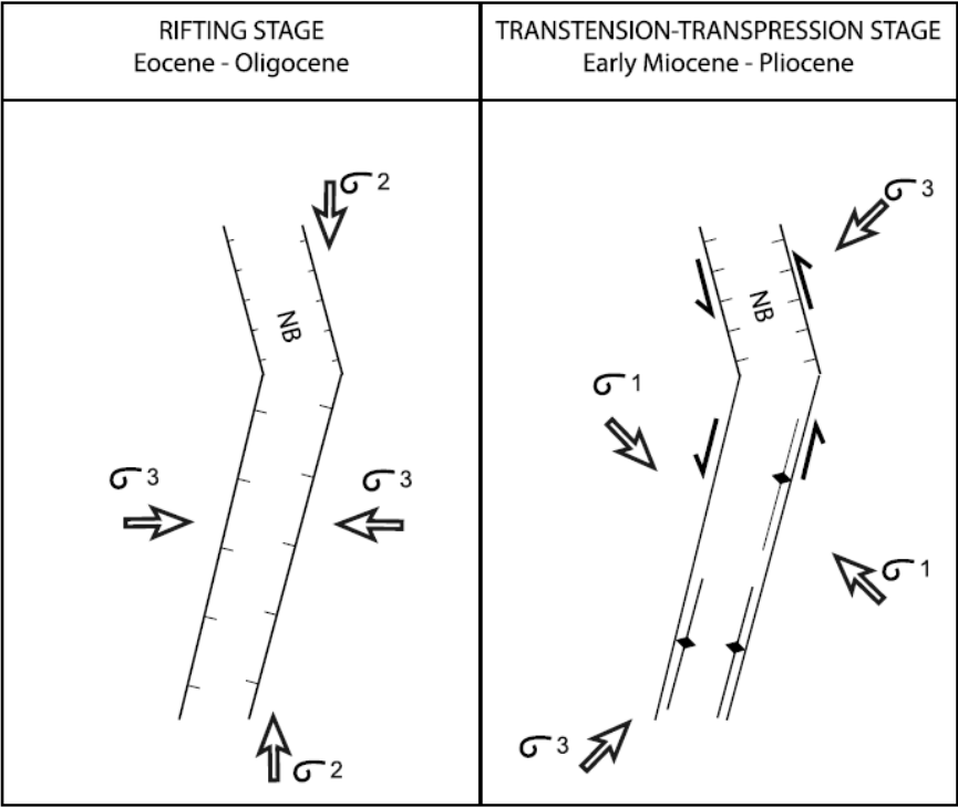
Figure A.0.43. Simplified stress history of the Upper Rhine Graben. Extension in the Eocene to Oligocene took advantage of pre-existing crustal weakness. This was followed by a transition to left-lateral transpression and transtension in the Miocene to Pliocene. Source: Rotstein and Schaming (2011).
