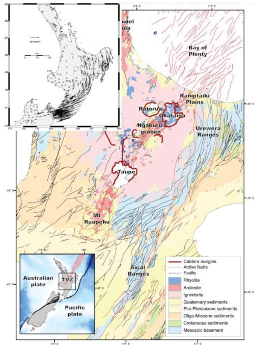
Figure A.54. Geologic map of the North Island, including the volcanoes and calderas of the Taupo Volcanic Zone, and extensional faults of the overlapping Taupo Rift (Villamor et al., 2017) . Upper left inset shows crustal velocities of the Pacific Plate relative to the Australian plate (Wallace et al., 2004). Note the clockwise rotation of the forearc, resulting in extension at the Taupo Rift, and transpression towards the south.
