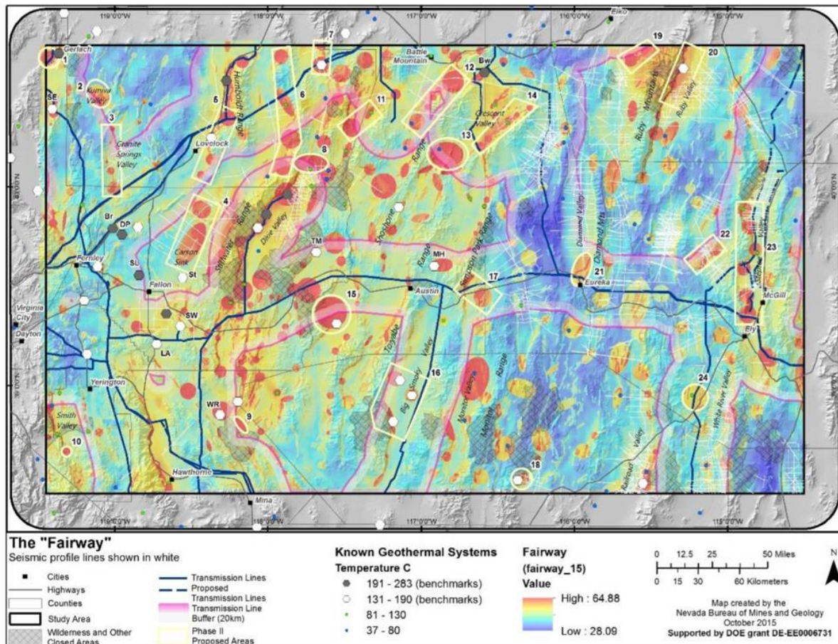
Figure A.33. Final product of the Play-Fairway analysis of the Great Basin. Most favourable areas for new geothermal development are highlighted in bright red, based on a statistical analysis of numerous layers of data. Source: Faults et al. (2016).
