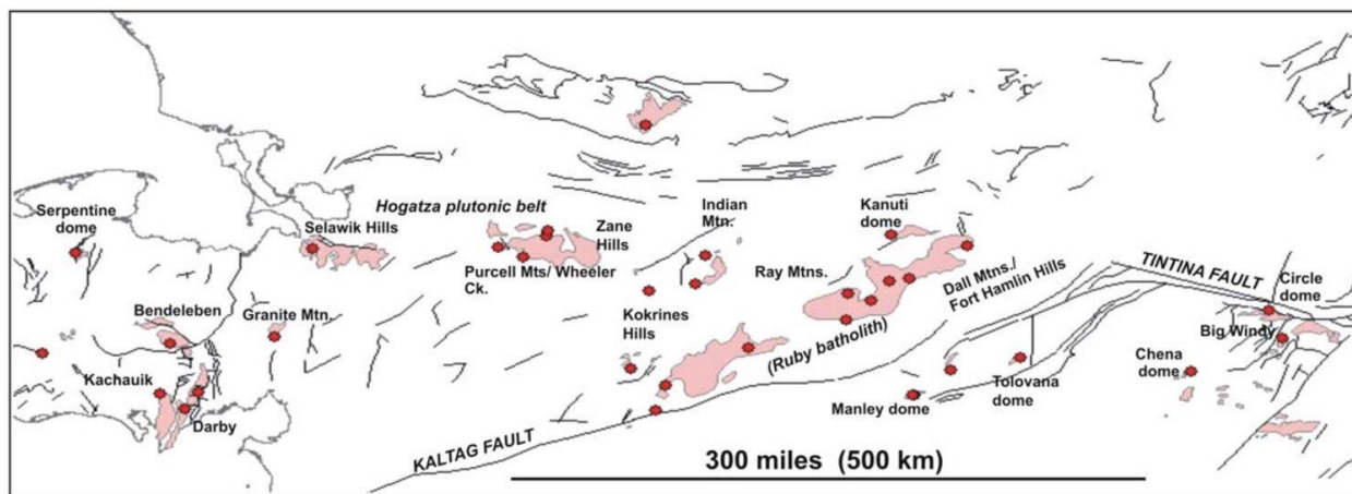
Figure A.6. The Central Alaska Hot Springs Belt, and associated plutons. Chena and Manley are in the bottom right. (Kolker, 2008). The Cretaceous plutons often form the core of “domes”, which are basically just rounded hills.
