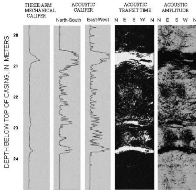
Figure A.29. Example of acoustic televiewer data displaying dipping fractures in a borehole. Zones with intense fracturing may act as conduits for hydrothermal waters. Source: Williams and Johnson (2004)
