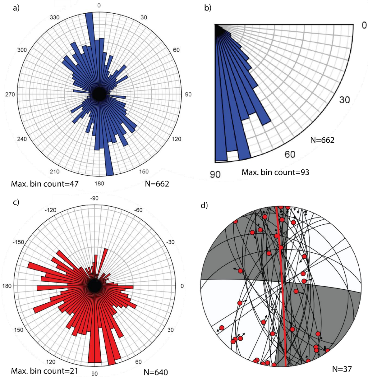
Figure 2.8. a) Bidirectional equal-distance circular histogram of the strikes of all 662 fault planes measured in this study. The strong NNW-SSE population is apparent, as is the subsidiary NE-SW population at high angles to the valleys. b) Unidirectional equal-distance quadrant histogram of the dips of all fault planes measured in this study. The majority are steeper than 60°. c) Unidirectional equal-distance circular histogram showing rake of slickenlines on fault planes using the standard convention of hanging-wall motion relative to the foot-wall, such that 0° = sinistral, +90° = normal, 180° = dextral, and -90° = reverse. The largest populations are normal and dextral. d) Kinematics of large fault planes with observable damage/fracture zones, and/or gouge layers greater than 1cm in width. These large faults are dominantly north-south striking, steeply-dipping, and dextral.
