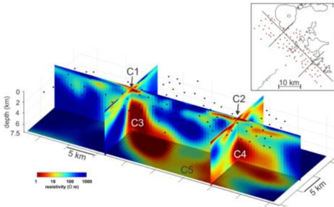
Figure A.56. Magnetotelluric resistivity model of the Taupo Volcanic Zone, showing the deep roots of the hydrothermal system (Heise et al., 2016). Models like this are useful for locating potential supercritical geothermal resources, as well as understanding the long term evolution of the earth's plumbing system.
