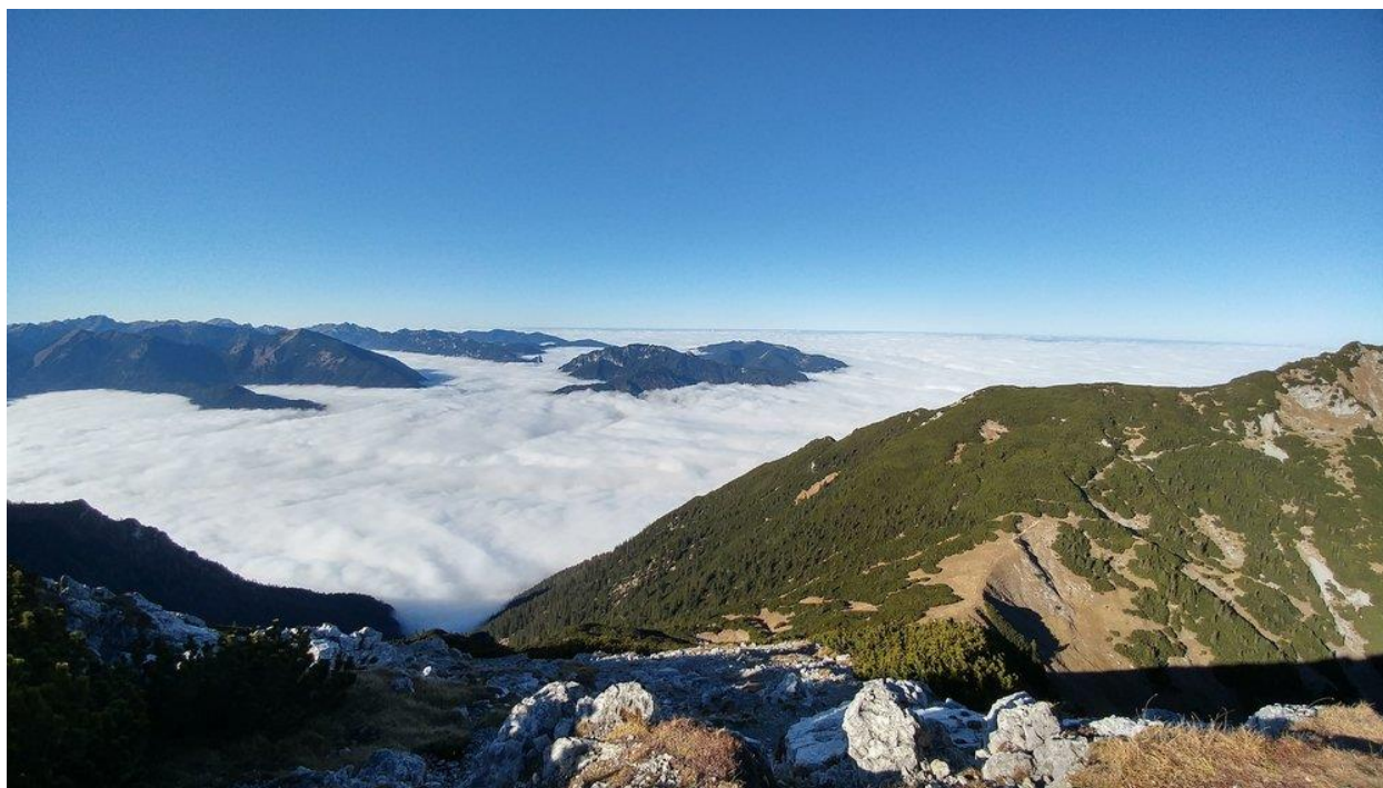
Figure A.49. View northwest from Bischof peak in the Bavarian Prealps. Munich is in the distance on the right, hidden beneath the fog. The geology, morphology, and vegetation of these mountains were very reminiscent of the front ranges of the Canadian Rockies.
