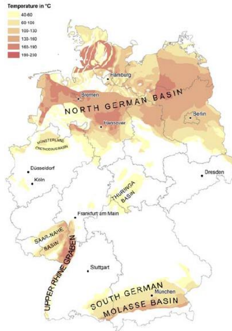
Figure A.42. Regions with potential geothermal resources in Germany. Main regions are the North German Basin, Molasse Basin, and Rhine Graben. Source: Agemar et al. (2014).
