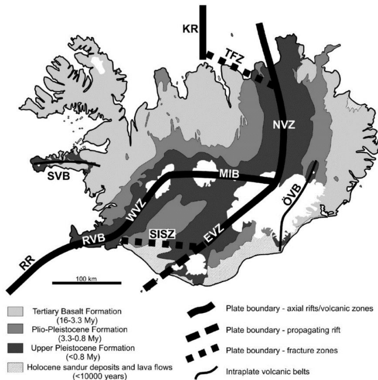
Figure A.27. Major crustal boundaries in Iceland. Note the Tjornes Fracture Zone (TFZ) offshore to the north of the north-south orientated Eyjafjordur. North-south oriented faults in Eyjafjordur may be the hosts of hydrothermal reservoirs. Source: Thordarson and Larsen (2007)
