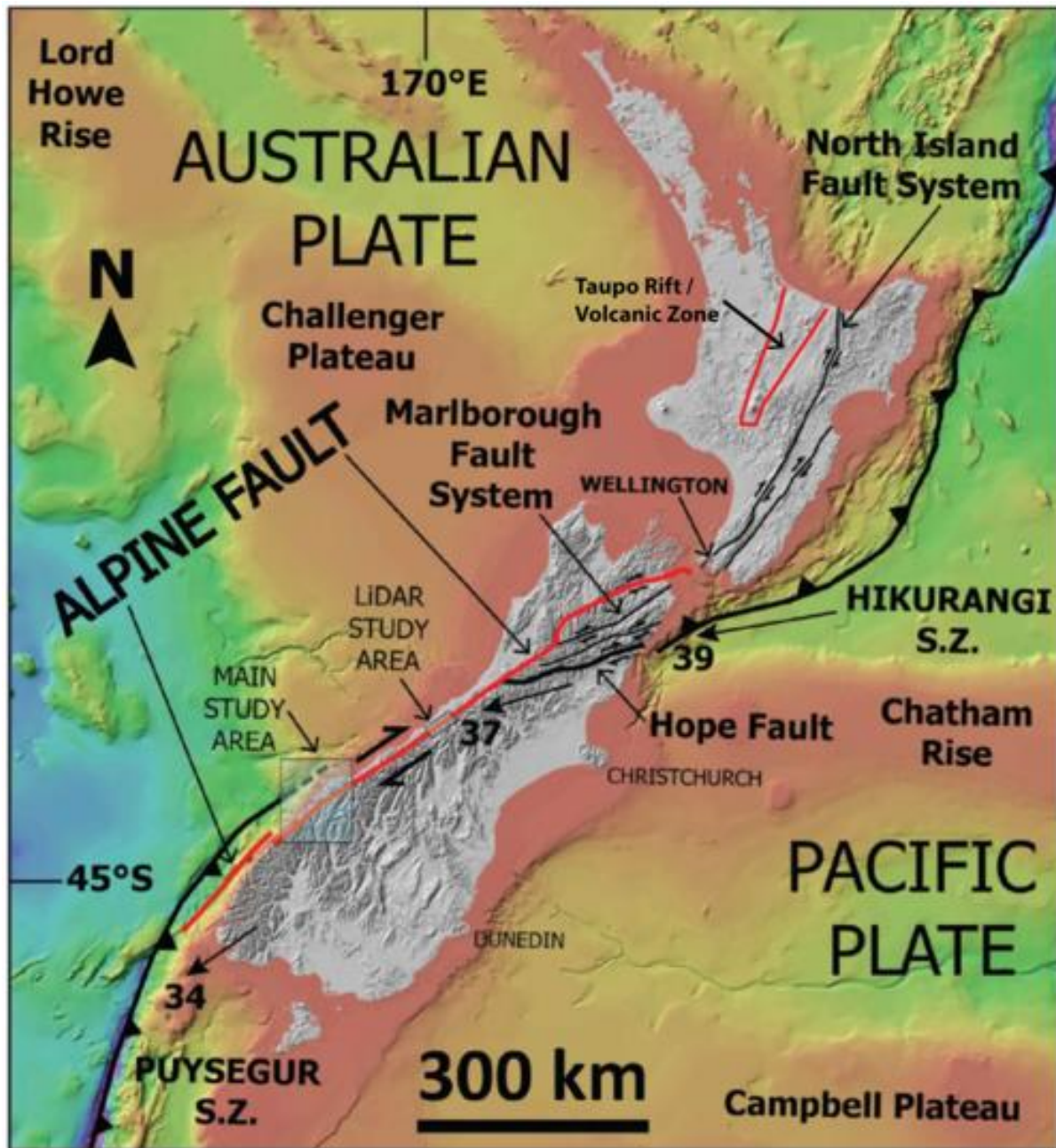
Figure A.52. Tectonic setting of New Zealand adapted from Barth (2013), showing the west-dipping Hikurangi Subduction Zone, the approximate outline of Taupo Rift / Volcanic Zone, the dextral Marlborough Fault System and Alpine Fault, and the east-dipping Puysegur Subduction Zone.
