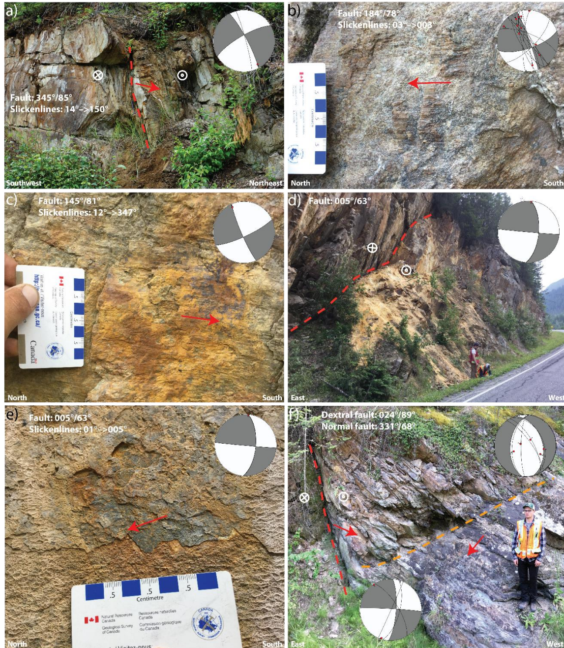
Figure 2.11. Photos from the Purcell Trench. See Figure 2.5 and Figure 2.6 for photo locations. Beachballs show kinematics for each fault plane. Concentric circles indicate movement out of the page, circles containing an 'x' indicate movement into the page. a) Breccia and gouge zone at outcrop of the Adit fault near Beaton (lat. 50.7025^{\circ}\text{N} , long. 117.7095^{\circ}\text{W} ). Dextral slickenlines ( 14^{\circ} \rightarrow 150^{\circ} ) are present on a subvertical, limonitic fault plane ( 345^{\circ}/85^{\circ} ). Rock hammer for scale. b) One of numerous dextral slickenlines ( 03^{\circ} \rightarrow 003^{\circ} ) observed on vertical fault zone ( 184^{\circ}/78^{\circ} ) along Duncan Lake (lat. 50.4164^{\circ}\text{N} , long. 116.9591^{\circ}\text{W} ). c) Dextral slickenlines ( 12^{\circ} \rightarrow 347^{\circ} ) on a limonitic subvertical fault plane ( 145^{\circ}/81^{\circ} ) located 10 km north of Duncan Lake (lat. 50.6958^{\circ}\text{N} , long. 117.1007^{\circ}\text{W} ). d) Dextral fault zone ( 005^{\circ}/63^{\circ} ) on the western shore of Kootenay Lake
