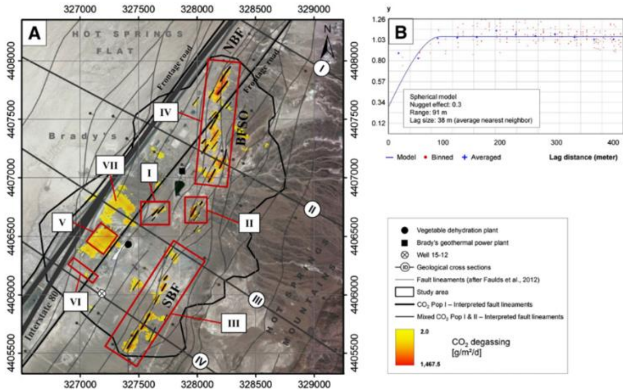
Figure A.51. Map of CO 2 emissions near the Brady's geothermal system in Nevada. Note how closely the anomalies match mapped fault traces. Source: Jolie et al. (2015).
