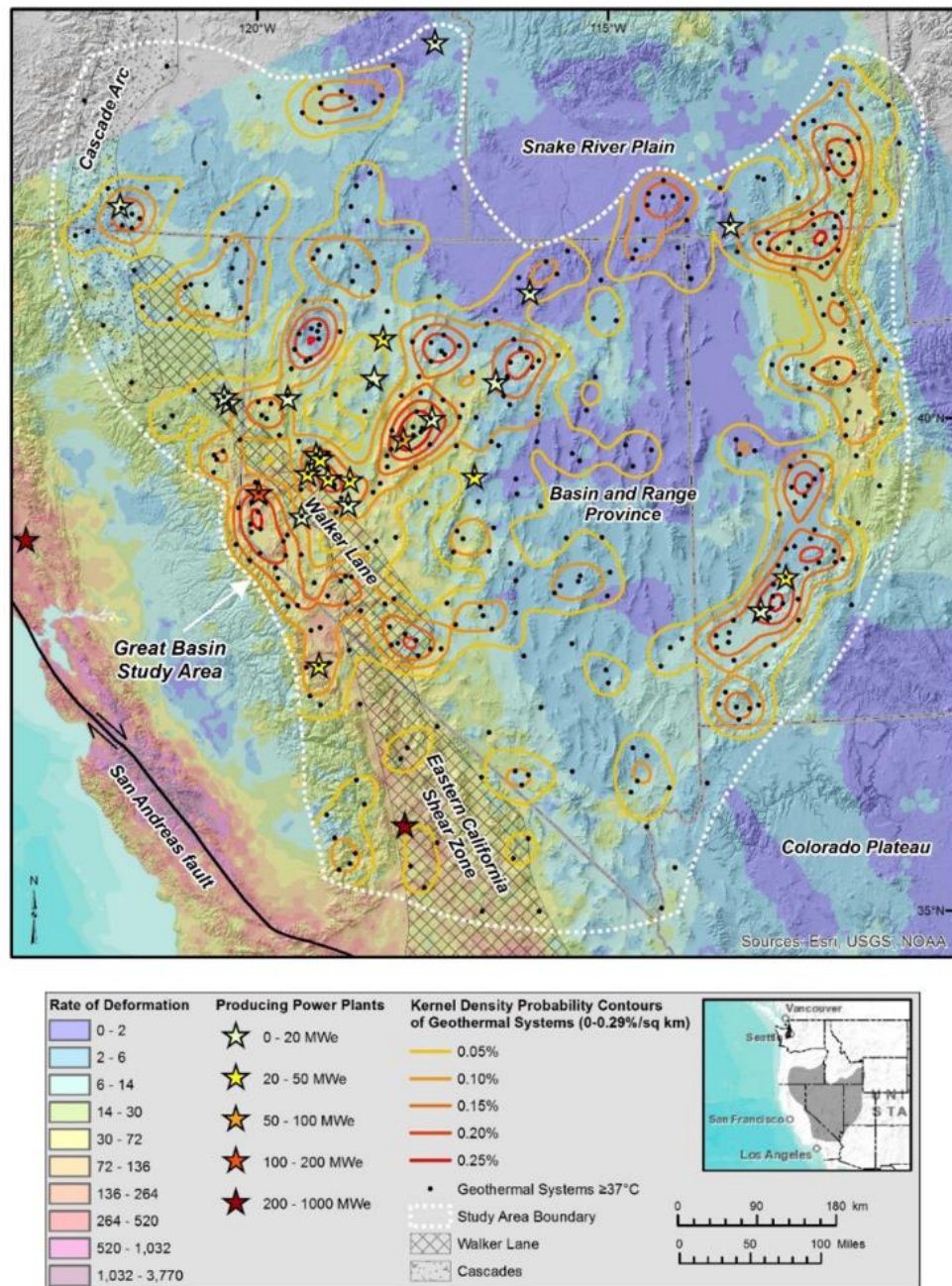
Figure A.31. Geothermal systems and regional tectonic setting of the central-western United States. The Basin and Range geologic province is characterized by north-south trending horsts (ranges) and grabens (basins). The majority of dextral shear strain between the Pacific and North American plates is accommodated on or near the San Andreas fault, with a minor component on the Eastern California Shear Zone and Walker Lane. Note that Nevada hosts the greatest number of geothermal power plants, but the largest power producers are in California. Source: Faults and Hinz (2015)
