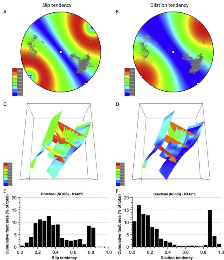
Figure A.44. Results from a Slip and Dilation Tendency Analysis performed by Meixner et al. (2016) on 3D fault model of the Bruchsal geothermal system near Karlsruhe. You can see that the WNW-ESE oriented faults are much more likely to slip and dilate, indicating that they may be more favourable fluid paths.
