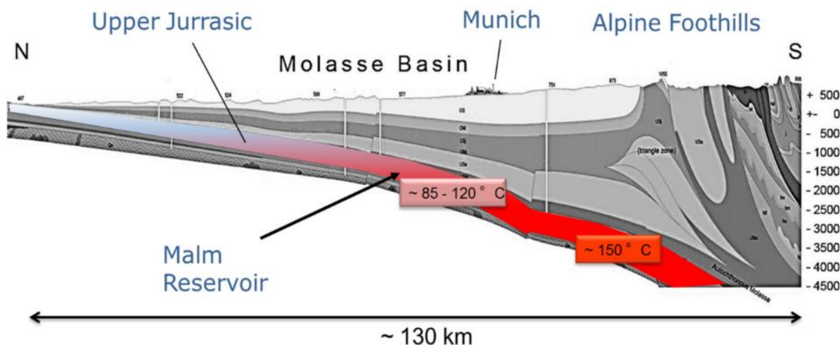
Figure A.46. Simplified cross-section of the Alpine foothills and foreland near Munich. The Jurassic Malm formation contains a significant volume of hot water, increasing in temperature to the south. Source: Farquharson et al. (2016).
