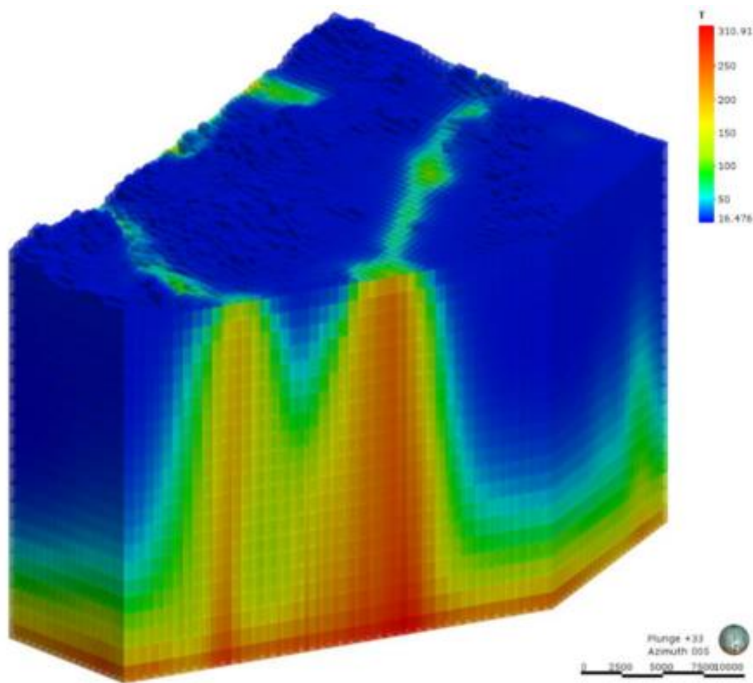
Figure A.58. Results from a TOUGH2 flow simulation that suggest that the locations of high-temperature geothermal resources in New Zealand may be controlled by subtle topographic lows (Pearson-Grant et al., 2017).
