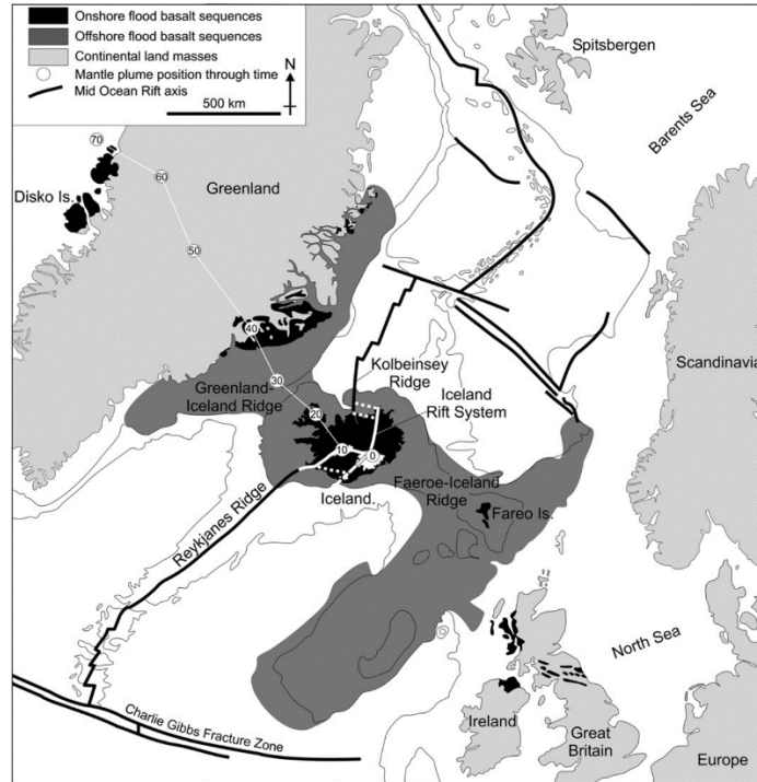
Figure A.18. Tectonic setting of Iceland in the northern Atlantic. Note how the Iceland Rift System steps out east from the trend of the submarine Reykjanes and Kolbeinsey Ridges. Circled numbers indicate the location of the mantle plume over the past 70 million years. Source: Thordarson and Larsen (2007).
