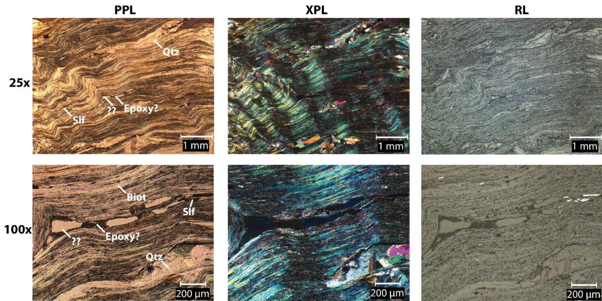
Figure 3.15. Photomicrographs of sample 138 under PPL, XPL, and RL at 25x and 100x magnification.
