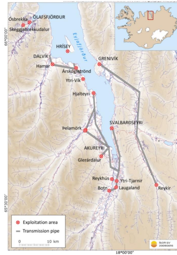
Figure A.23. Map of the district heating system serving Akureyri and surrounding settlements in Eyjafjörður. Source: Flóvenz et al., (2010)
