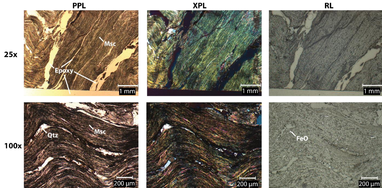
Figure 3.20. Photomicrographs of sample 144 at 25x and 100x magnification. Sample location is shown in Figure 3.1. In row 1, epoxy is shown filling 50μm to 1 mm wide fractures. One such fracture is imaged with the SEM in Figure 3.21a. The optical characteristics of epoxy at the bottom edge of the thin section is shown for comparison to the fracture-filling epoxy. In row 2, minor layers of quartz are shown between muscovite. Abbreviations: Msc – Muscovite, Qtz – Quartz, FeO – Iron Oxide.
