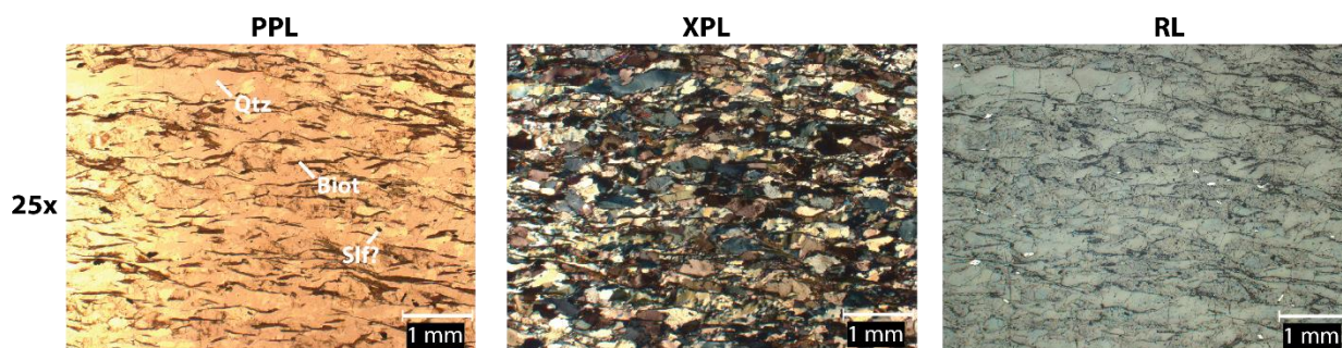
Figure 3.13. Photomicrographs of sample 117 under PPL, XPL, and RL at 25x magnification. Sample location is shown in Figure 3.1. Abbreviations: Qtz – Quartz, Biot – Biotite, Slf – Sulfide.
