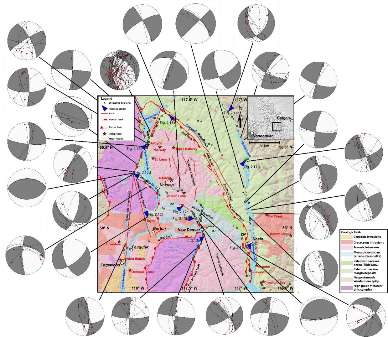
Figure 2.6. Geology of the Purcell Trench, Slocan Lake fault, and southern Columbia River fault, after Cui et al. (2017). Lower-hemisphere stereoplots ('beachballs') show fault plane (black great circles) and slickenline (red dots) orientations for subsets of stations data collected as part of this research . P (white) and T (grey) quadrants represent the average kinematics for each subset. Blue triangles point in direction of photos shown in Figure 2.11 Figure 2.12 Figure 2.13.
