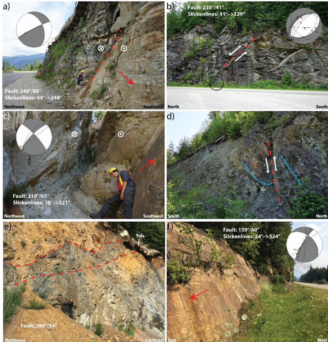
Figure 2.12. Photos from the Columbia River fault. See Figure 2.3 for photo locations. Beachballs show kinematics for each fault plane. Concentric circles indicate movement out of the page, circles containing an 'x' indicate movement into the page. a) View northeast at outcrop on Highway 23 above the southeastern abutment of the Revelstoke Dam (lat. 51.0486°N, long. 118.1901°W). A splay of the main Columbia River fault is exposed here and is reinforced with rebar and shotcrete. Dextral slickenlines (44°→248°) are present on the footwall of the splay fault (240°/88°). b) A set of SW-NE striking normal faults (fault: 235°/41°; slickenlines: 41°→329°) exposed near Mica Dam (lat. 52.0710°N, long. 118.5590°W). Person circled for scale. c) A wide (1.2 m) gouge zone exposed along Highway 23 near Halcyon Hot Springs (lat. 50.5217°N, long. 117.8998°W). Dextral slickenlines (10°→221°) are present on the fault walls (218°/65°). d) Fault originally mapped as a normal fault by Thompson et al. (2004b), reinterpreted as a reverse fault based on folded footwall and reverse slickenlines on the hanging wall. This fault occurs in a possible restraining bend of the
