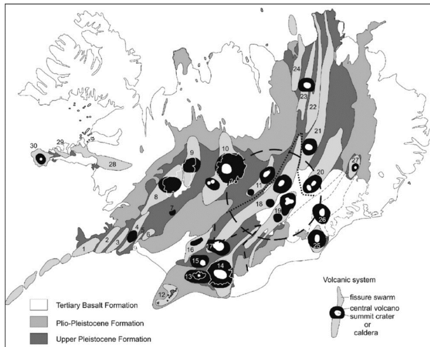
Figure A.19. Map of active volcanic systems in Iceland. Reykjanes-Svartsengi (1), Hengill (4), Krafla (23), and Theistareykir (24) all host high temperature geothermal power plants. Source: Thordarson and Larsen (2007).
