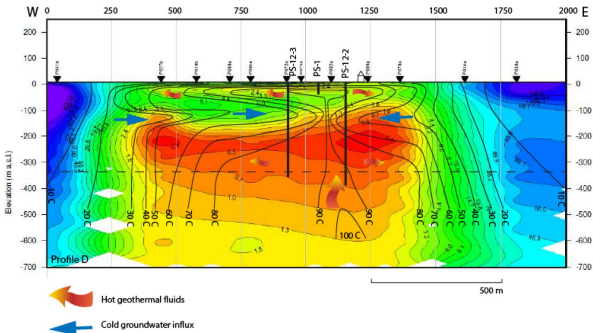
Figure A.16. Subsurface model of the Pilgrim Hot Springs geothermal system. Note that the geothermal reservoir is only at 300m depth in unconsolidated sediment, though the hot water is believed to emanate from a fault at greater depth, near the 100C isotherm, but the exact location is still unknown. Source: Miller et al., (2013).
