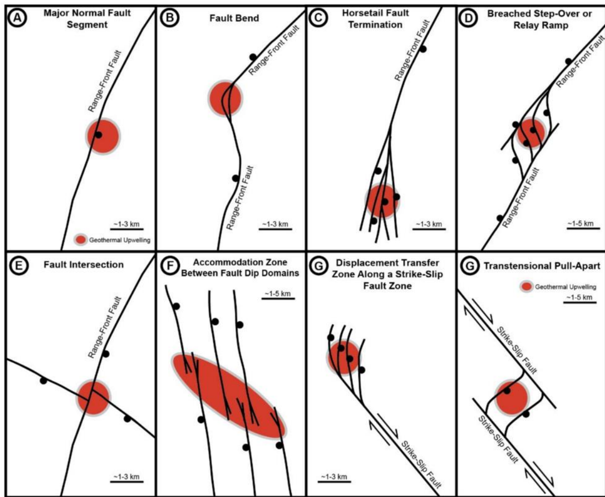
Figure A.32. Favourable structural settings for hydrothermal systems in Nevada. The highest percentage of geothermal systems in Nevada occur on fault terminations (C), fault step-overs (D), and fault intersections (E). Source: Faults and Hinz (2015)
