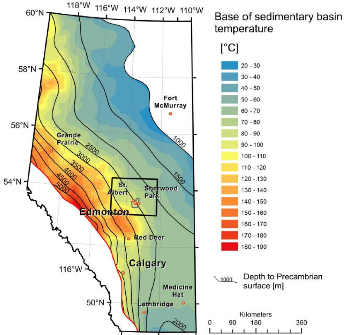
Figure 1.4. Map of temperatures at the basement unconformity of the Western Canada Sedimentary Basin. Temperatures increase from northeast to southwest as the basement unconformity is more deeply buried. Temperatures exceed 180°C near Hinton, AB. Source: (Hofmann et al., 2014)
