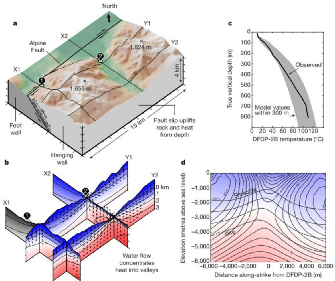
Figure A.60. a) Location map of DFDP-1 and DFDP-2 boreholes along the Alpine Fault near Whataroa. b) Temperature contours and fluid flow in the vicinity of the boreholes. c) temperature profile at DFDP-2, indicating a thermal gradient of \sim 130^{\circ}\text{C}/\text{km} . d) Fluid pressure and temperature on the Alpine Fault plane. (Sutherland et al., 2017).
