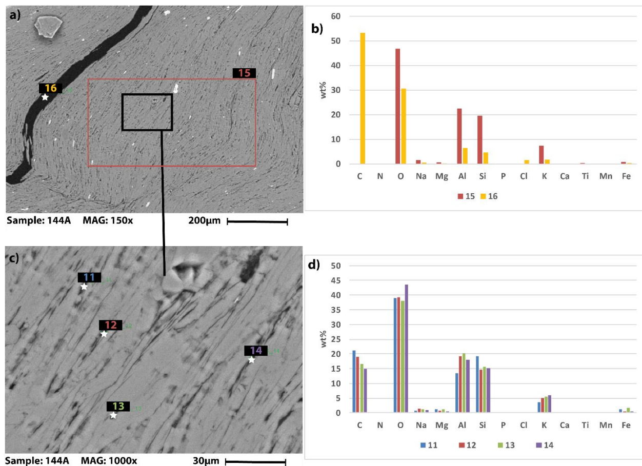
Figure 3.21. SEM images and elemental spectra of sample 144. a) and b) SEM image and EDS data for a 1.5 \times 10^5 \mu\text{m}^2 area (15) and a 50-μm-wide fracture (16). Fracture has 53 wt% carbon, but a trace amount of chlorine indicates possible epoxy contamination. Large rectangular area has no detectable carbon. c) and d) show higher magnification image and EDS data for the area within black box in (a); dark regions on muscovite grain boundaries (points 11-14) are carbon rich (15-21 wt%) and do not contain chlorine.
