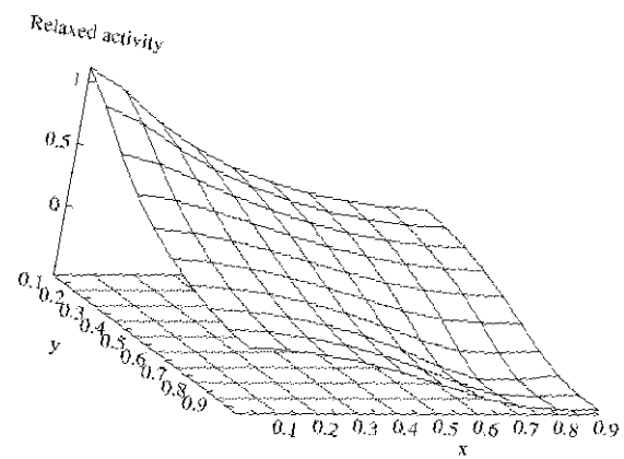
Figure 3: Relaxed neural activity field
