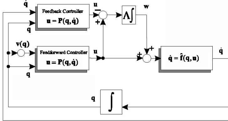
Fig. 1. SDS Control by doubling the role of the inverse dynamics controller
