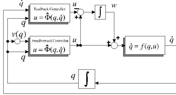
Figure 2: Doubling the role of the inverse-dynamics controller
