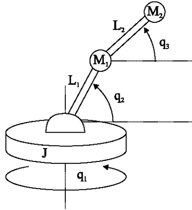
Figure 6: Idealized 3-joint robotic manipulator
