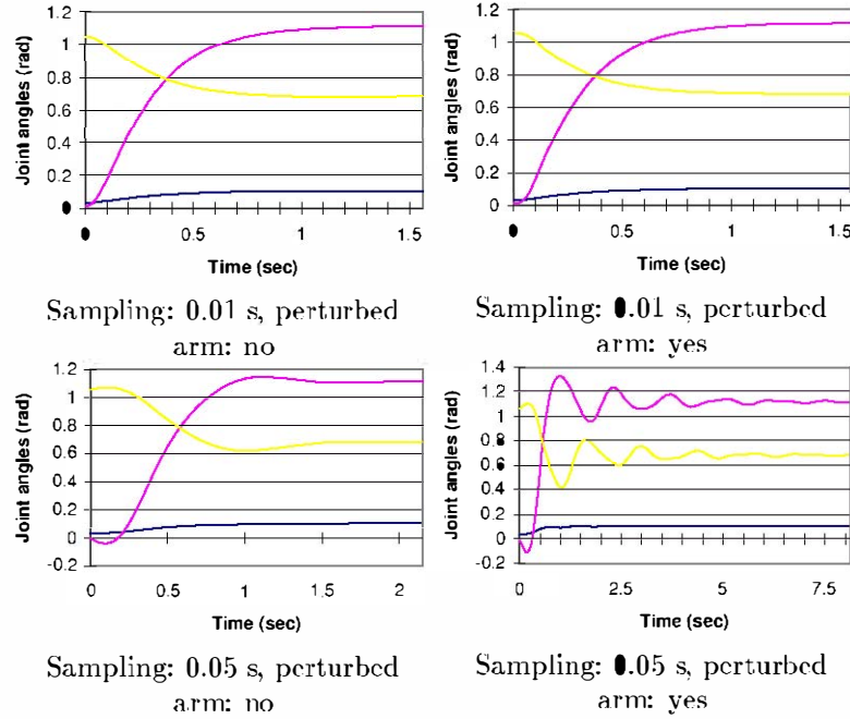
Figure 7: Control of a robotic manipulator using the SDS scheme
