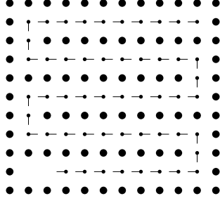
Figure 1: The intersection of two optimal policies for tasks with neighboring goals. The figure shows a macro in a specific environment. The big dots denote walls, small dots denote states in the open space, and the thin sticks starting at a small dot give the direction of the action chosen by the macro at the corresponding state. States without sticks are outside of the domain of the macro. The intersection of the policies defined for the two tasks defined by goal-states placed in the lower left corner are shown in the figure as a macro. .
