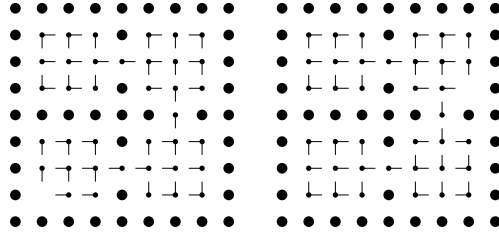
Figure 2: An example environment. A 4-room environment, used in the computer experiments is shown with the solution of two distinct tasks. Note that the optimal solutions are shown as multi-policies, i.e., all the optimal actions are shown for all the states. .
