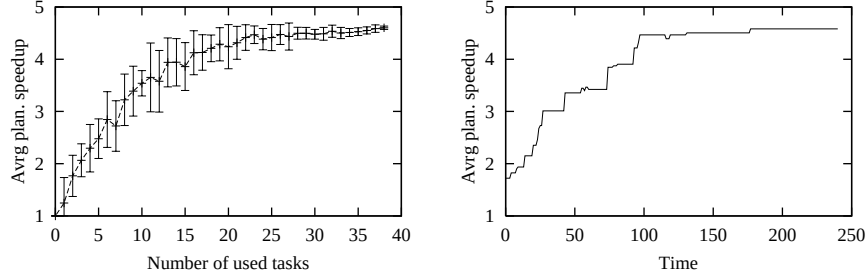
Figure 4: Measures of the planning speed-up In the left figure, the planning speed-up rate is shown as a function of the number of random tasks inputted to the algorithm. In the right figure the planning speed-up rate is shown as a function of time for the on-line learning case when in each time step a random task is added to the list of known tasks. .
