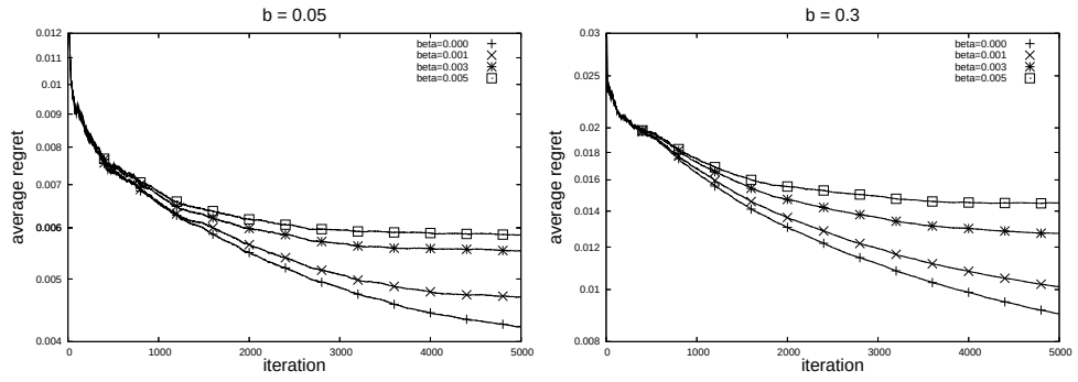
Fig. 3. Regret curves on two instances of the dynamic pricing problem for various values of \beta .
