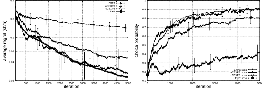
Fig. 8. Learning curves of the four algorithms. Left graph: regret, right graph: probability of choosing the best opponent model ( spsa ). Each data point is averaged over 100 runs.
