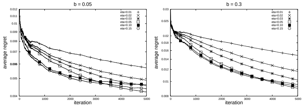
Fig. 2. Regret curves on two instances of the dynamic pricing problem for various values of \eta .
