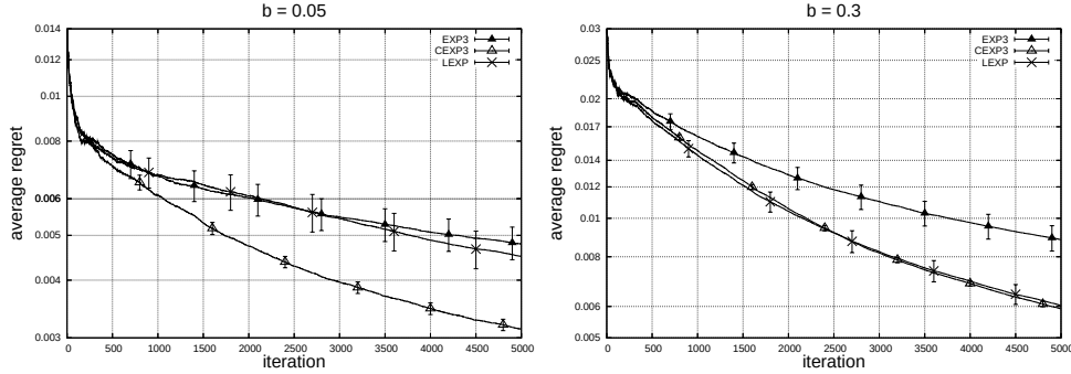
Fig. 5. Regret curves on two instances of the dynamic pricing problem. The 95% confidence intervals are also shown in the figures.
