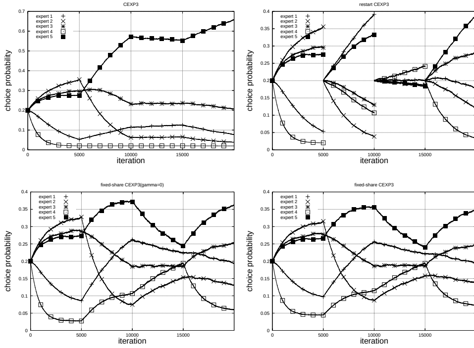
Fig. 7. Choice probabilities for the CExp3 algorithms on the non-stationary dynamic pricing problem.
