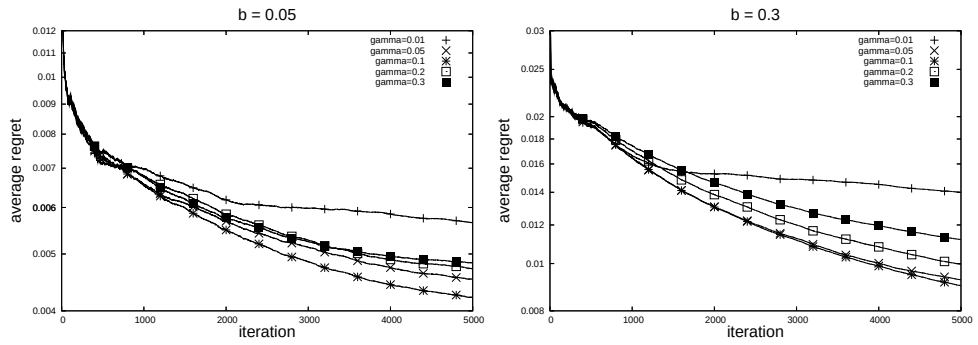
Fig. 4. Regret curves on two instances of the dynamic pricing problem for various values of \gamma .
