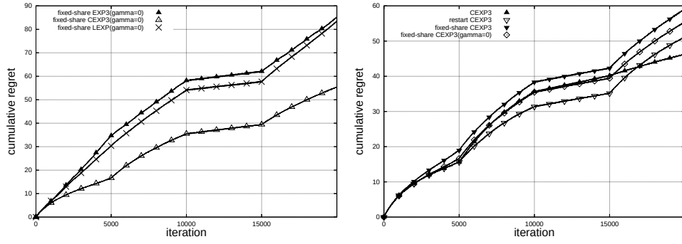
Fig. 6. Cumulative regret for the non-stationary dynamic pricing problem.
