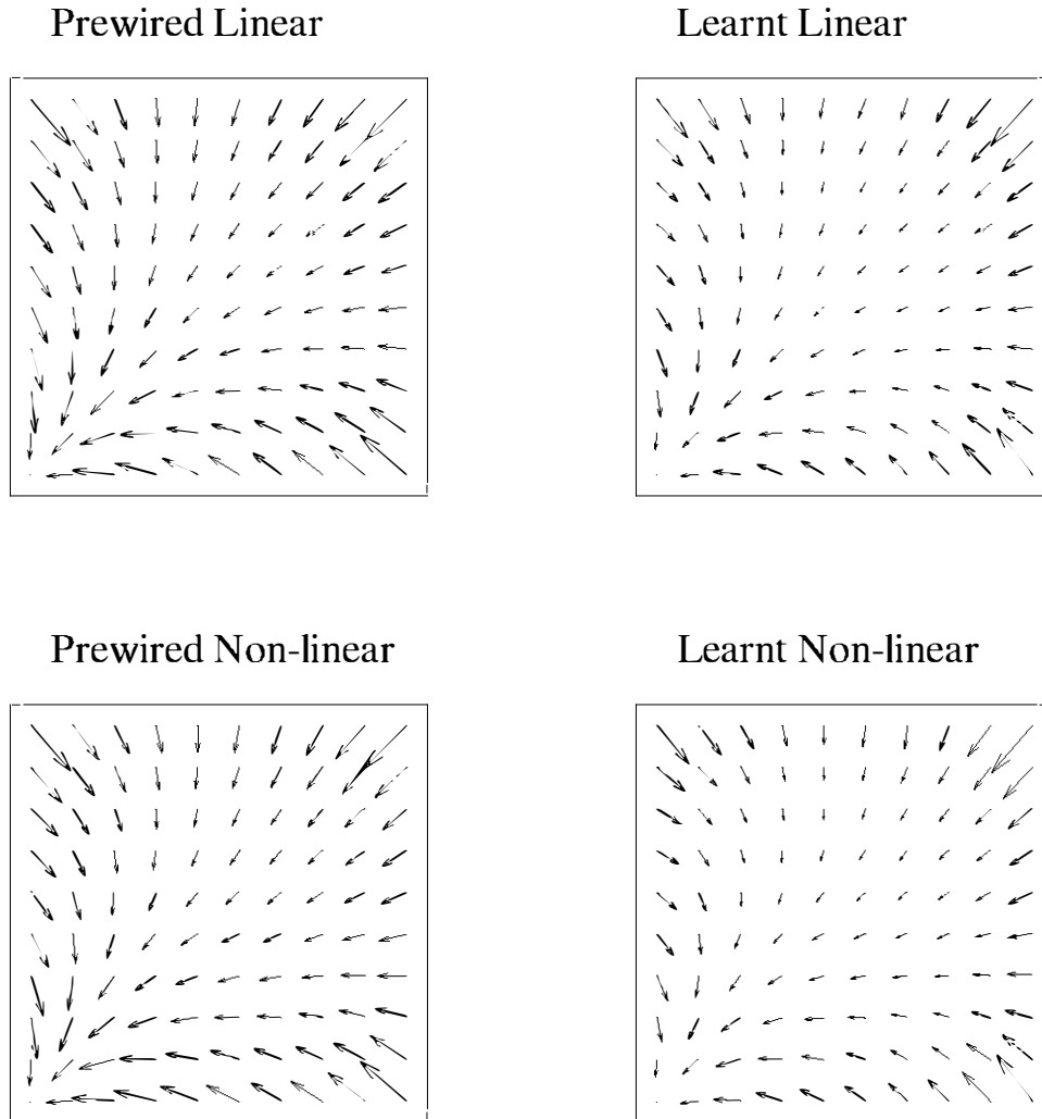
Figure 4: Speed vector fields
