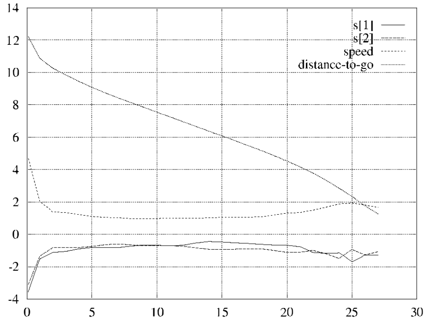
Figure 5: Distance-to-go and components of the speed-vector vs. time
