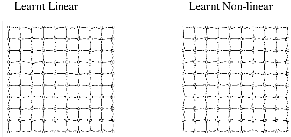
Figure 7: Learnt control command vectors for linear and non-linear plants.
