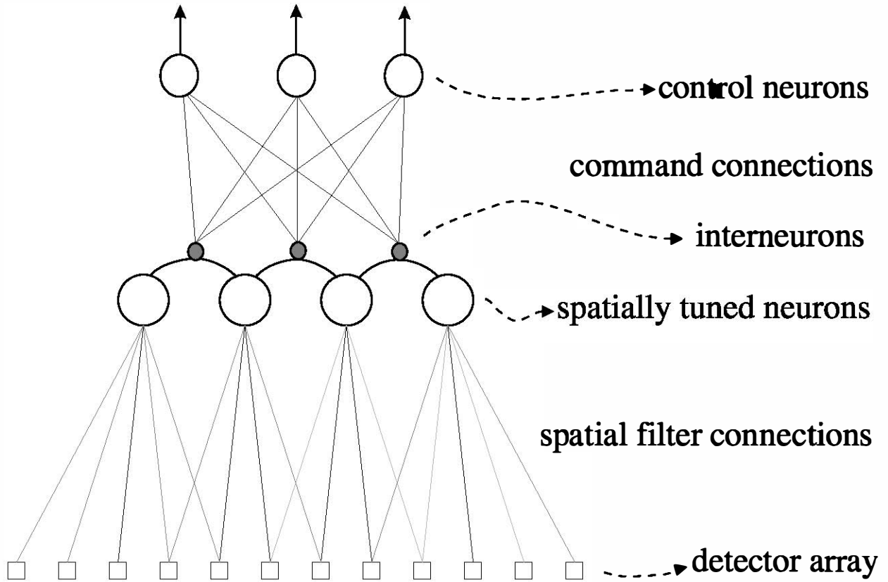
Figure 1: The architecture of the network.
