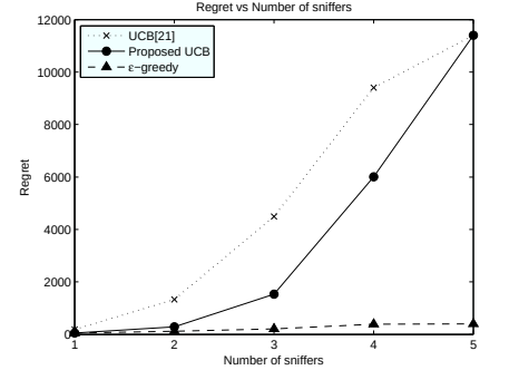
(c) Regret vs. sniffers K = 5, t = 5000
