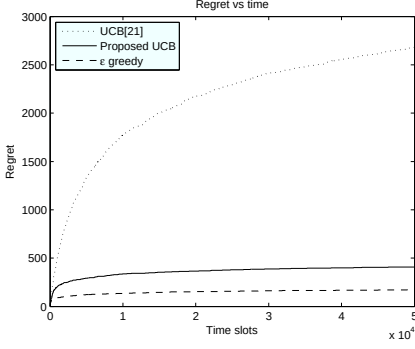
(a) Regret vs. time p = 2, K = 5
