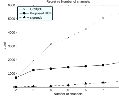
(b) Regret vs. # of chan. p = 3, t = 5000
