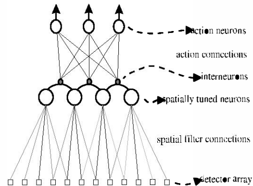
Figure 4: Hierarchy of self-organizing neurocontrol
