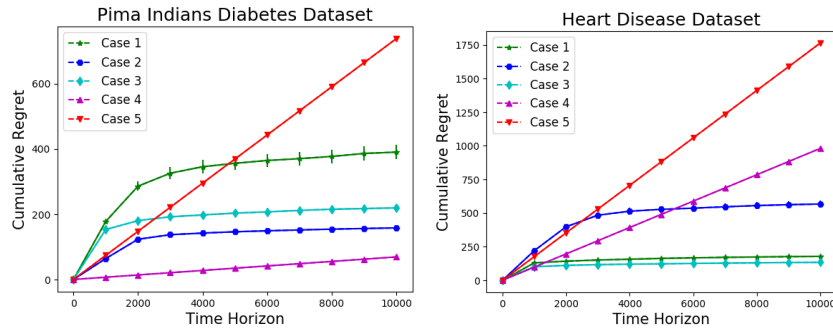
Figure 7: Cumulative regret of \text{USS-UCB}(\alpha = 0.51) for different problem instances of the Real Datasets where last two classifier are interchanged in the sequence while keeping the cost same as given in the Table 2. Note that, i^* = K for Case 4 and WD automatically holds but after interchanging last two classifiers, WD does not hold for Case 4.
