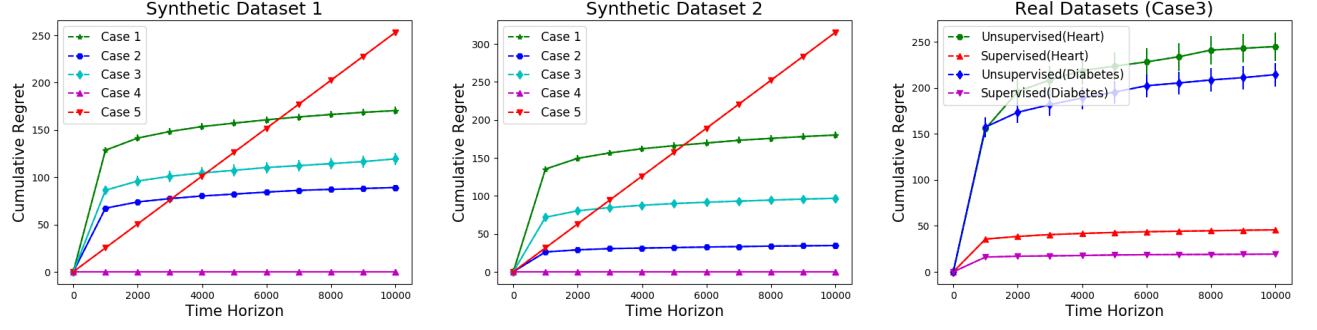
Figure 8: Cumulative regret of \text{USS-UCB}(\alpha = 0.51) for different problem instances of the Synthetic Dataset 1 and 2. Rightmost figure: Comparison between unsupervised and supervised setting for Case 3 of real datasets.
