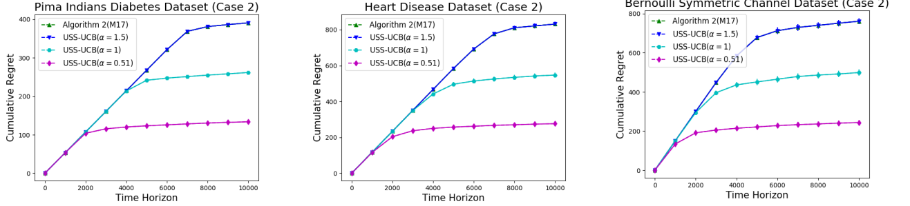
Figure 5: Comparison between Heuristic Algorithm 2 proposed in [1] and USS-UCB with parameter \alpha = \{1.5, 1, 0.51\} for Case 2 of the real datasets and synthetic BSC dataset.
