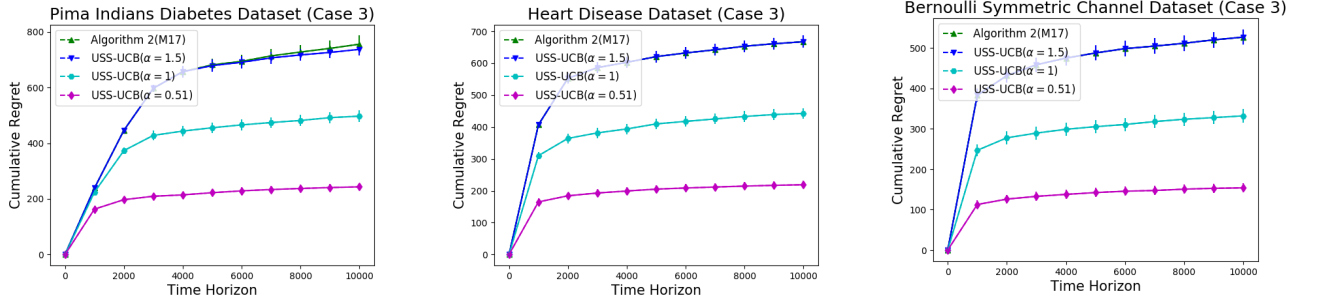
Figure 6: Comparison between Heuristic Algorithm 2 proposed in [1] and USS-UCB with parameter \alpha = \{1.5, 1, 0.51\} for Case 3 of the real datasets and synthetic BSC dataset.
