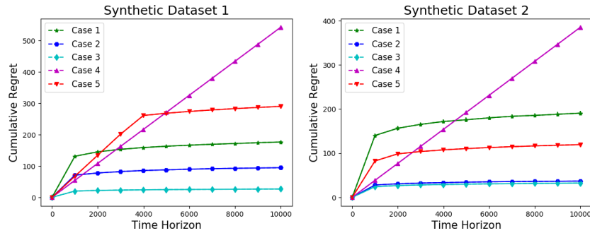
Figure 11: Cumulative regret of \text{USS-UCB}(\alpha = 0.51) for different problem instances of the Synthetic Dataset 1 and 2 with last two classifier are interchanged in the sequence while keeping the cost same as given in the Table 3 and 4. Note that, i^* = K for Case 4 and WD automatically holds but after interchanging last two classifiers, WD does not hold for Case 4 whereas holds for Case 5.
