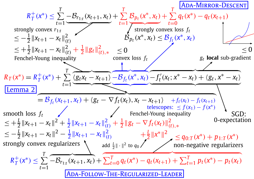
Fig. 2. A summary of the proof techniques that incorporate each of the assumptions into regret bounds; see Corollaries 19–21 and Table 2. The identity in the middle is from Lemma 2, whereas the top and bottom bounds on R_T^+ are due to Theorem 3. Each arrow shows the transformation of one of the terms, using the stated assumption or technique. The matching terms cancel, and the terms shown in red appear in the final bounds. (For interpretation of the colors in the figures, the reader is referred to the web version of this article.)
