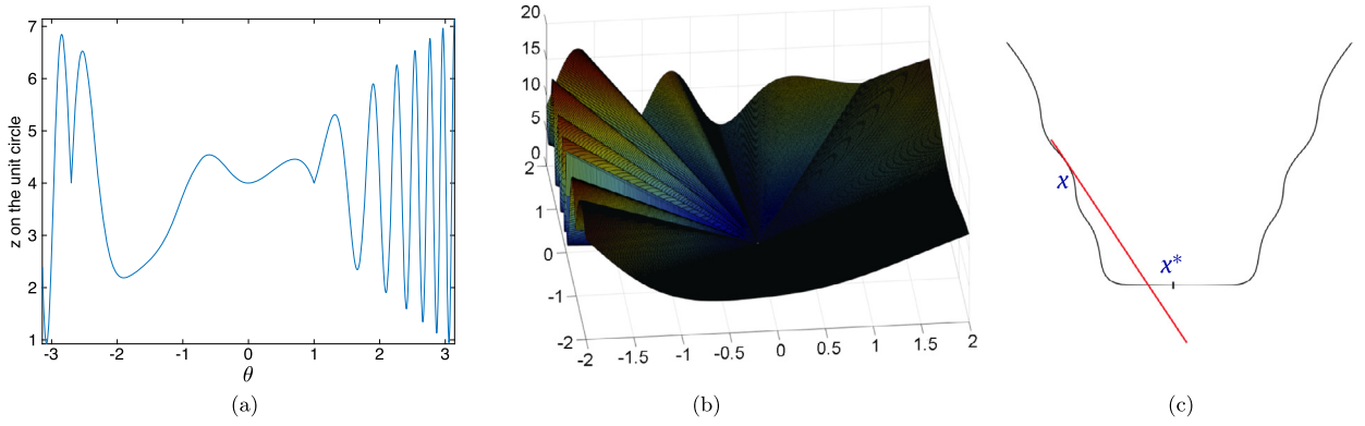
Fig. 3. Star-convex functions: (a) z defined on the unit circle and (b) its star-convex extension to two dimensions. (c) The linear approximation of a star-convex function fitted at any point is a lower bound at the minimum.
