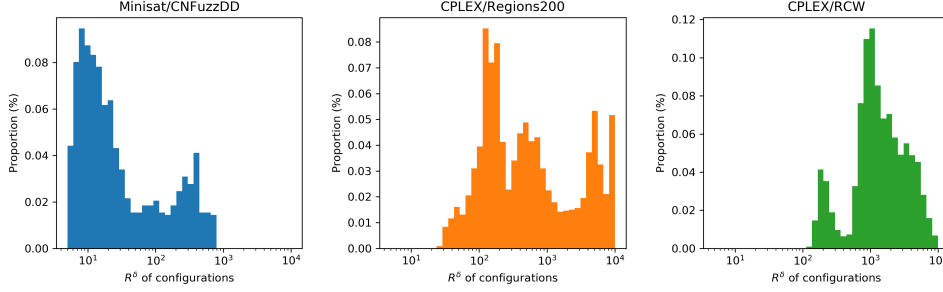
Figure 2: Distribution of \delta -capped mean runtime of the sampled configurations, with \delta = 0.1 . For Minisat/CNFuzzDD, many configurations are close to the optimal one, whereas for CPLEX/Regions200 and CPLEX/RCW, many configurations are significantly worse than the optimal one. Consequently, PRECHECK is able to discard more configurations in the latter two scenarios.
