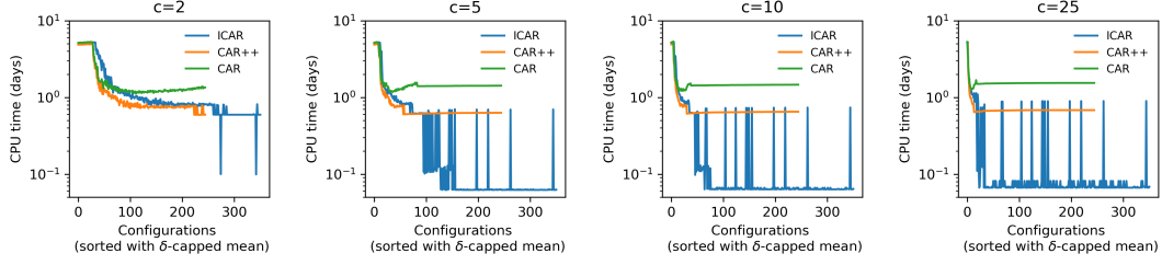
Figure 3: Synthetic experiments: As the proportion of configurations that are far from the optimal gets larger (i.e., as c gets larger), the CPU runtime of CAR was more dominated by the work spent on bad configurations, while ICAR was able to drop more bad configurations with its PRECHECK mechanism. Note the log scale on the y -axis.
