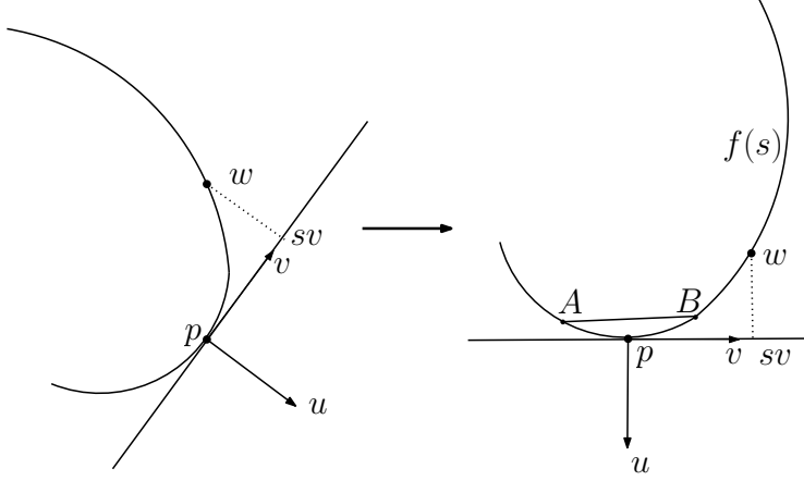
Figure 3: The local coordinate system of p .
