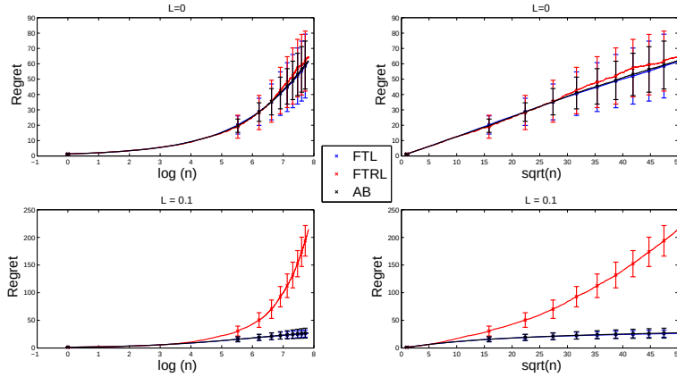
Figure 4: Regret of FTL, FTRL and AB(FTL,FTRL) against time for stochastic data.
