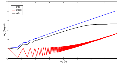
Figure 6: Experimental results for worst-case data.
