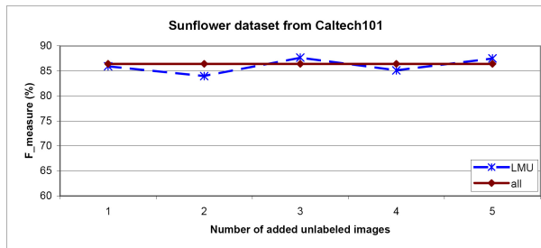
Figure 7. LMU of sunflower category in Caltech101 dataset
