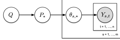
Figure 1. Graphical model of our bandit environment.
