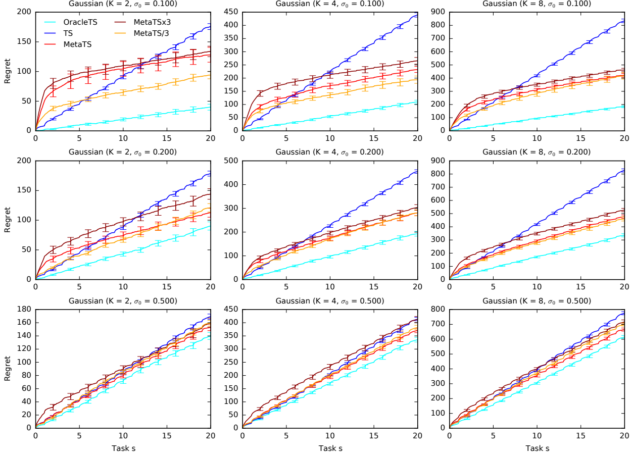
Figure 3. MetaTS in K -armed Gaussian bandits with a varying number of arms K and instance prior width \sigma_0 .
