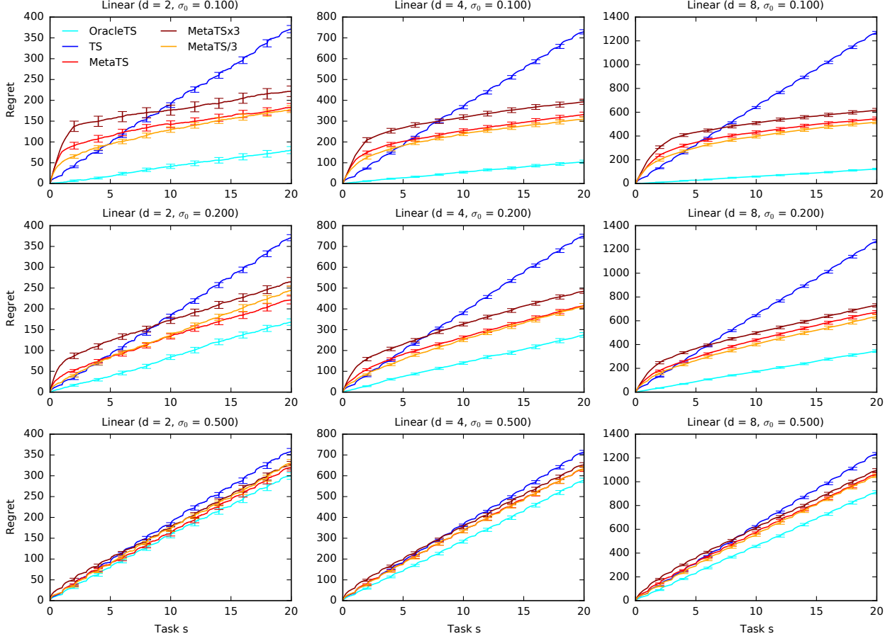
Figure 4. MetaTS in d -dimensional linear bandits with a varying dimensionality d and instance prior width \sigma_0 .
