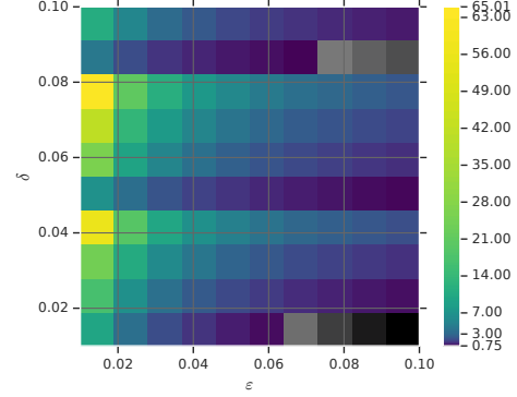
Figure 2: The ratio of the total runtime of LEAPSANDBOUNDS and CAPSANDRUNS for various values of \varepsilon and \delta . Ratios greater than 1 mean CAPSANDRUNS is faster; values lower than 1 are shown in greyscale.
