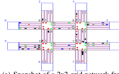
(a) Snapshot of a 2x2-grid network from GLD simulator. The figure shows eight edge nodes that generate traffic, four traffic lights and four-laned roads carrying cars.
