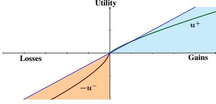
Figure 2. An example of a utility function. A reference point on the x axis serves as the point of separating gains and losses. For losses, the disutility -u^- is typically convex, for gains, the utility u^+ is typically concave; they are always non-decreasing and both of them take on the value of zero at the reference point.
