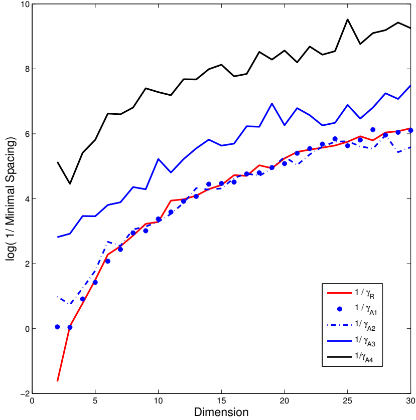
Figure 3. The values of 1/\gamma for matrices with different coherences
