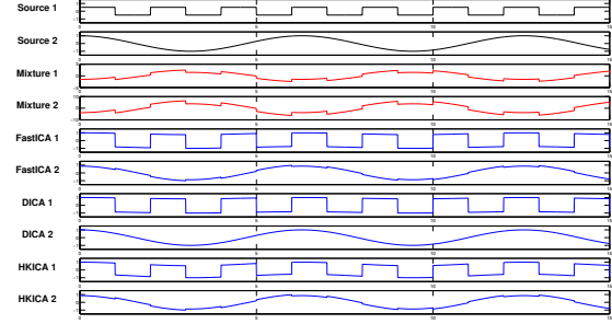
Figure 1. Example of ICA for deterministic sources: The first two rows show the source signals s_1(t) = 0.5 - \lfloor t - 2\lfloor t/2 \rfloor \rfloor , s_2 = \cos(t) , the next two rows present the observations with mixing matrix A = \begin{pmatrix} 1 & -2 \\ 2.6 & -5.1 \end{pmatrix} . The reconstructed (and rescaled) signals are shown for FastICA, HKICA, and DICA after sampling As(t) at 10000 uniformly spaced points in the interval [0, 15] .
