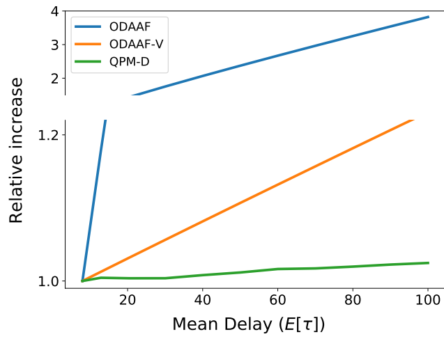
Figure 5: The relative increase in regret at time T = 250000 for increasing mean delay when the delay is \mathcal{N}_+ with variance 100.
