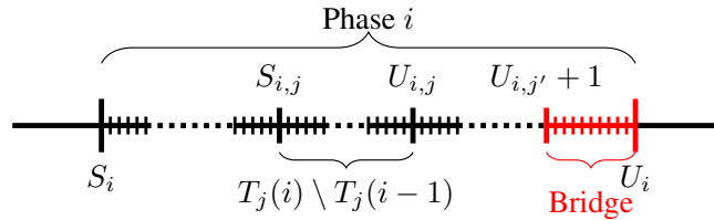
Figure 4: An example of phase i of our algorithm.
