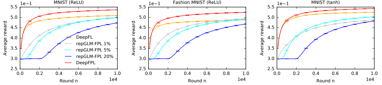
Figure 2: Evaluation of DeepFPL and DeepTSL on contextual bandit problems in Section 5.3.
