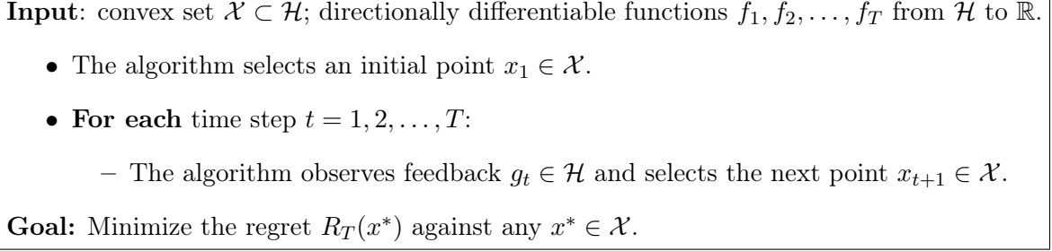
Figure 1: Iterative optimization.
