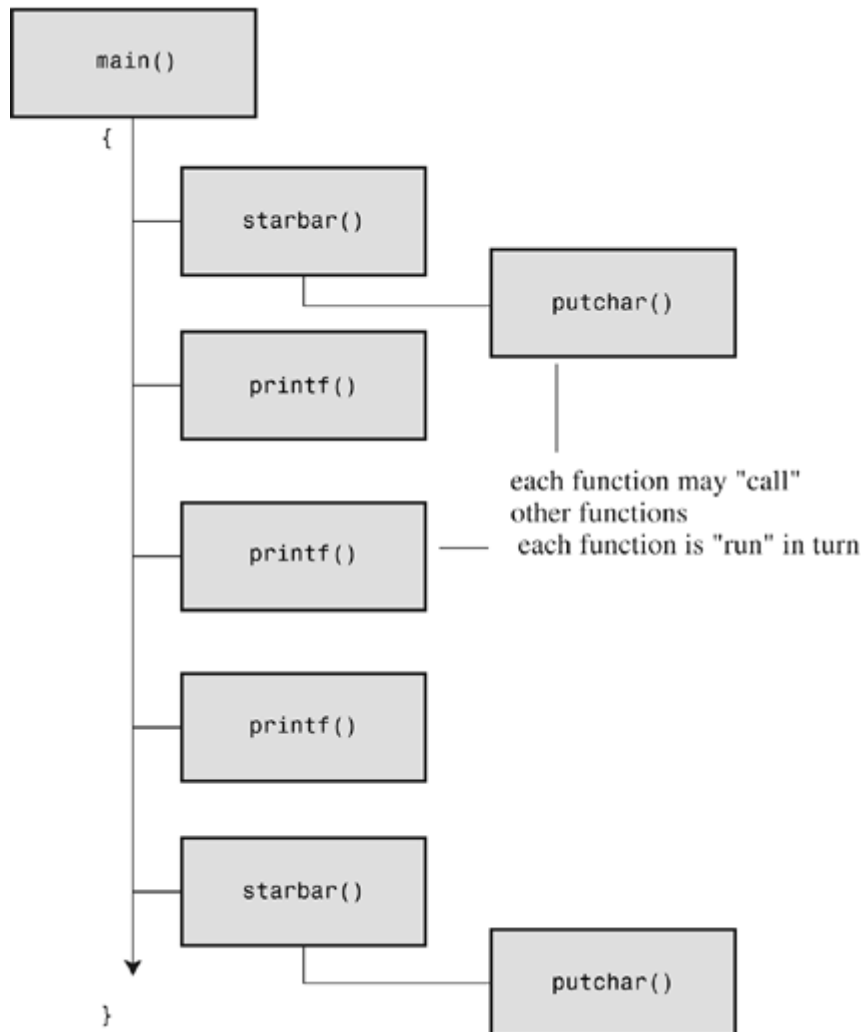
Figure 9.1. Control flow for lethead1.c ( Listing 9.1 ).
