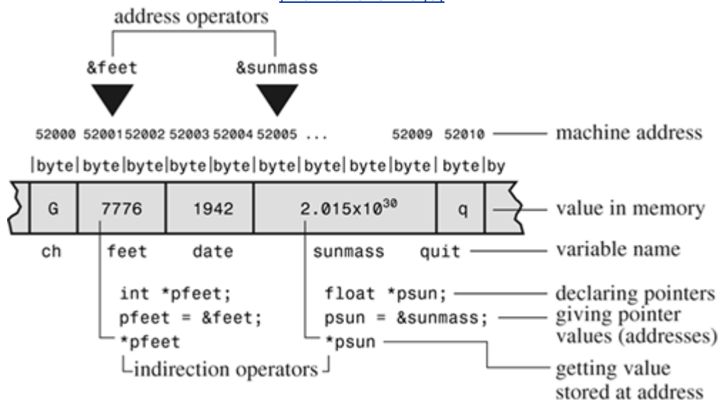
Figure 9.5. Declaring and using pointers.
