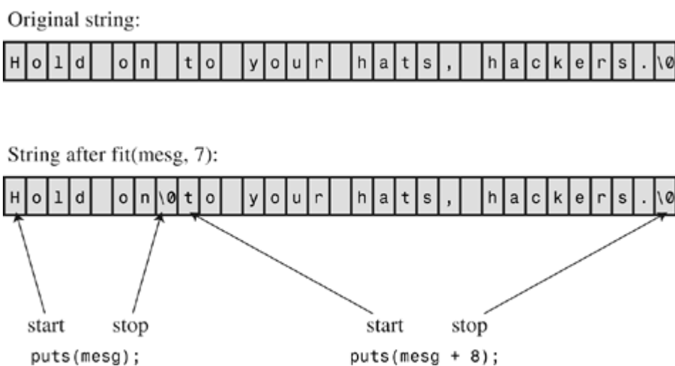
Figure 11.4. The puts() function and the null character.
