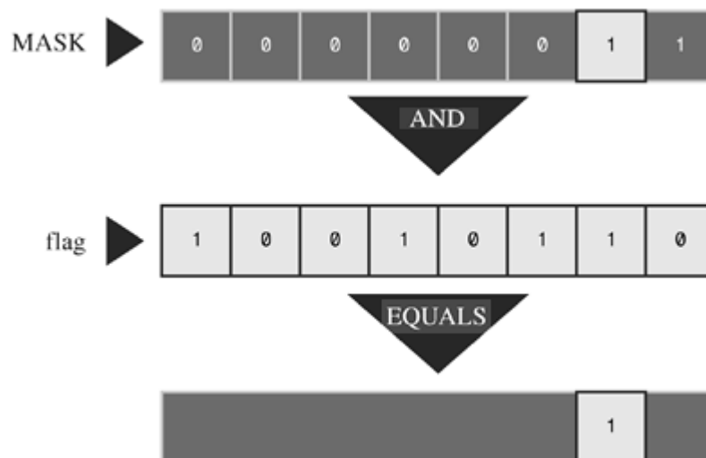
Figure 15.2. A mask.
