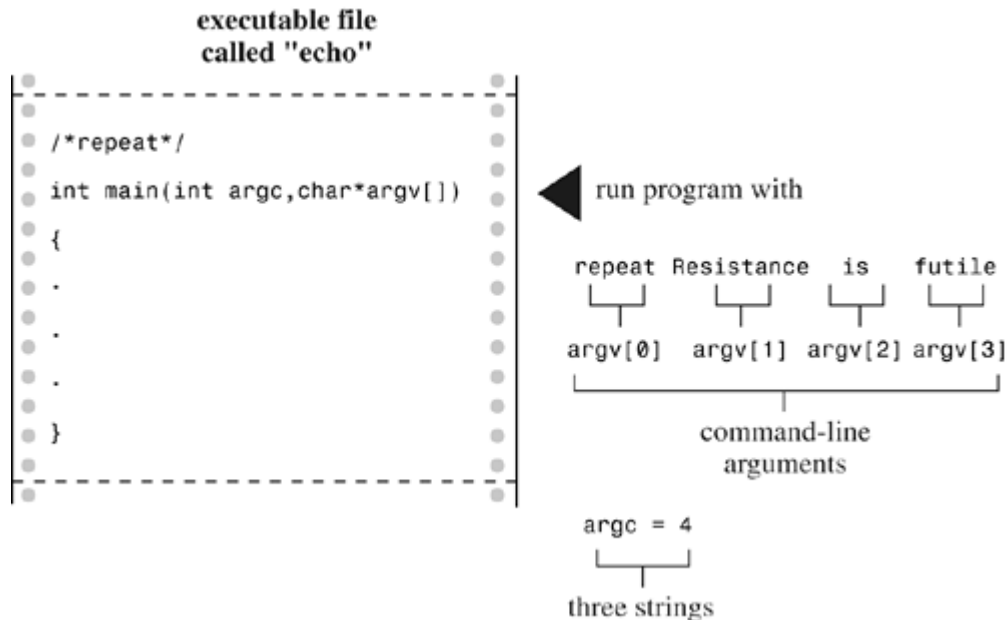
Figure 11.7. Command-line arguments.
