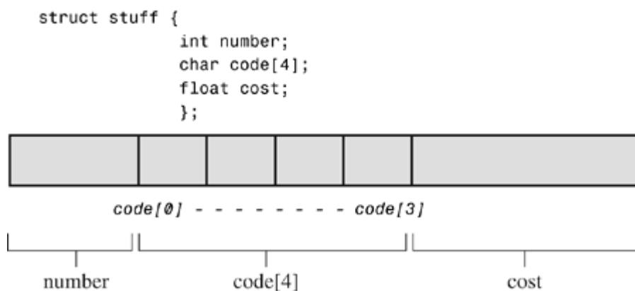
Figure 14.1. Memory allocation for a structure.
