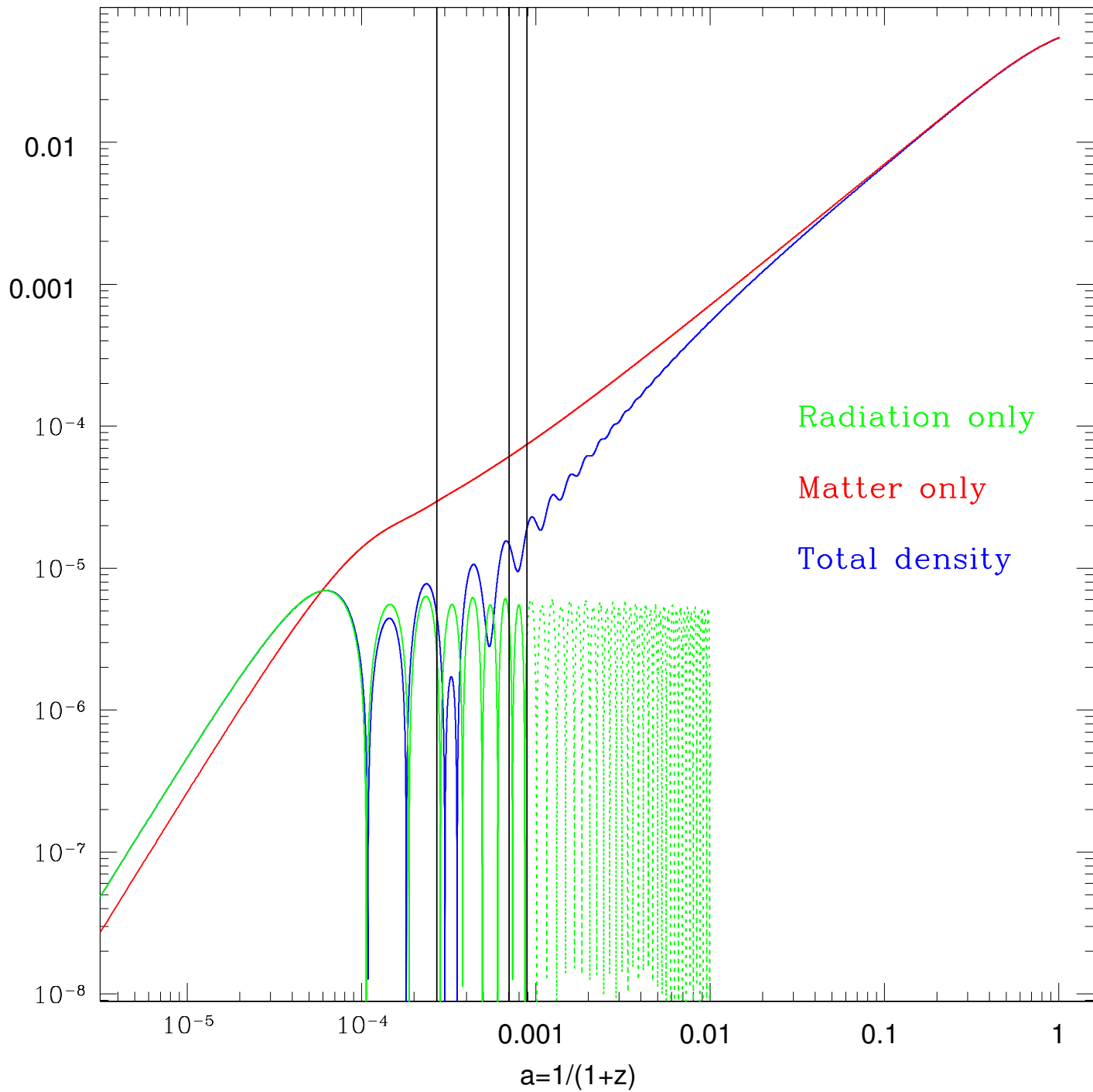
Evolution of fluctuations at fixed k
