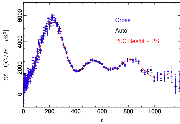
Figure D.9. The power spectrum from the Planck 70 GHz channel, before removal of unresolved sources. Both the auto-spectrum from the 70 GHz maps, and the weighted cross spectra from maps of the three 70 GHz horn pairs are shown. The best-fitting cosmological model from CamSpec, shown for comparison with the best-fitting source power added, gives a good fit to the data.
