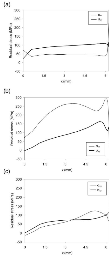
Fig. 9. Residual stress distribution in the interlayer near the interface with the ceramic: (a) joint with 0.3 mm Ni single interlayer; (b) joint M-1: \text{Si}_3\text{N}_4/0.3 \text{ mm W}/0.3 \text{ mm Ni}/\text{Inconel 718} ; (c) joint M-2: \text{Si}_3\text{N}_4/0.3 \text{ mm Ni}/0.3 \text{ mm W}/\text{Inconel 718} .
