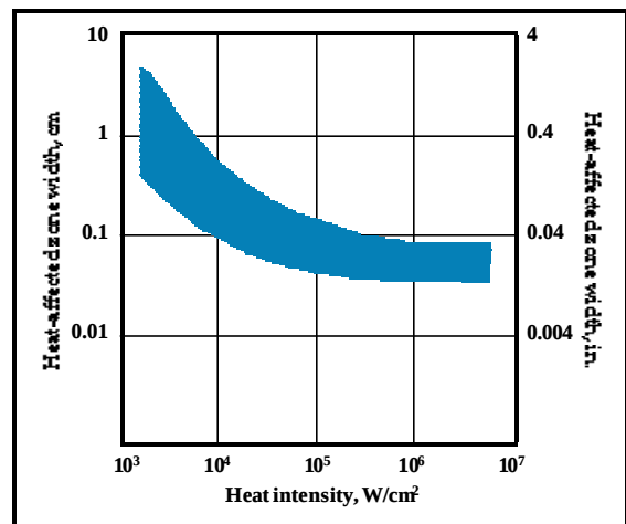
Fig. 4 — Size of the HAZ as a function of intensity of the heat source.
