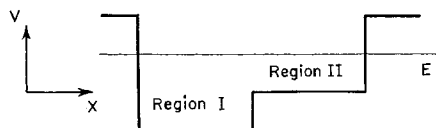
FIG. 1. Potential plot used to analyze peak heights of wave function as a function of well depth.
