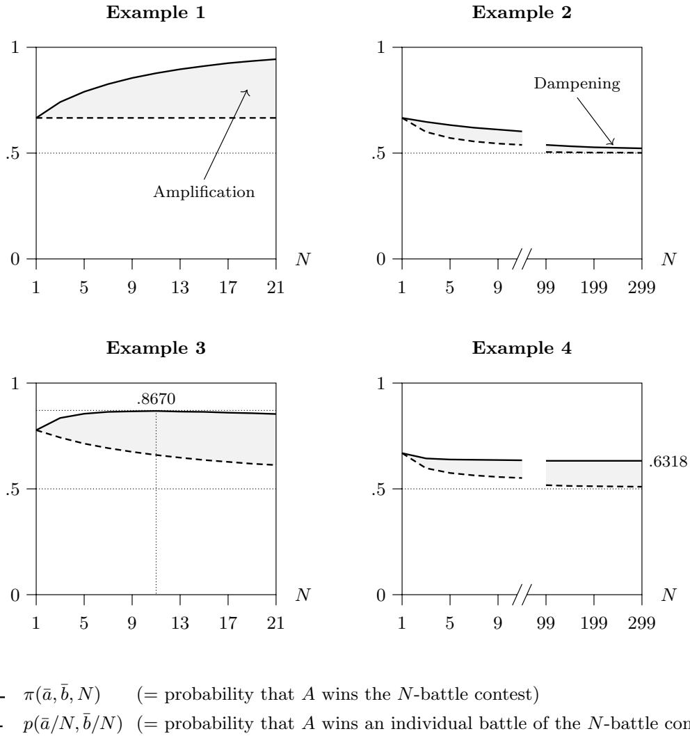
Figure 1: Win probability as a function of contest length.
