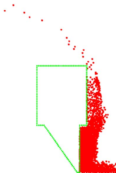
Fig. 14. Simulation of 2000 particles scraped from the bottom surface at 7 \times 10^{-1} s after starting up.
