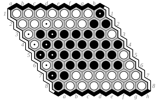
Fig. 8. 1-move 8×8 Hex openings (dotted). Cell color shows winner if black opens there.
