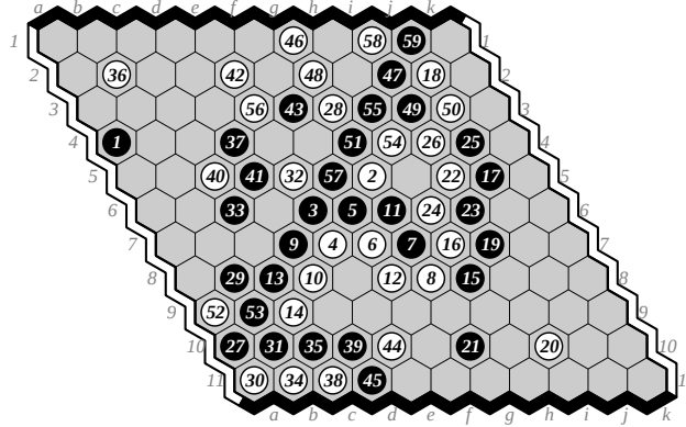
Fig. 7. An 8min/move DeepHex (Black) win over MoHex. With 26.i4 MoHex has winrate .51 and PV a10 g3 g4 f4 a8 c7 d5 d4 a6 a5 b5 c5 e4 f2 i3 i2 j3 a11 f5 h3 h4 h9 g9 d10 e9 e10. With 27.a10 DeepHex finds a loss – unproven due to pruning – with PV f4 h4 h5 g4 f5 b8 d5 a6 a5 b5 a11 b10 b11 c10 c11 d10 c3 b4 b2 i3 j3 e4 e5 c2 b3. But MoHex blunders with 28.g3 : winrate is .52 but DeepHex sees a huge advantage. With 33.c6 DeepHex finds a proven win, PV d1 d4 e3 d2 e10 b11 c2 d3 e1 e2 f1 f2 g1 g2 h1 h2 i1 b2 b3 a3 b4 a5 b6 b5 c5 c4 d5 f5. By 38.c11 MoHex finds a proven loss.
