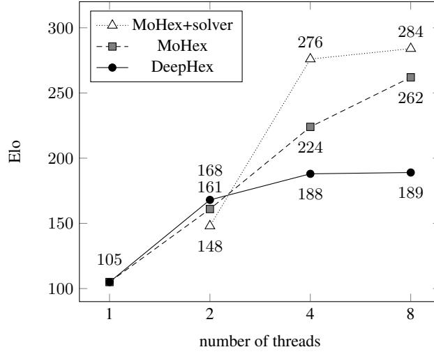
Fig. 8. Tournament results. Each point has error within 14 Elo, with 80% confidence. Reference player is 1-thread Wolfe, BayesElo score 0.
