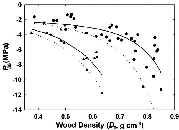
Fig. 7. P_{50} vs wood density for angiosperm (circles) and conifer stems (triangles). Same species as Figs. 6, 8, 10. Drought-resistant xylem showed greater density in both conifers and angiosperms. Conifers achieve a given P_{50} with less biomass (lower density) than angiosperms. Solid curves represent expected trend based on conduit reinforcement against implosion by negative pressure; the r^2 of the curve fit was 0.62 in angiosperms and 0.73 in conifers. Dashed curves suggest a lower boundary line set by a conduit implosion limit (from Hacke et al. 2001b).
