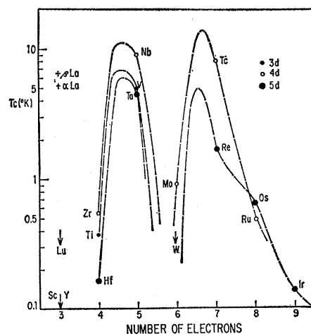
Fig. 1. Variation in superconductivity of the transition elements in the periodic system.
