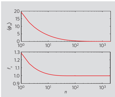
Figure 1 | Species abundance* . Top, plot of \langle \phi_n \rangle , the average number of species with abundance n , against n for the model described in ref. 2, using the biodiversity parameter \Theta = 50 , the immigration parameter m = 0.1 and a population of 20,000. Bottom, plot of \hat{r}_n , the density-dependent birth rate–death rate ratio, against n , deduced from the RSA data.
