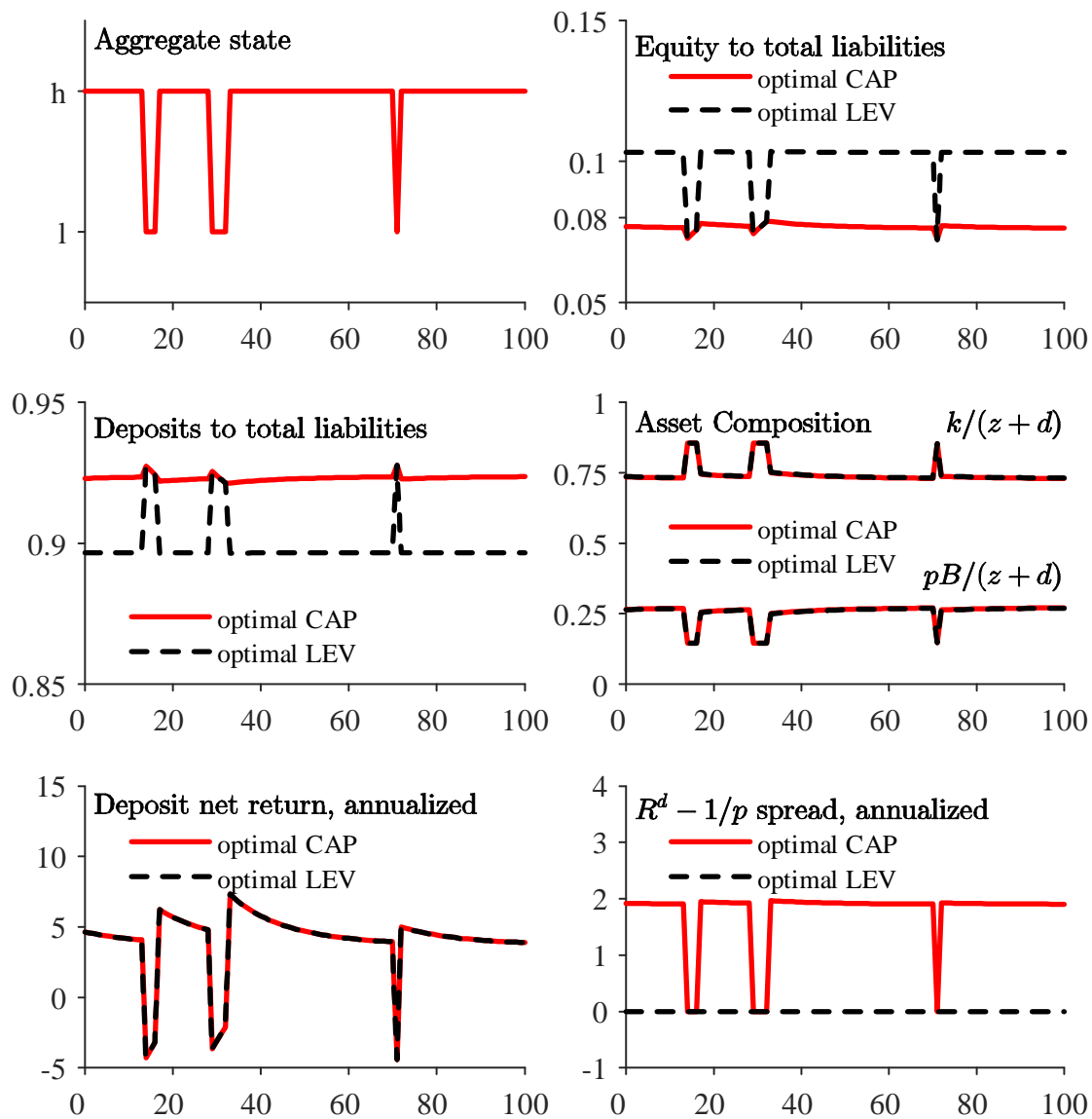
Figure 3: OPTIMAL CAP AND OPTIMAL LEV ECONOMIES: BALANCE SHEET COMPOSITION AND ASSET RETURNS
