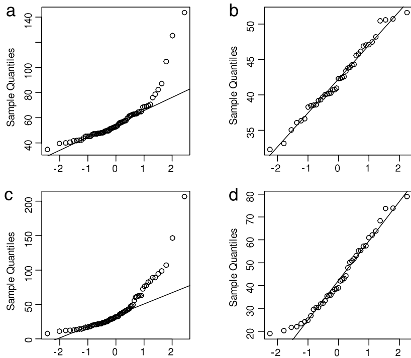
Fig. 5. Top: qq-plots of \{t_j = \Delta(\mathbf{S}_j, \hat{\Sigma}_{TMIL})\} for the (a) untrimmed and (b) trimmed samples of EEG spectral matrices. Bottom: qq-plots of \{d_j = \Delta(\mathbf{S}_j, \hat{\Sigma}_{MILD})\} for the (c) untrimmed and (d) trimmed samples.
