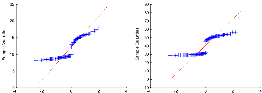
Fig. 4. Representative qq-plots of (a) \{t_j\}_{j=1}^n , and (b) \{d_j\}_{j=1}^n ; (\varepsilon_1, \varepsilon_2) = (0.5, 0.2) and f_{small} = 0.5 .
