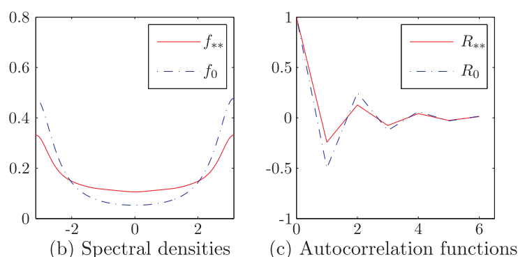
Figure 2. (a) Sampling designs for an approximate AR(1) model; \varepsilon = 0.25 , n = 30 , N = N_0 = 200 . Values of \max_{\mathcal{F}_\varepsilon} \text{AMSPE} are shown for \varepsilon = 0 (left) and \varepsilon = 0.25 (right). (b) Base spectral density f_0 and least favourable spectrum f_{**} ; (c) corresponding autocorrelation functions.
