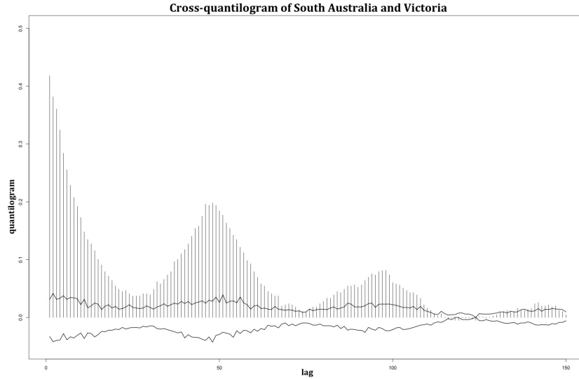
Figure 5.3: A: Cross-quantilograms for SA conditioning on VIC (2009 – 2014).
