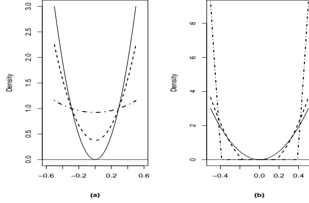
Figure 2.1: Forms of possible I-optimal densities for different values of b . Plot (a) presents three cases of robust densities m_0(x) in which \nu tends to one: b = 0 , \nu = 0.13 (solid line), b = -0.05 , \nu = 0.26 (dashed line), and b = -1 , \nu = 0.85 (dotted-dashed Line); and plot (b) presents three cases of robust densities m_0(x) in which \nu tends to zero: b = 0 , \nu = 0.13 (solid line), b = 0.03 , \nu = 0.083 (dashed line), and b = 0.15 , \nu = 0.0096 (dotted-dashed Line).
