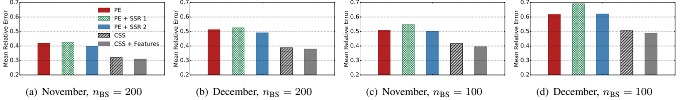
Fig. 2. Comparison of the estimation's Mean Relative Error of different methods when n_{BS} = 200 or n_{BS} = 100 for stress-testing. In each figure, the bars from left to right stands for Patched Estimation, Patched Estimation + SSR 1, Patched Estimation + SSR 2, Constrained Spatial Smoothing, and Constrained Spatial Smoothing + Features respectively.
