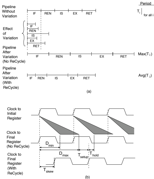
Figure 2: Effect of process variation on pipelines (a) and skewing a clock signal (b).
