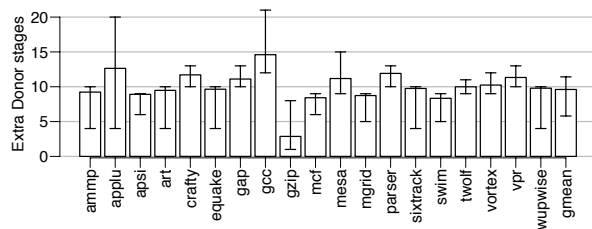
Figure 13: Number of donor stages needed to match the performance of the no-variation pipeline.
