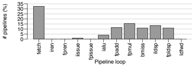
Figure 7: Histogram of critical pipeline loops.
