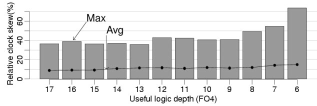
(b) Skew versus logic depth
