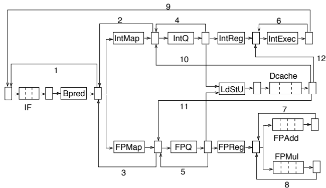
(a) Simplified logical pipeline structure.
