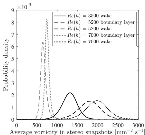
FIGURE 11. Probability density functions of average streamwise vorticity ( \langle\omega_x\rangle ) per unit area of the conditionally sampled vortex cores with Q > 3000 \text{ s}^{-2} in the boundary layer at x = -0.3h and wake at x = 2h for Re(h) = 3500 , 5200, and 7000. A change in vortex strength of nearly an order of magnitude is visible between the boundary layer and wake.
