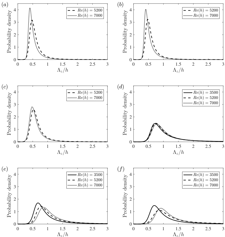
FIGURE 8. Probability density functions of the distance between adjacent low-speed zones ( \Lambda_z ) at Re(h) = 3500, 5200, and 7000 at streamwise locations (a) x = -2h, (b) x = -h, (c) x = 0, (d) x = h, (e) x = 2h, and (f) x = 3h. The peak of each distribution represents the most probable value for \Lambda_z at the corresponding streamwise location and Re.
