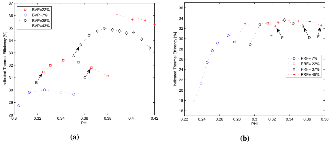
Figure 3: Variation of indicated thermal efficiency versus equivalence ratio at different (a) BVPs and (b) PRFs. (A through F correspond to engine operating points listed in Table 2)
