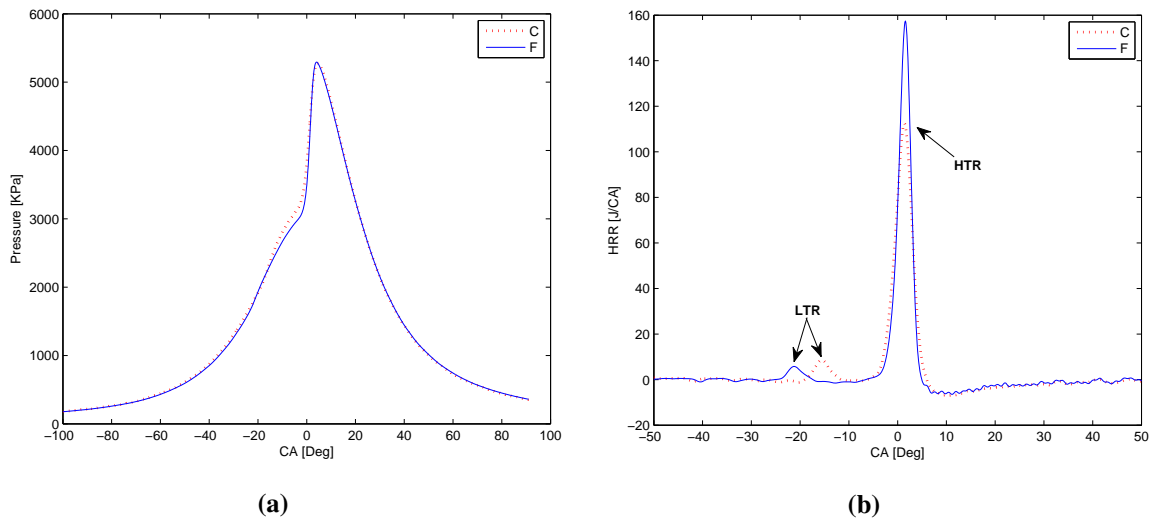
Figure 6: (a) Cylinder pressure versus Crank Angle (b) Heat release Rate versus Crank Angle (C and F refer to engine operating points in Table 2)
