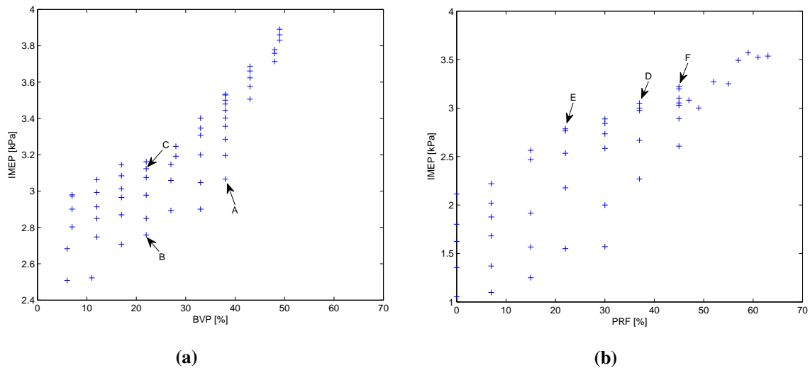
Figure 2: IMEP versus (a) BVP and (b) PRF (A through F correspond to engine operating points listed in Table 2)
