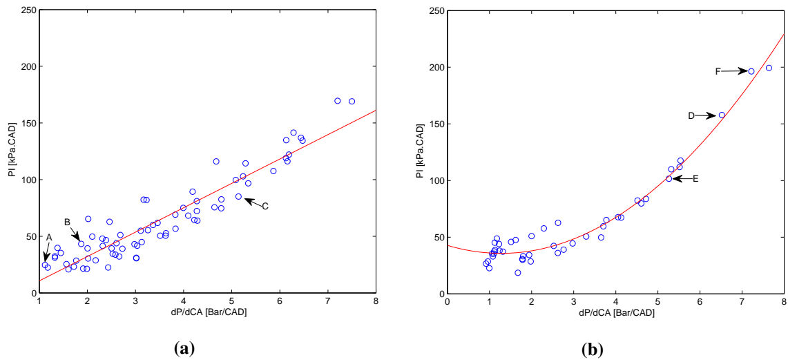
Figure 4: Pressure Intensity (PI) versus maximum rate of pressure rise at different (a) BVPs and (b) PRFs. (A through F correspond to engine operating points listed in Table 2)
