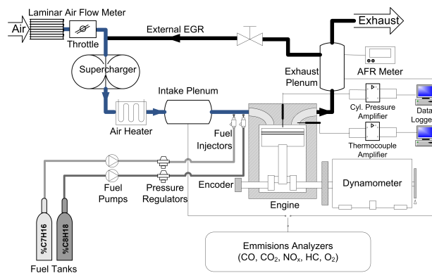
Figure 1: Single cylinder engine testbench schematic
