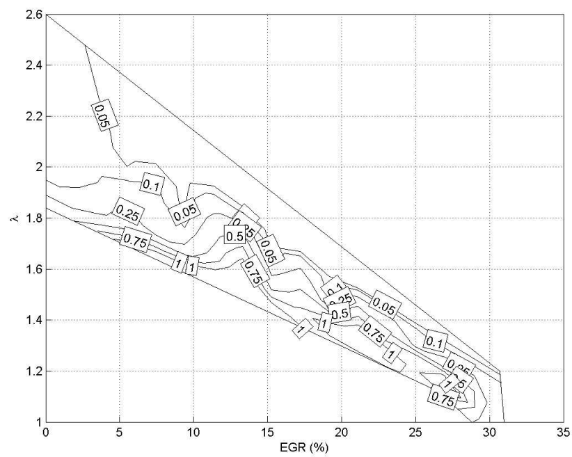
Figure 4.5: Indicated Specific \text{NO}_x in g/kWh for PRF20
