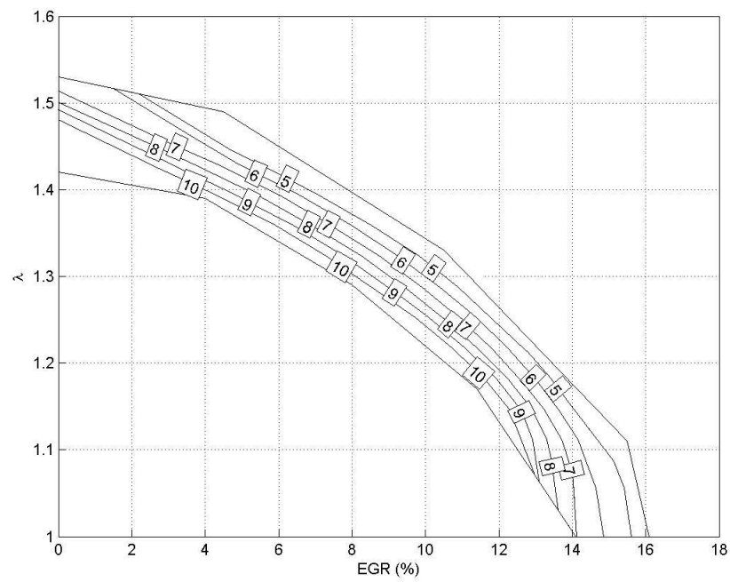
Figure 4.23: Indicated Specific \text{NO}_x in g/kWhr for PRF60
