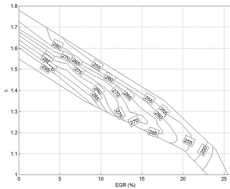
Figure 4.17: ISFC in g/kWhr for PRF40
