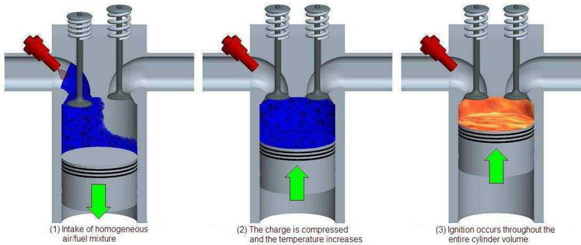
Figure 2.1: HCCI Operation
