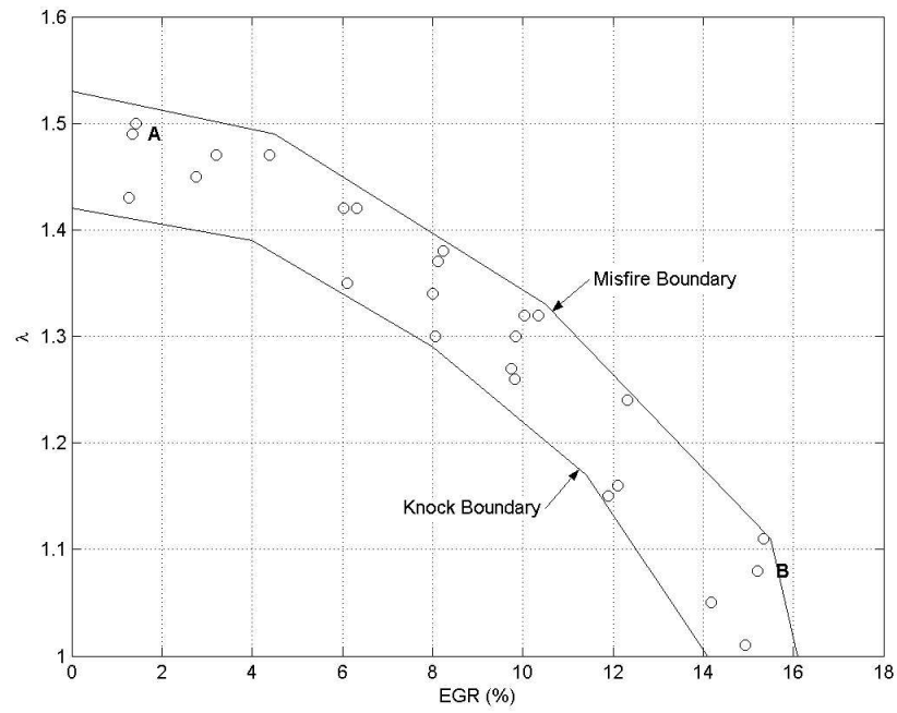
Figure 4.20: HCCI Operating Region for PRF60
