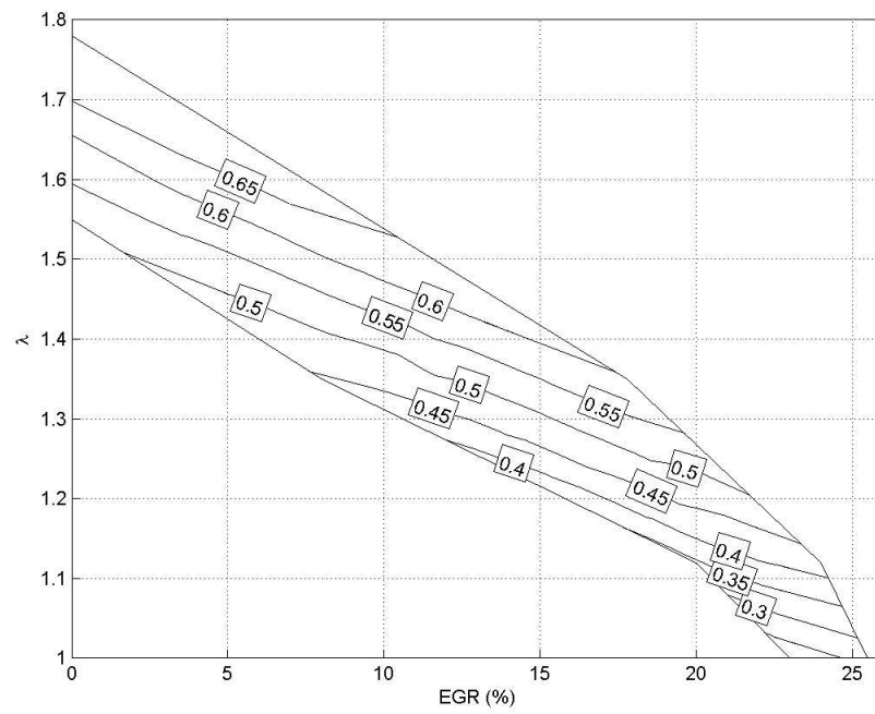
Figure 4.12: Effective Dilution for PRF40
