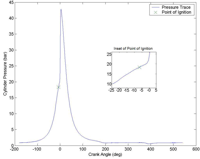
Figure 3.2: Point of Ignition, EGR=1.6%, \lambda=1.81
