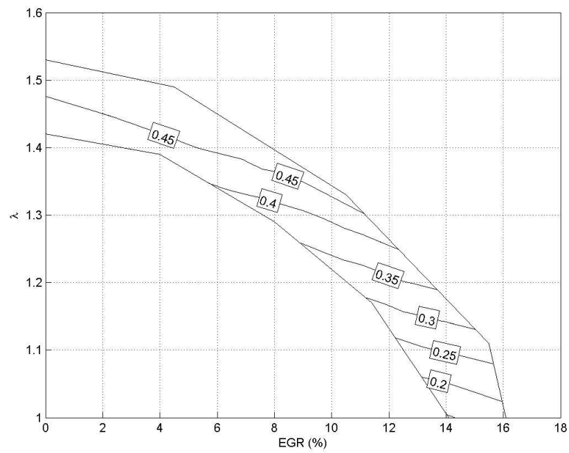
Figure 4.21: Effective Dilution for PRF60
