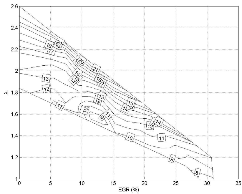
Figure 4.7: Indicated Specific CO in g/kWhr for PRF20
