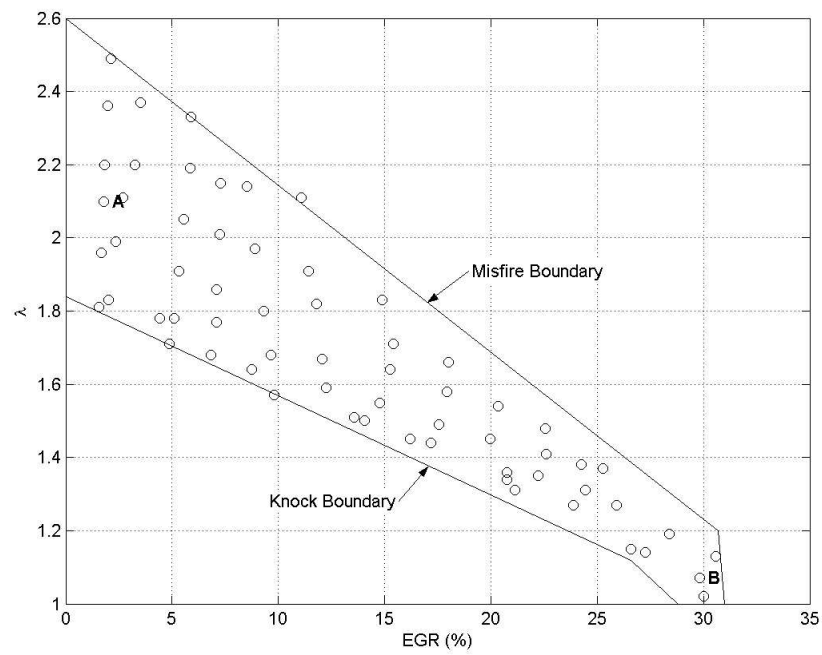
Figure 4.2: HCCI Operation Region for PRF20
