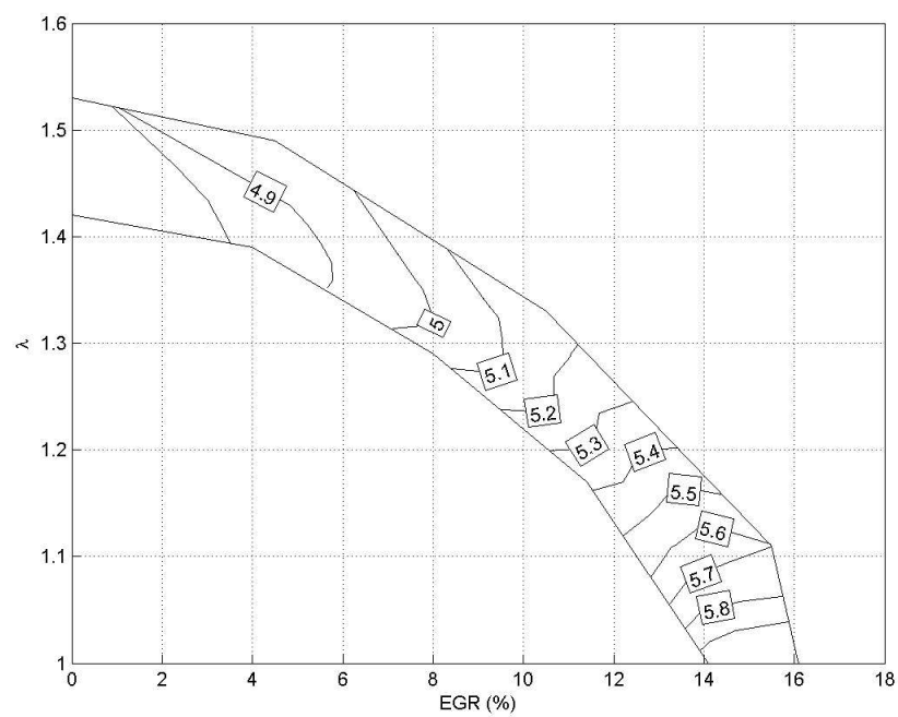
Figure 4.22: IMEP in bar for PRF60
