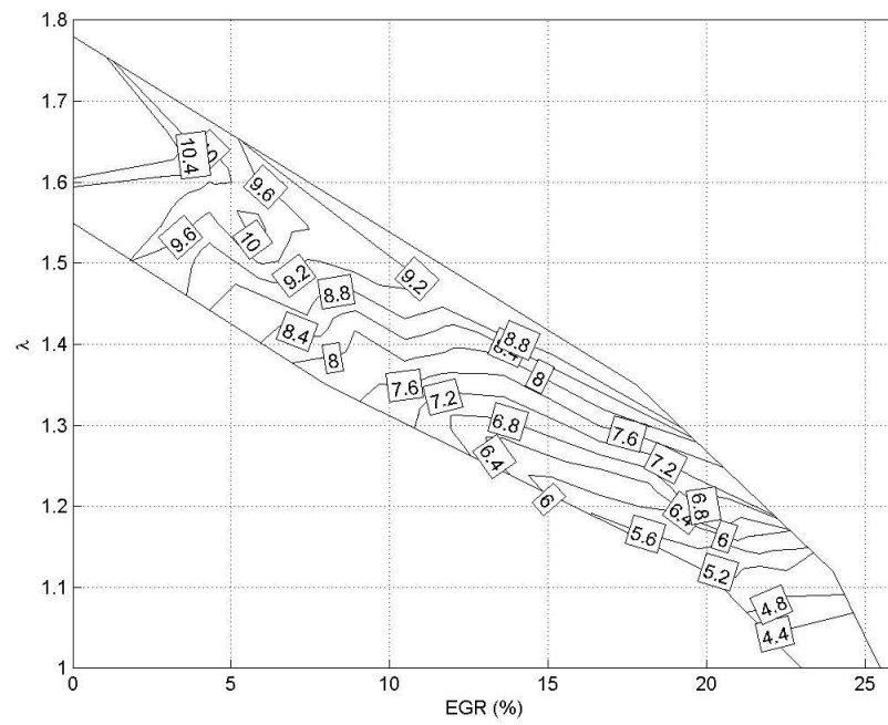
Figure 4.16: Indicated Specific CO in g/kWhr for PRF40
