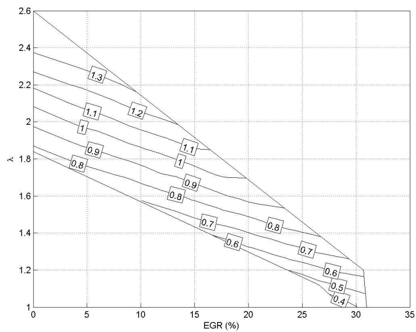
Figure 4.3: Effective Dilution for PRF20
