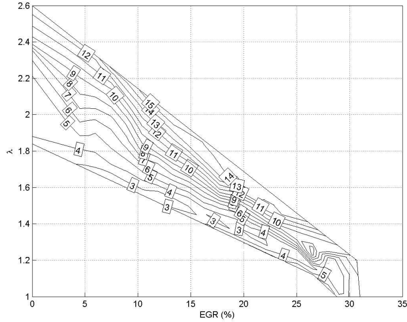
Figure 4.10: Burn Duration (10-90% Burnt) in degrees for PRF20
