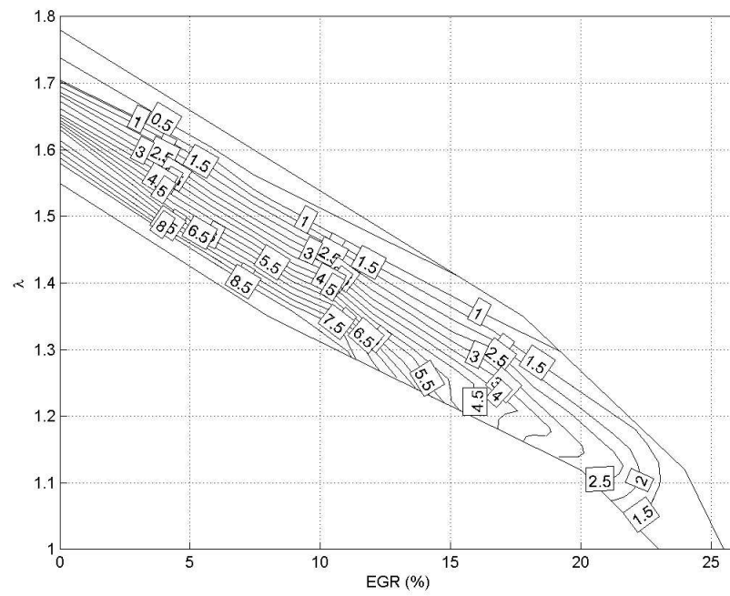
Figure 4.14: Indicated Specific \text{NO}_x in g/kWhr for PRF40
