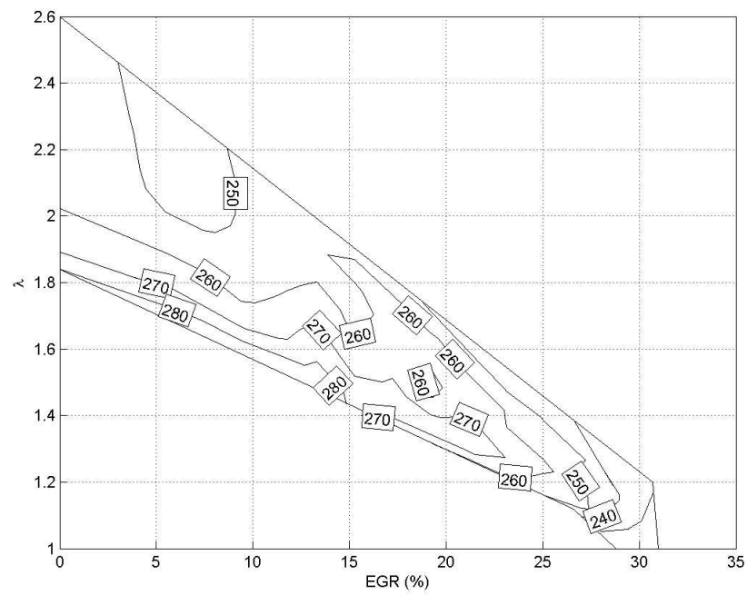
Figure 4.8: ISFC in g/kWhr for PRF20
