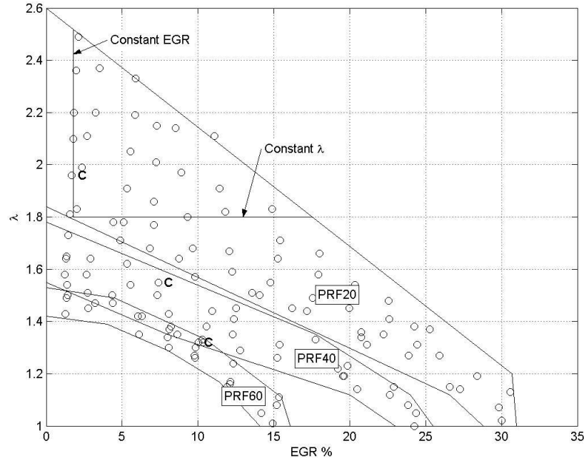
Figure 5.1: Operating Region For PRF20, PRF40 and PRF60
