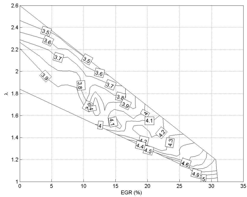
Figure 4.4: IMEP in bar for PRF20
