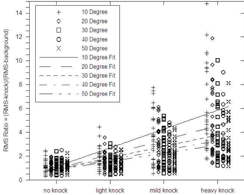
Figure 3.1: RMS Bandpass and Audible Knock Correlation
