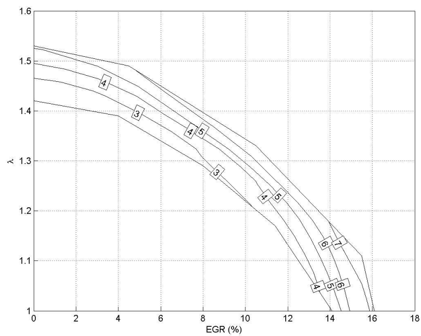
Figure 4.28: Burn Duration (10-90% Burnt) in degrees for PRF60
