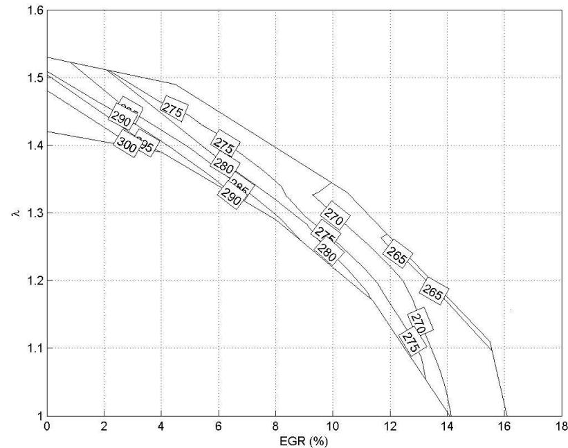
Figure 4.26: ISFC in g/kWhr for PRF60
