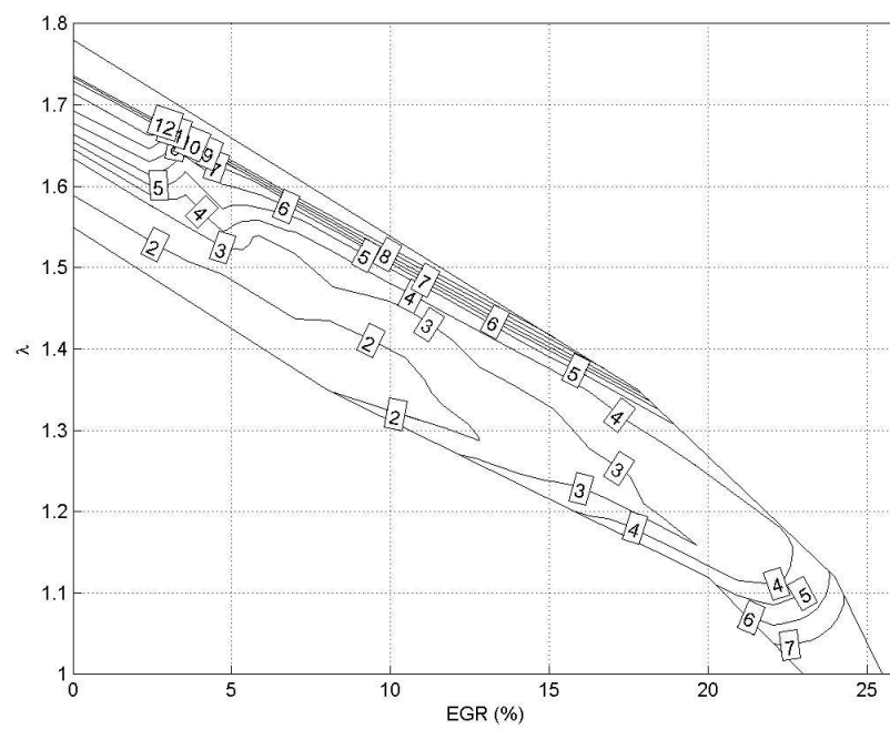
Figure 4.19: Burn Duration (10-90% Burnt) in degrees for PRF40
