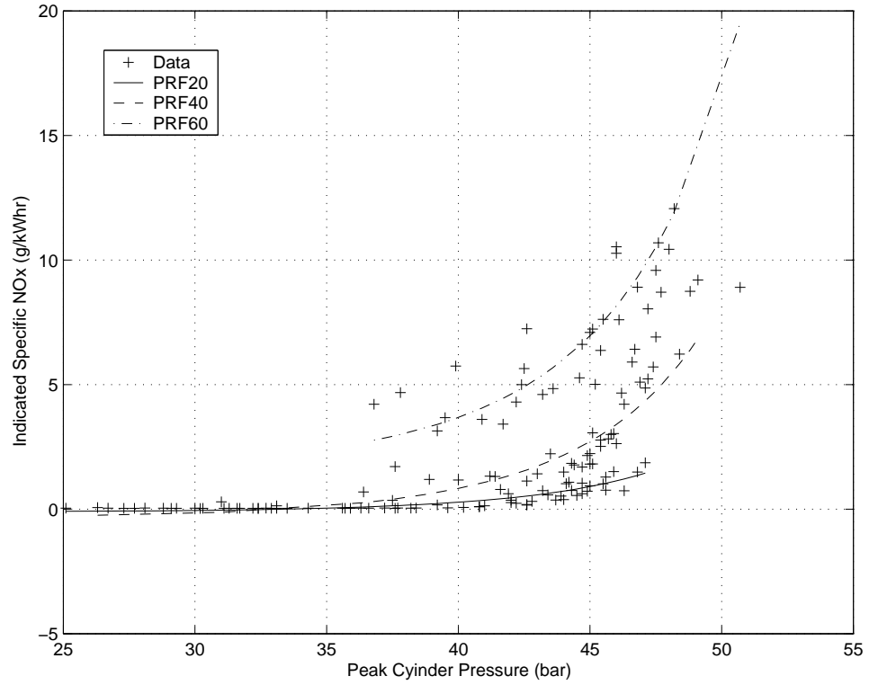
Figure 5.3: \text{NO}_x versus Peak Pressure Correlation
