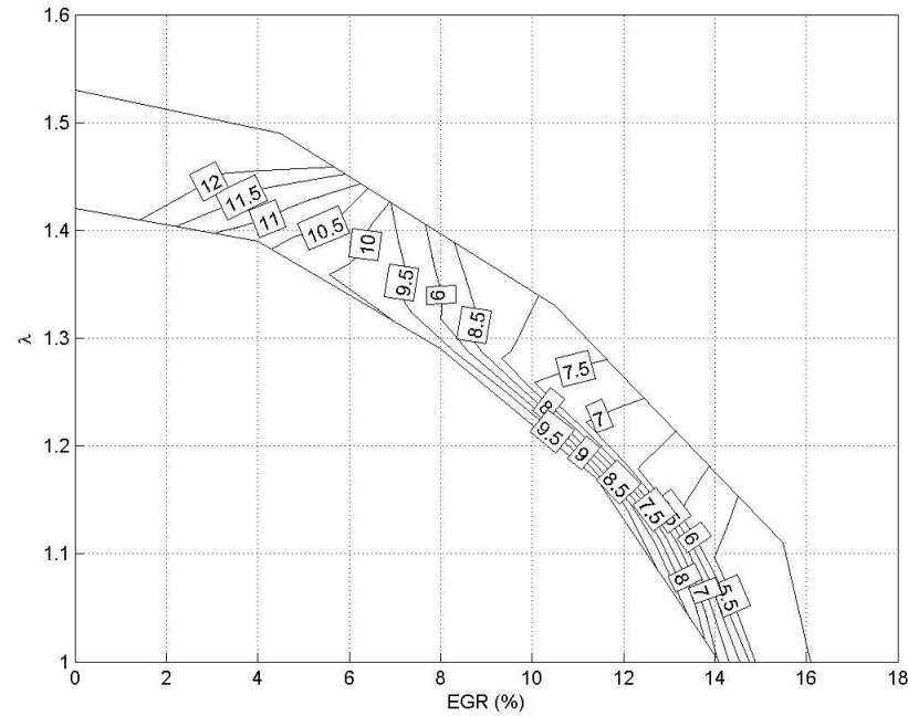
Figure 4.25: Indicated Specific CO in g/kWhr for PRF60
