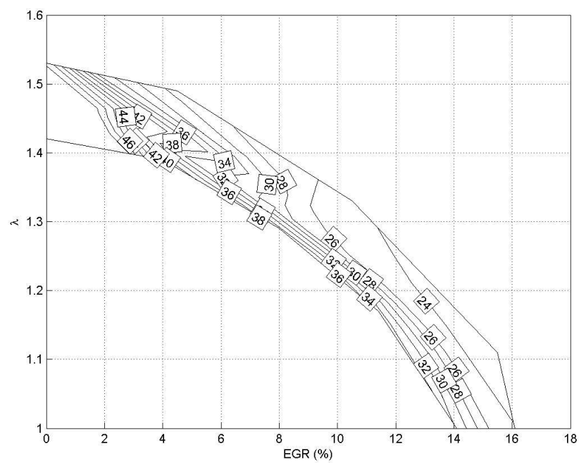
Figure 4.24: Indicated Specific HC in g/kWhr for PRF60
