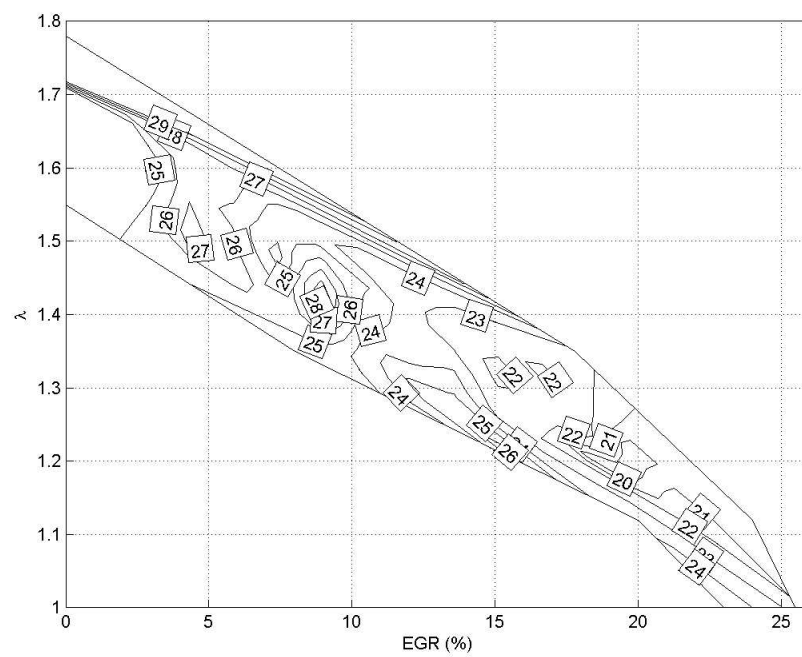
Figure 4.15: Indicated Specific HC in g/kWhr for PRF40
