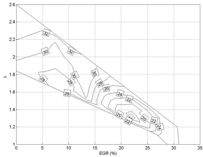
Figure 4.6: Indicated Specific HC in g/kWhr for PRF20
