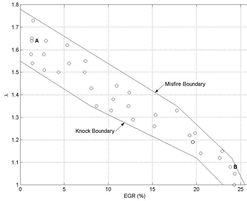
Figure 4.11: HCCI Operating Region for PRF40
