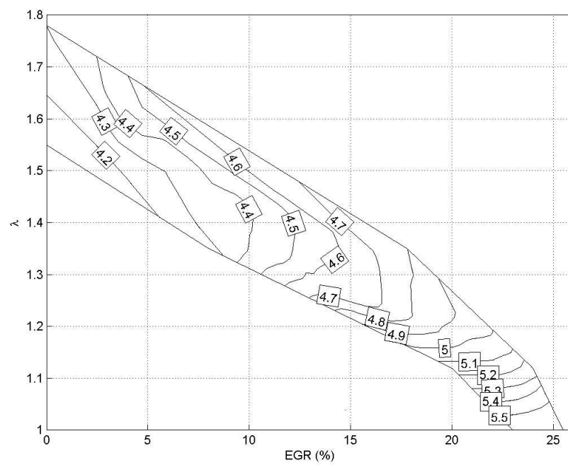
Figure 4.13: IMEP in bar for PRF40
