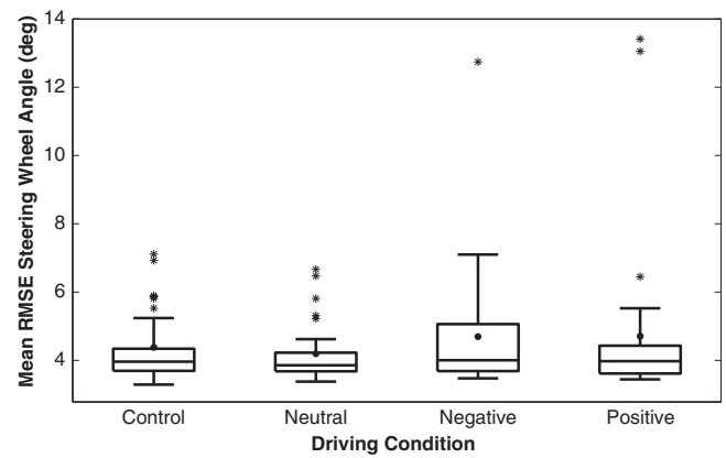
Fig. 3. Distribution of mean steering wheel angle, in the form of root mean square error (RMSE), within each driving condition.
