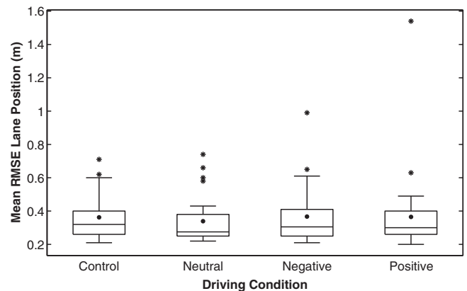
Fig. 4. Distribution of mean lane position, in the form of root mean square error (RMSE), within each driving condition.
