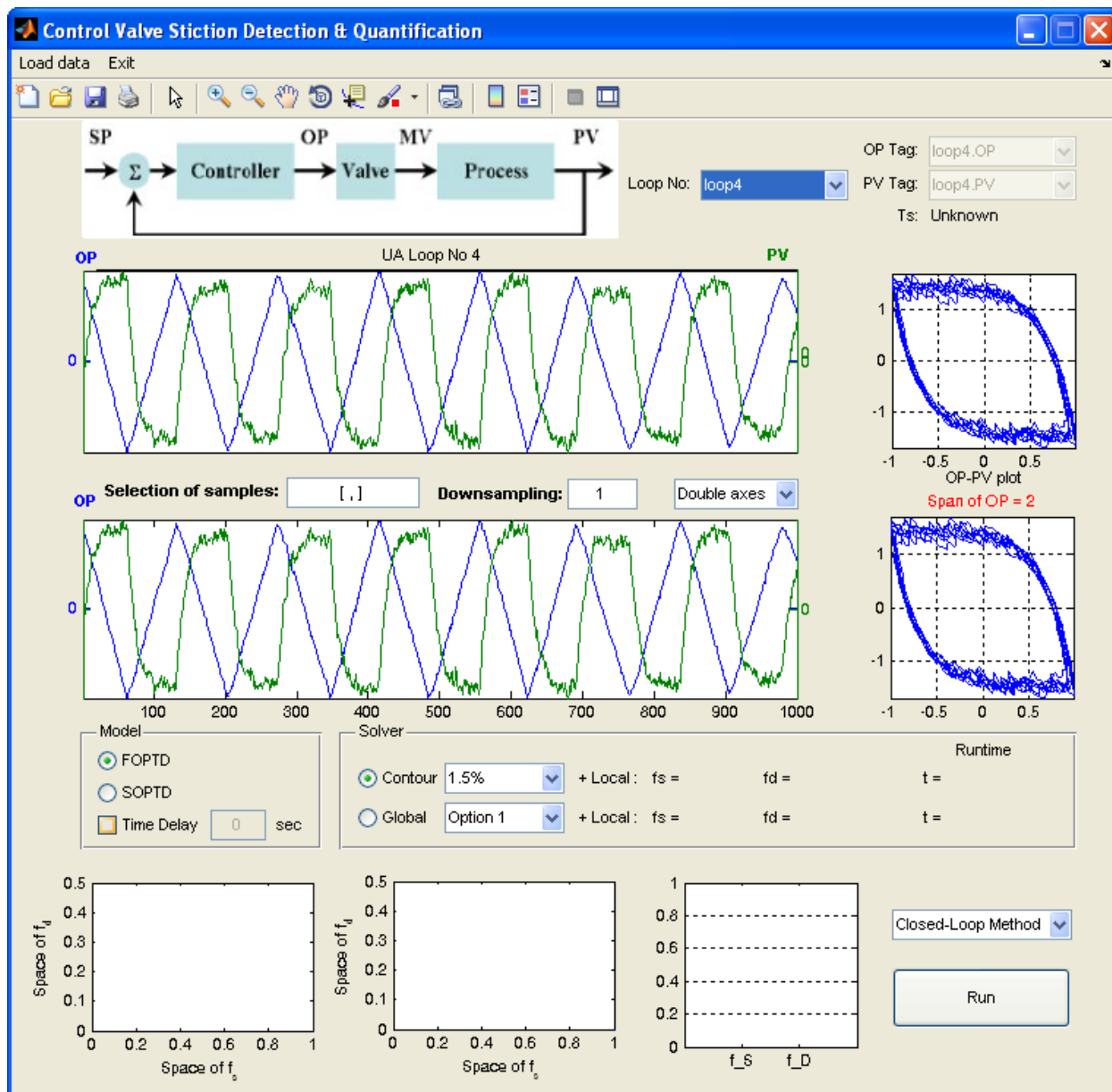
Figure 12: Screen shot 1 for the example
