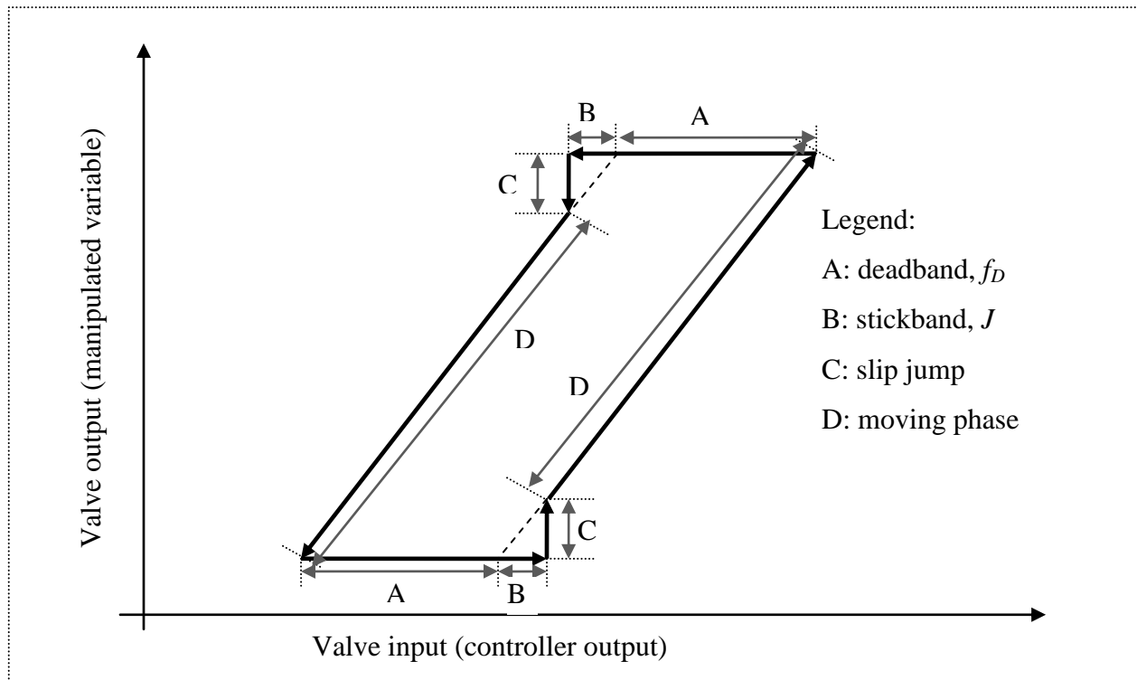
Figure 5: Phase plot for the typical behaviour of valve with stiction (after, (Shoukat Choudhury, Thornhill, & Shah, 2005))
