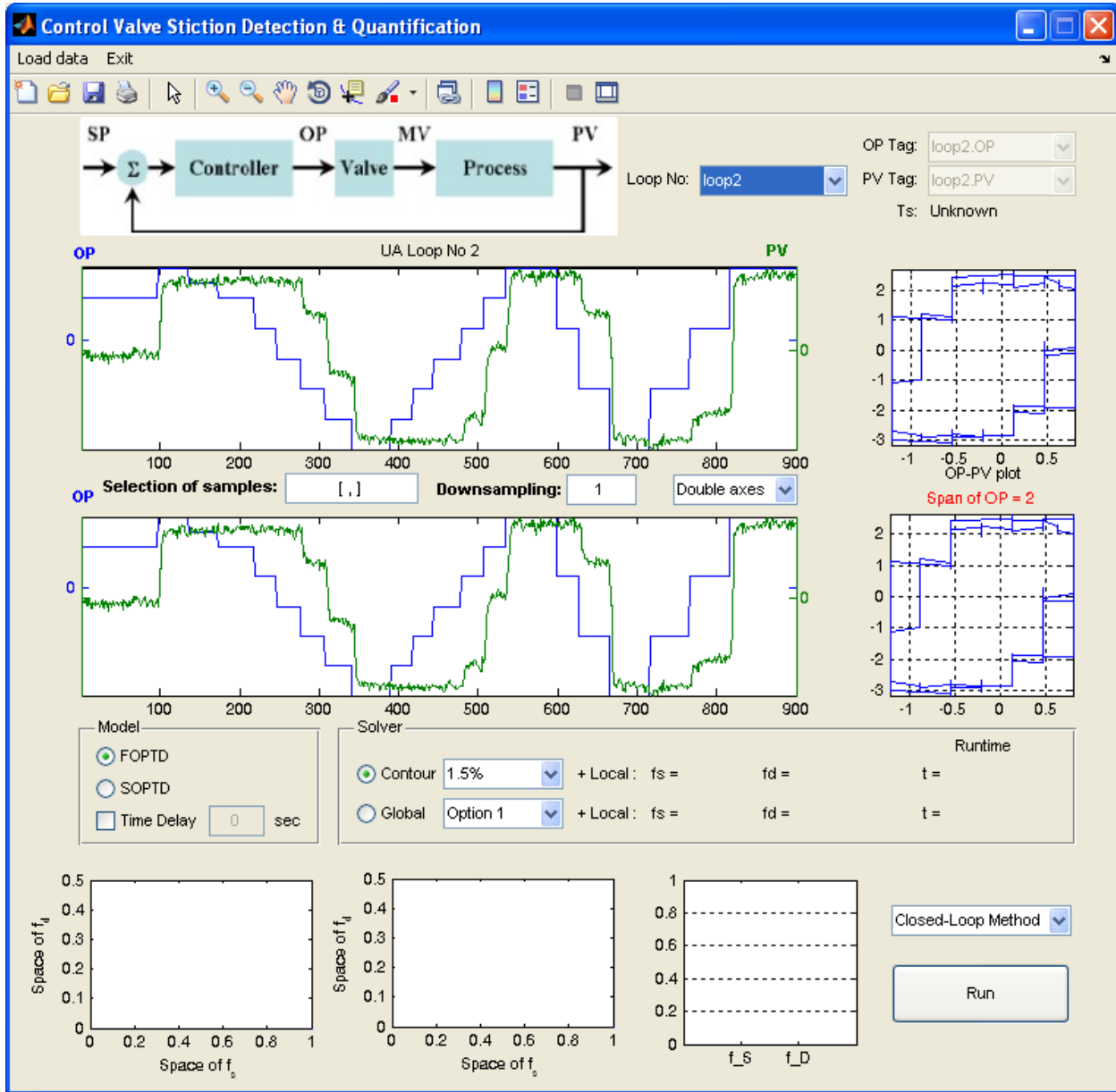
Figure 3: Screen shot after loading the data
