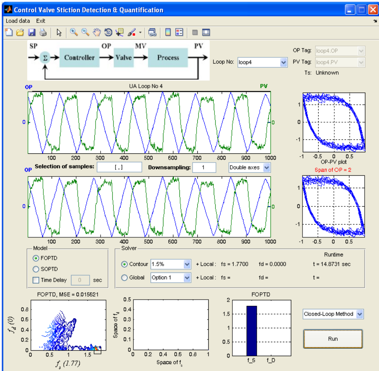
Figure 4: Screen shot after clicking "Run"
