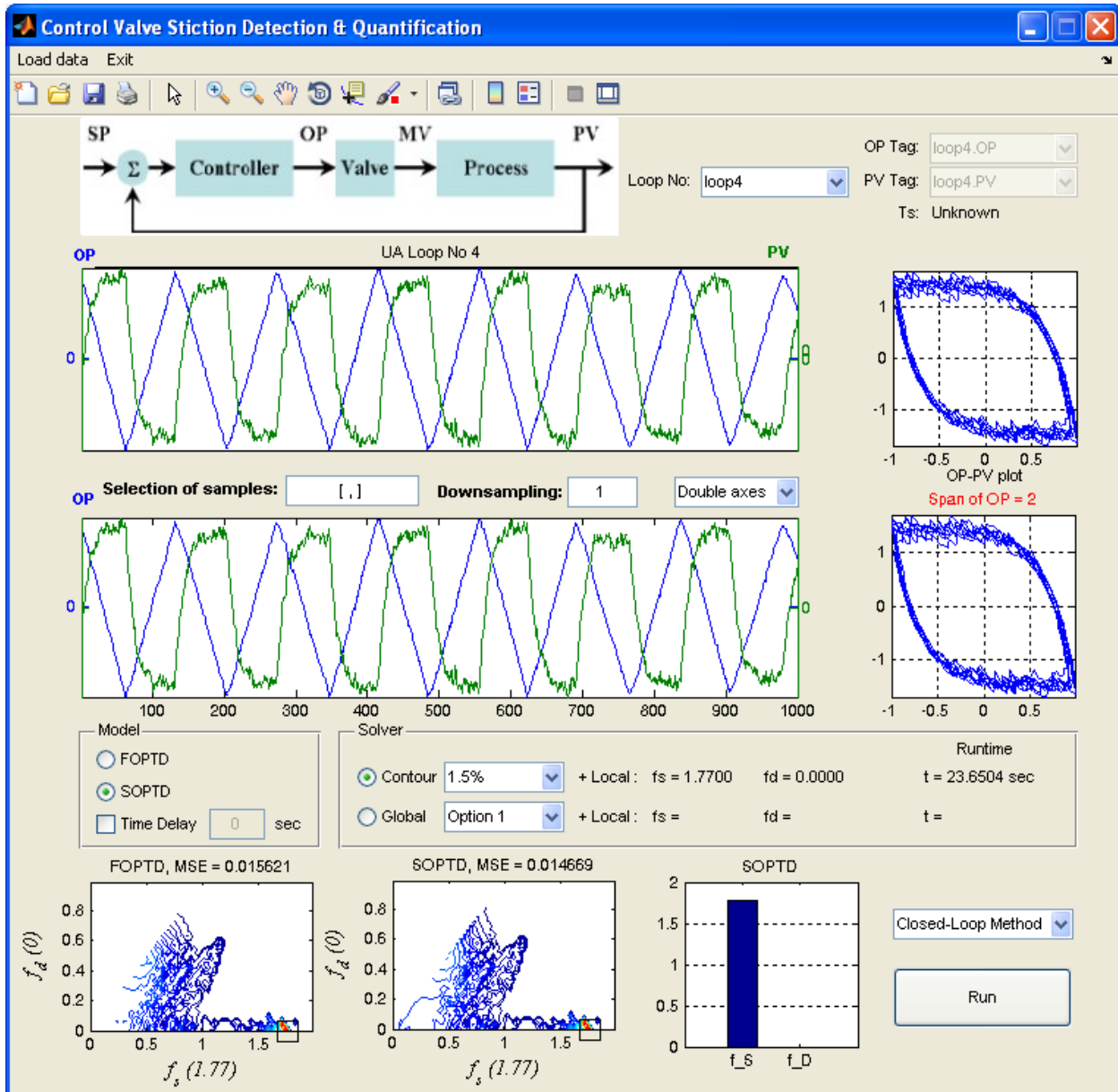
Figure 14: Second-order Model Results
