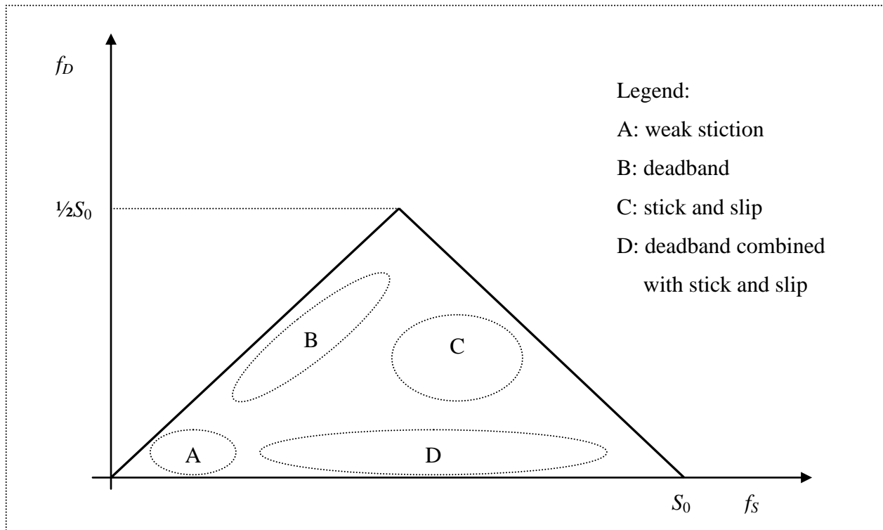
Figure 6: f_D as a function of f_S . The crucial regions are also highlighted. (after (Lee, Ren, & Huang, 2008))
