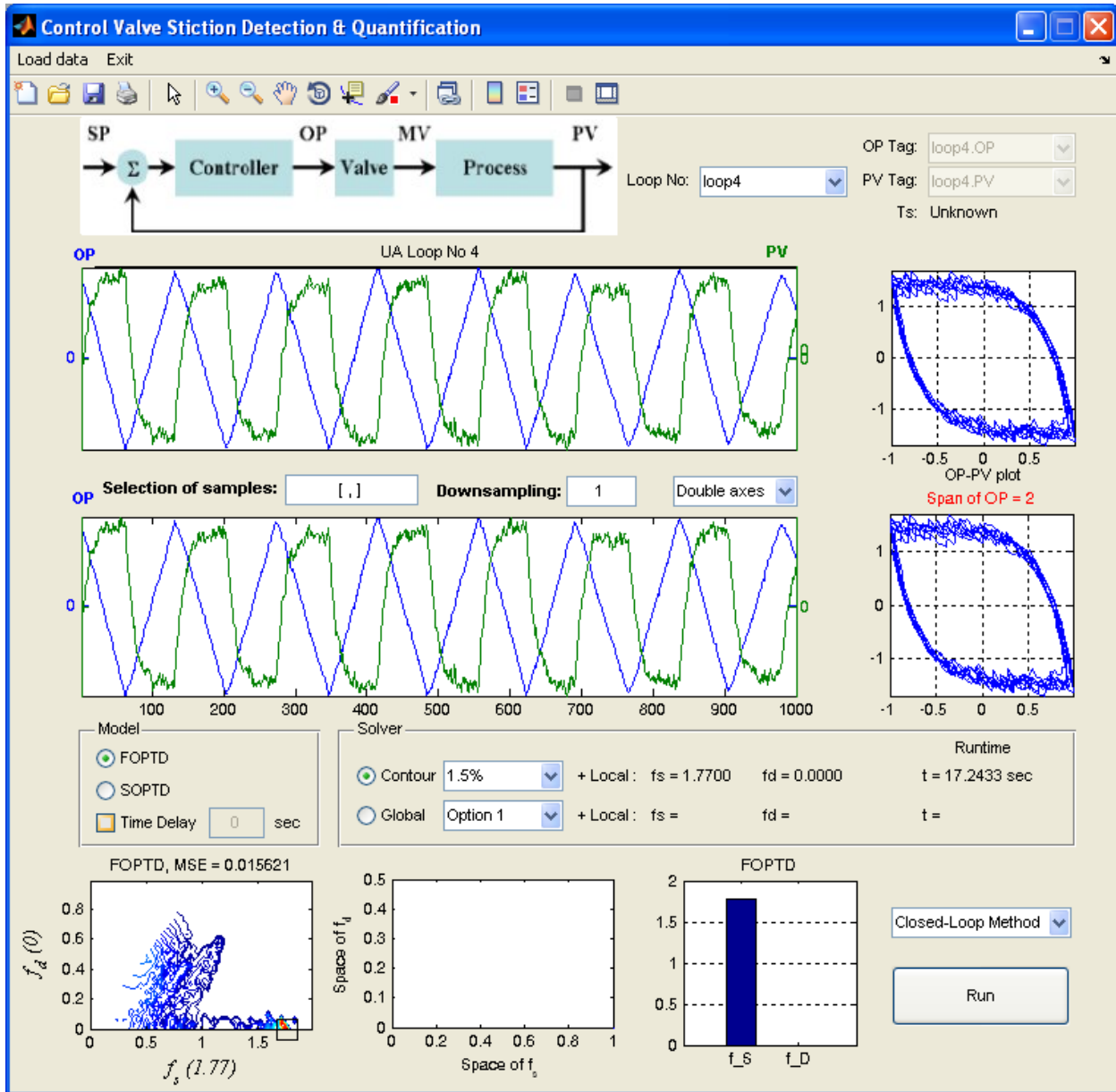
Figure 13: Screen shot 2 for the example
