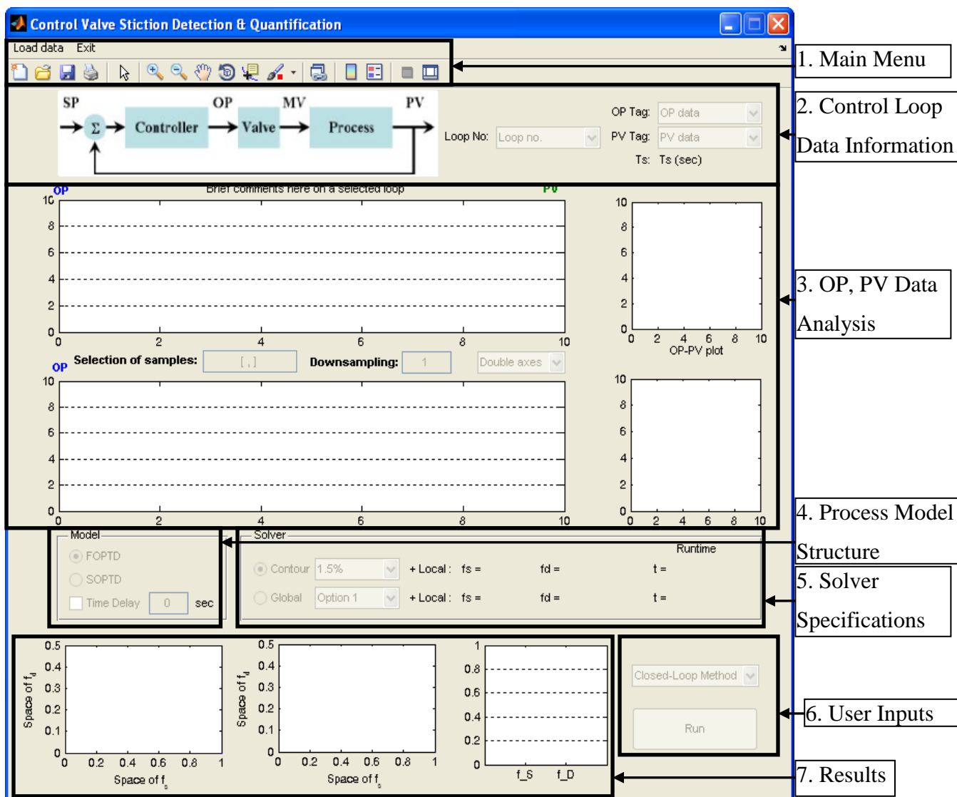
Figure 9: The main GUI for this toolbox, with the main regions highlighted
