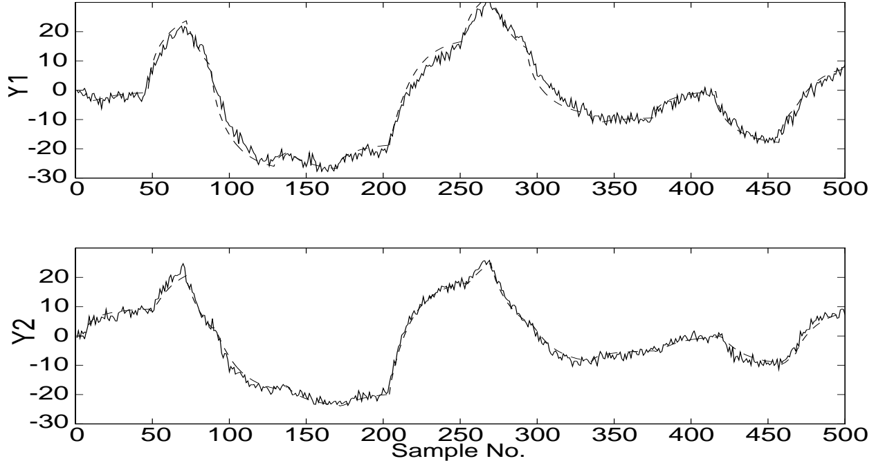
Figure 5: Cross validation for Wood-Berry Column : Model (dashed line) and Actual Plant (solid line) responses
