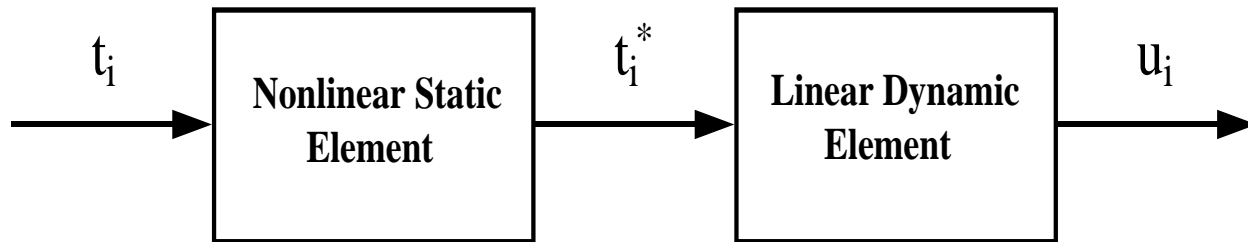
Figure 3: The Hammerstein Model
