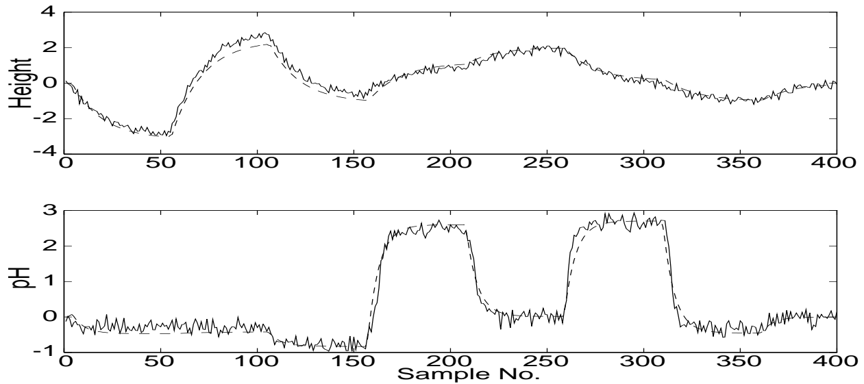
Figure 7: Cross validation with the identified PLS-Hammerstein model for the acid-base neutralization system : Model (dashed line) and Actual Plant (solid line)
