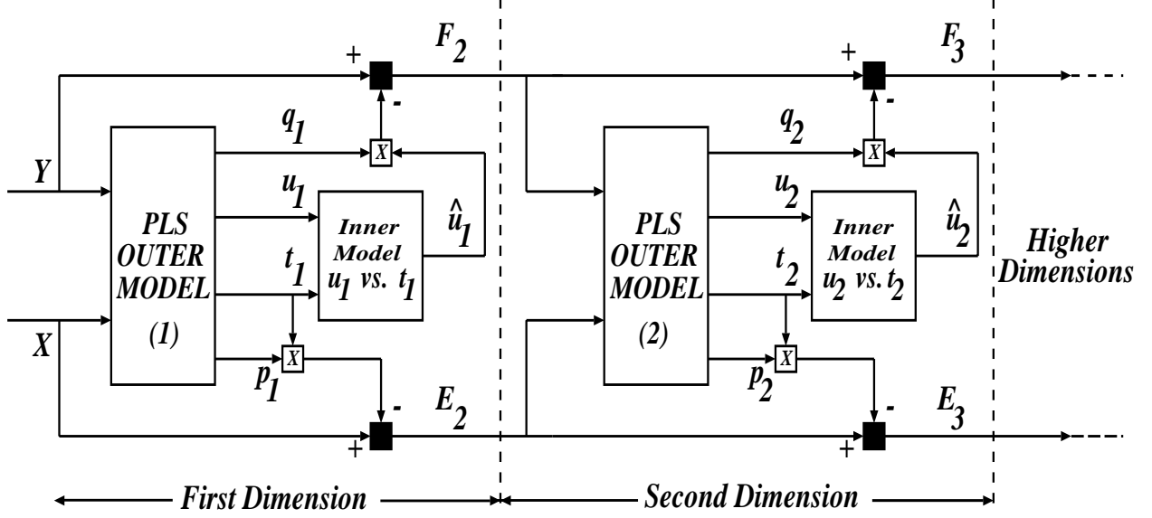
Figure 1: The Standard Linear PLS Algorithm
