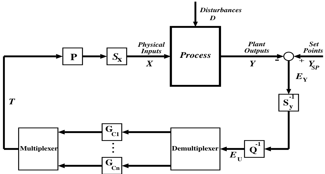
Figure 10: Feedback control using the PLS Framework : The Kaspar - Ray scheme for Linear Systems
