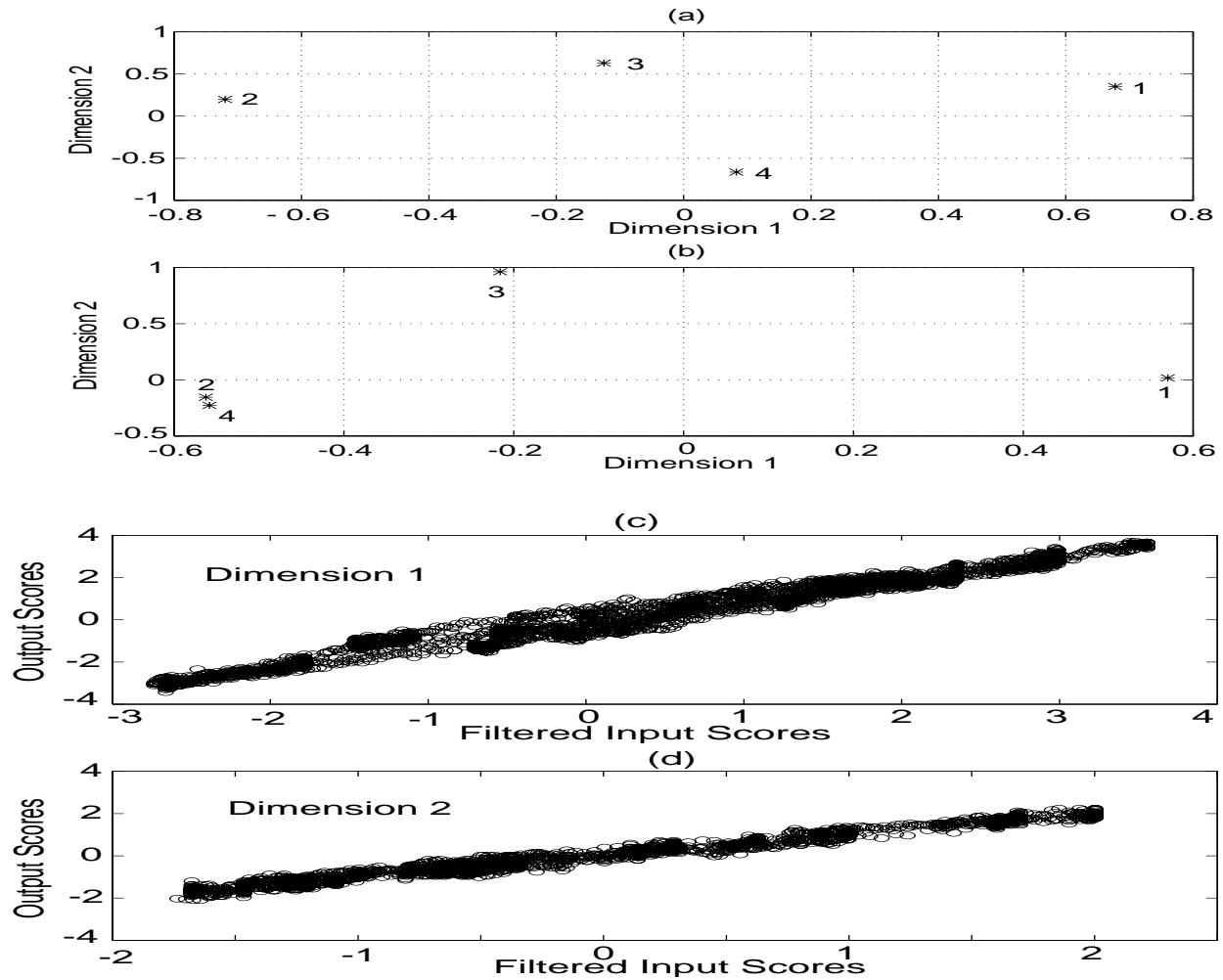
Figure 8: Results of the Dynamic PLS modelling strategy for the Alatiqi-Luyben Distillation Column : (a) Loadings plot for the inputs (b) Loadings plot for the outputs (c) Inner relationship plot for dimension 1 and (d) Inner relationship plot for dimension 2
