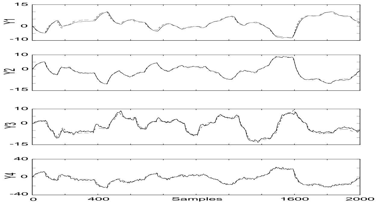
Figure 9: Cross validation for the Alatiqi-Luyben Distillation Column : Model (dashed line) and Actual Plant (solid line) responses
