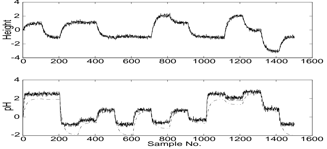
Figure 6: Comparison of Model fit for the acid-base neutralization system: PLS-Hammerstein model (dashed line), Linear model (dashed-dot) and Actual plant (solid line)
