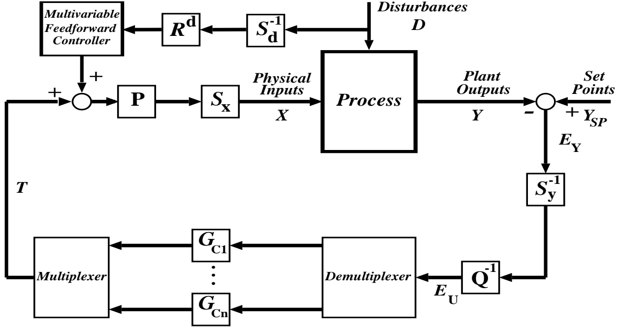
Figure 17: The combined feedback - feedforward control strategy for linear systems : The PLS Framework
