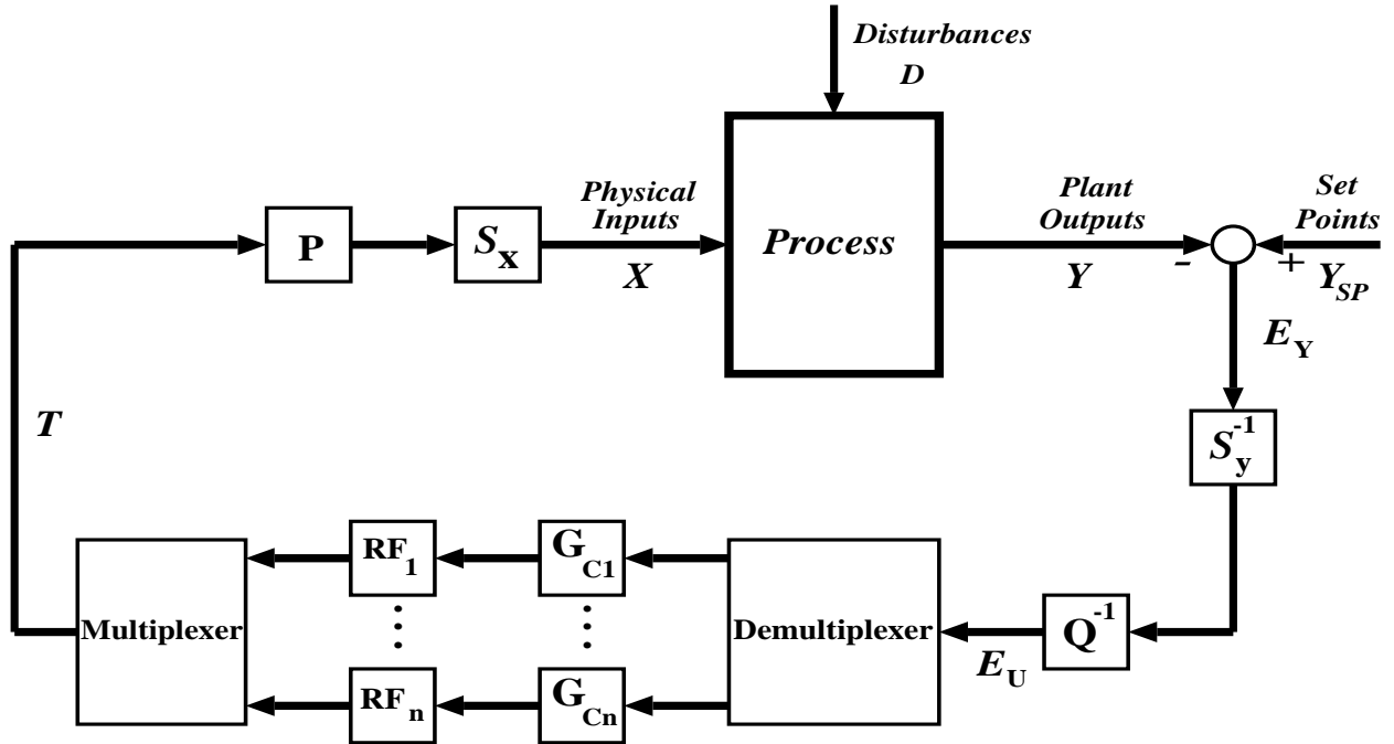
Figure 11: Feedback Control using the PLS Framework for systems modelled by the Hammerstein Structure
