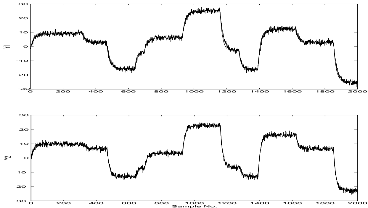
Figure 4: Identification of the Wood-Berry Column : Model (dashed line) and Actual Plant (solid line) responses
