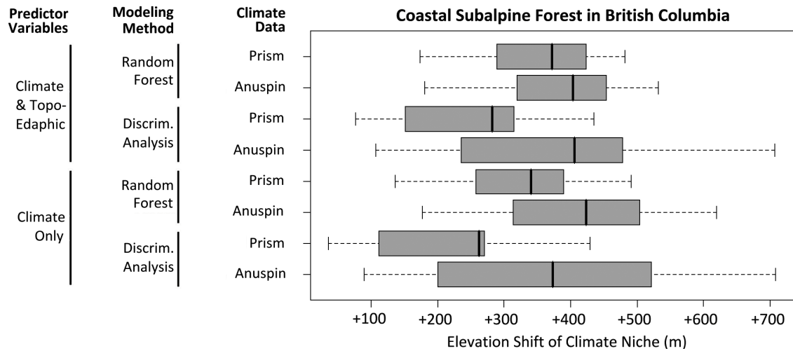
Figure 4-3. Variation in bioclimate envelope modeling results for different datasets and methods (left) and different climate change projections (boxplots). The measured variable is the 50 th percentile of elevation of the subalpine forest biome, reported as elevation shift in meters relative to the 1960-1990 reference climate projection.
