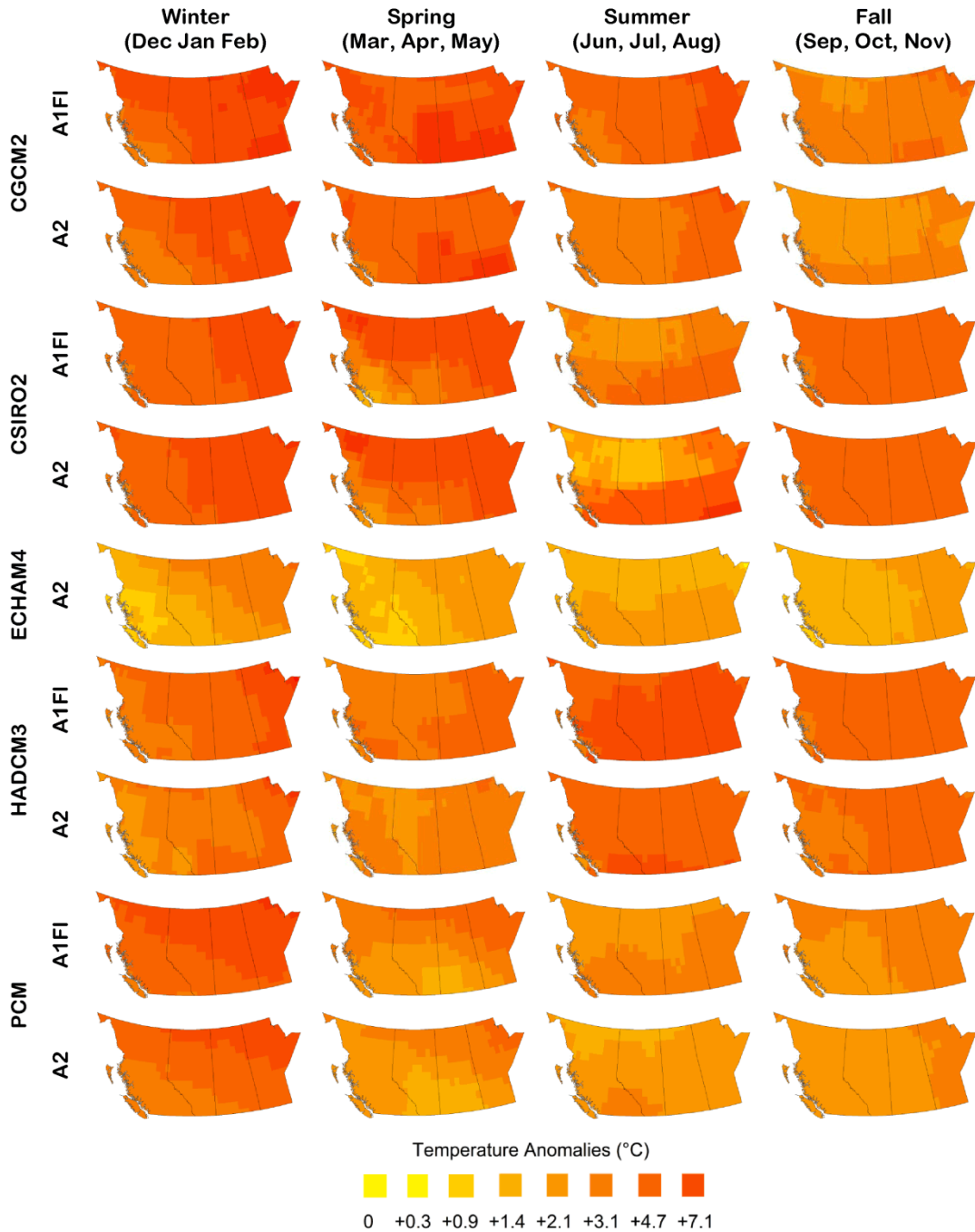
Figure 2-7. Projected mean seasonal 2050s temperature anomalies expressed in degree Celsius for western Canada for two emission scenarios (A1FI and A2) realized by five general circulation models -GCMs (CGCM2, CSIRO2, ECHAM4, HADCM3 and PCM).
