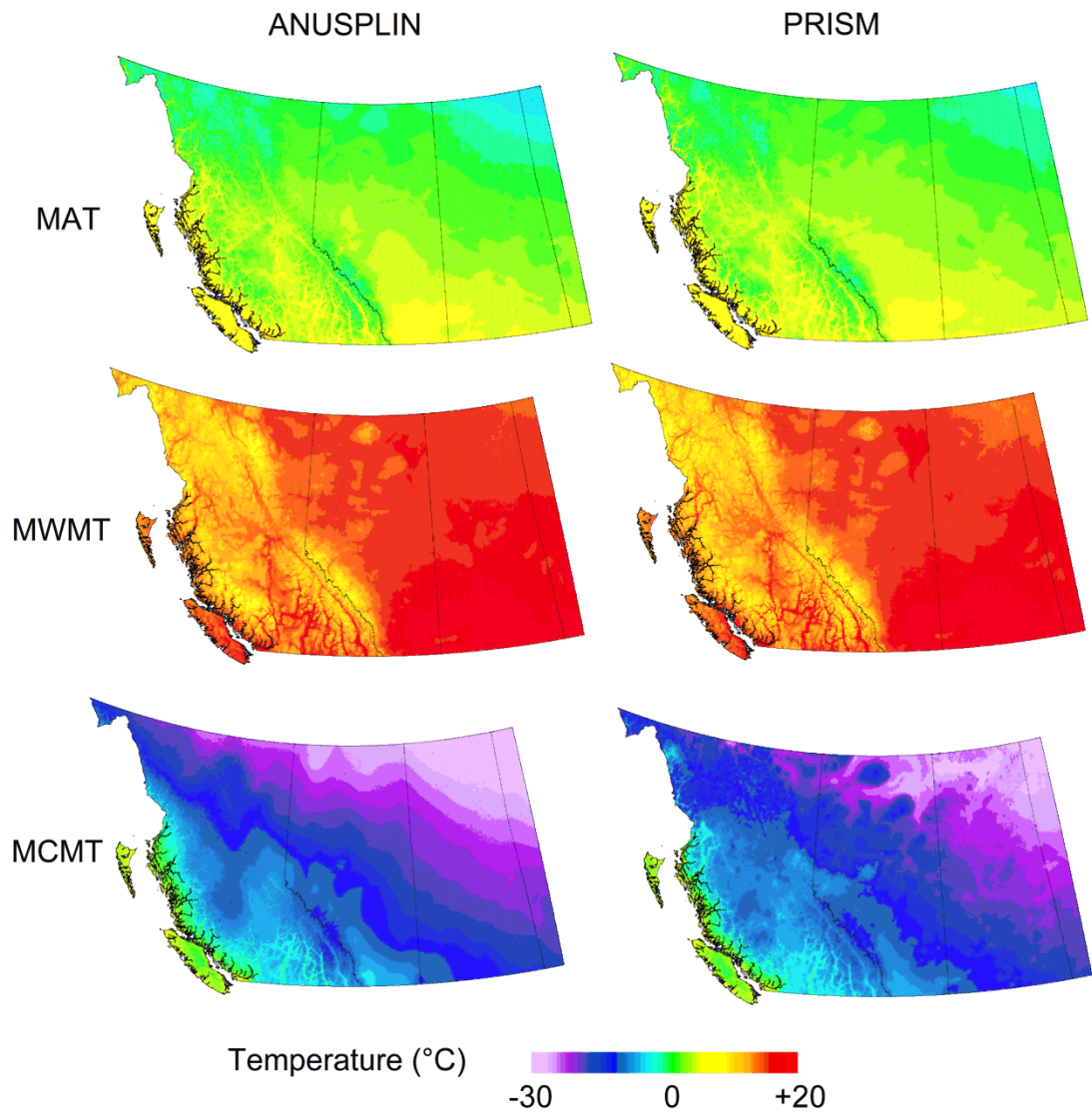
Figure 2-2. Western Canada 1961-1990 normal mean annual temperature-MAT, mean July temperature-MWMT and mean January temperature-MCMT grids based on ANUSPLIN and PRISM interpolation techniques.
