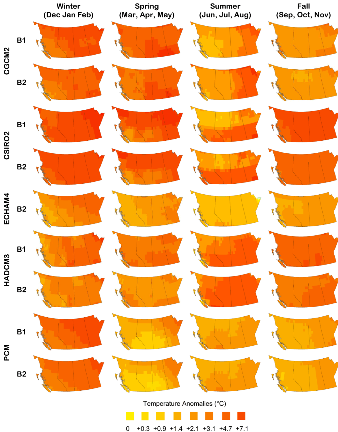
Figure 2-8. Projected mean seasonal 2050s temperature anomalies expressed in degrees Celsius for western Canada for two emission scenarios (B1 and B2) realized by five general circulation models-GCMs (CGCM2, CSIRO2, ECHAM4, HADCM3 and PCM).
