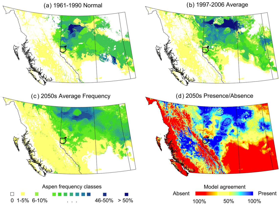
Figure 4-6. Predicted aspen frequencies for under for (a) the 1961-1990 climate normal period, representing the model training data, (b) a recent 10-year average, representing observed climate trends over the last 25 years relative to the climate normal, (c) average aspen frequency projections for the 2050s and (d) model agreement with respect to suitable aspen habitat predicted for the 2050s. The G16 management area for Query 4 is shown as a black outline.
