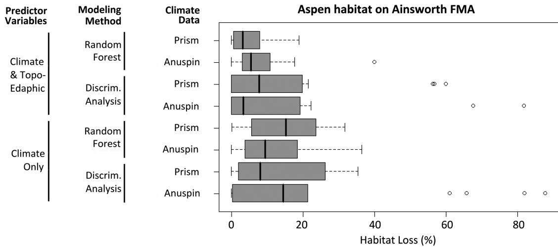
Figure 4-5. Variation in bioclimate envelope modeling results for different datasets and methods (left) and different climate change projections (boxplots). The measured variable is the area of projected aspen habitat, reported as percent loss relative to the 1960-1990 reference climate projection
