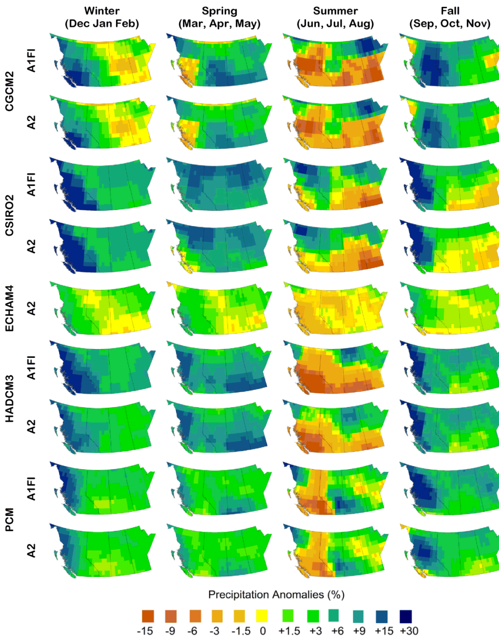
Figure 2-9. Projected mean seasonal precipitation 2050s anomalies expressed as percent change for western Canada for two emission scenarios (A1FI and A2) realized by five general circulation models-GCMs (CGCM2, CSIRO2, ECHAM, HADCM3 and PCM).
