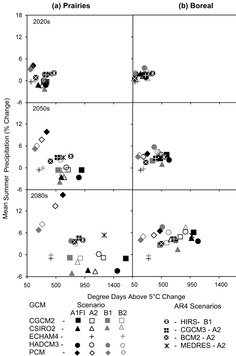
Figure 2-12. Relative change in projected degree days above 5°C and mean summer (May-September) precipitation for Prairies (A) and the southern Boreal (B) western Canada biomes based on ensemble runs of 4 SRES scenario families and 5 general circulation models, as well as 4 individual model runs selected from the IPCC's Fourth Assessment Report (AR4) for the 2020s, 2050s and the 2080s.
