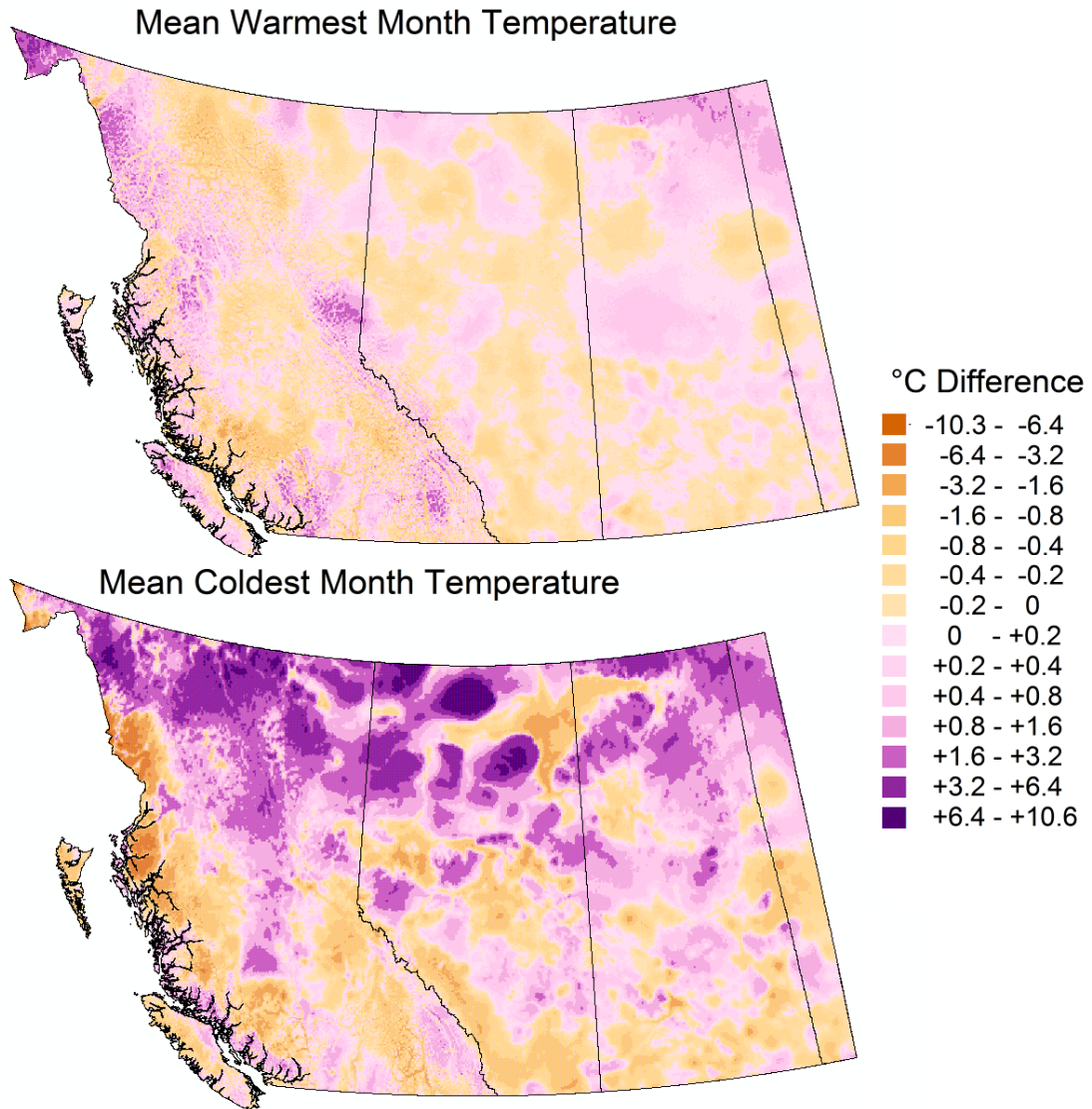
Figure 2-5. Difference between ANUSPLIN and PRISM 1961-1990 normals for western Canada for mean July and mean January temperature.
