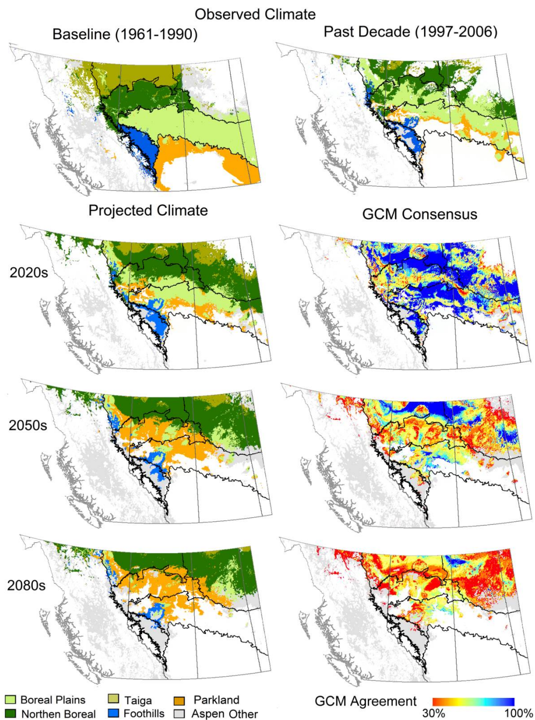
Figure 5-3. Aspen seedzone climate envelope under baseline (1961-1990), recent decade (1997-2006) and future climate scenarios for the 2020s, 2050s and 2080s, and general circulation model (GCM) consensus for predicted shifts under future climate. Outlines of current aspen seedzones are added for orientation.
