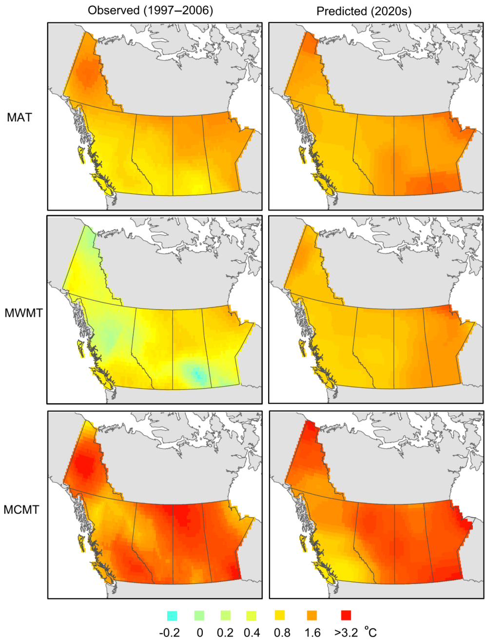
Figure 3-3. Maps of anomalies (deviations from 1961 - 1990 normals) of a recent 10-year average (1997 - 2006) and predicted by CGCM2-B2 for the 2020s for mean annual temperature (MAT), mean warmest month temperature (MWMT) and mean coldest month temperature (MCMT).
