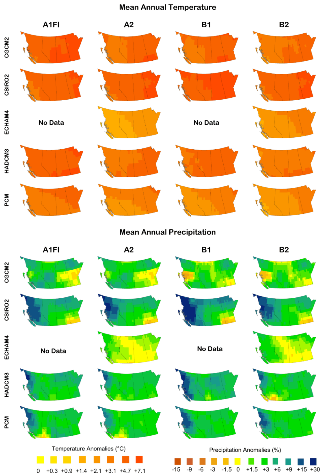
Figure 2-6. Projected 2050s mean annual temperature and mean annual precipitation anomalies for western Canada from five GCMs (CGCM2, CSIRO2, ECHAM4, HADCM3 and PCM) for four emission scenarios (A1FI, A2, B1 and B2).
