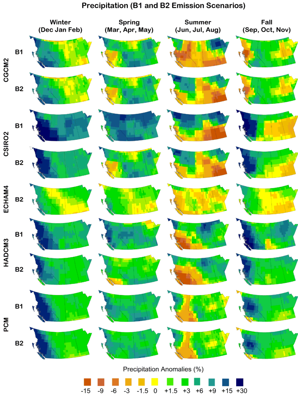
Figure 2-10. Projected mean seasonal precipitation 2050s anomalies expressed as percent change for western Canada for two emission scenarios (B1 and B2) realized by five general circulation models-GCMs (CGCM2, CSIRO2, ECHAM, HADCM3 and PCM).
