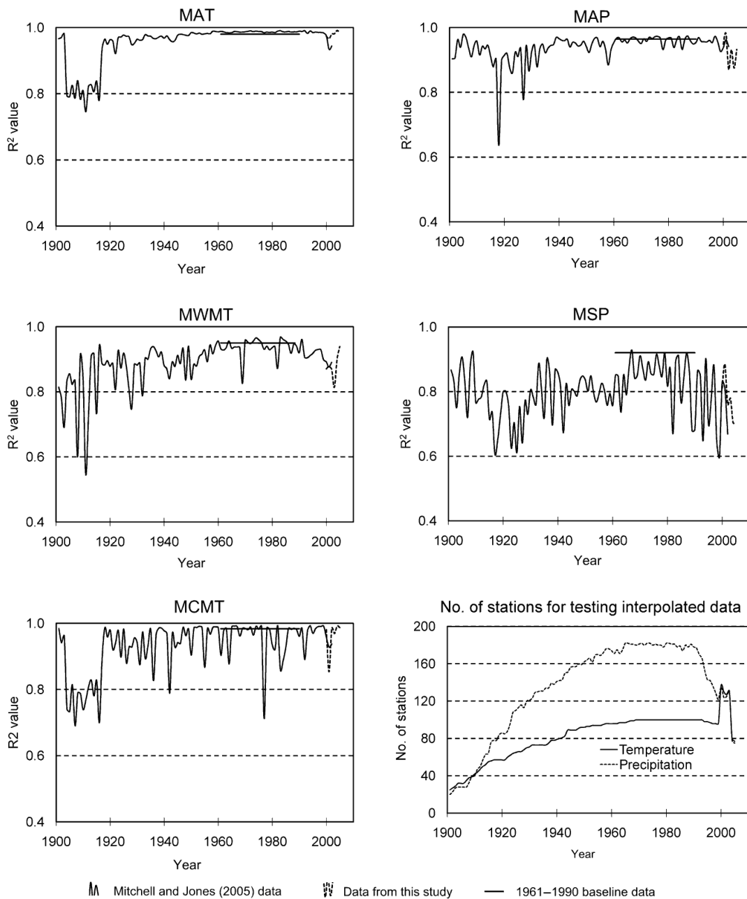
Figure 3-2. R^2 between observed and interpolated mean annual temperature (MAT), mean warmest month temperature (MWMT), mean coldest month temperature (MCMT) data, mean annual precipitation (MAP) and mean summer precipitation (MSP) for the 1901–2002 period and corresponding values for the 1961–1990 normals comparison with observed data. Number of stations for data comparison for each year is also shown.
