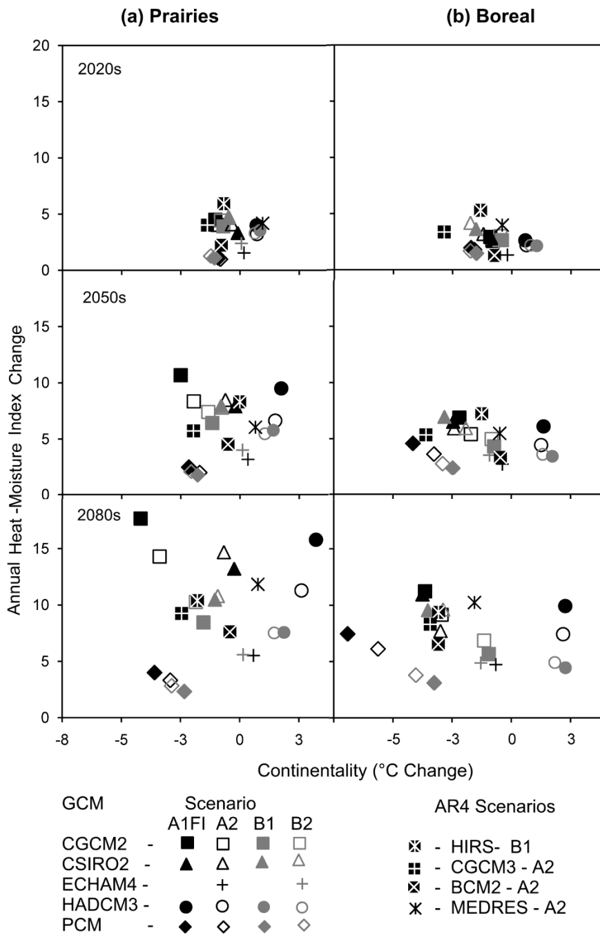
Figure 2-14. Relative change in projected difference between warmest and coldest month temperature (temperature difference) and annual heat moisture index for Prairies (A) and the southern Boreal (B) western Canada biomes based on ensemble runs of 4 SRES scenario families and 5 general circulation models, as well as 4 individual model runs selected from the IPCC's Fourth assessment Report (AR4) for the 2020s, 2050s and the 2080s.
