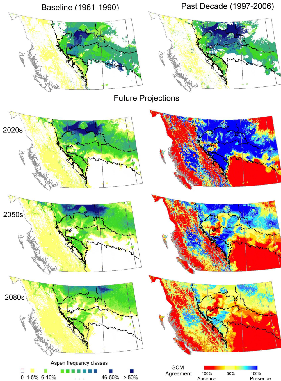
Figure 5-2. Aspen frequency under baseline (1961-1990), recent decade (1997-2006) and projected future climate scenarios for the 2020s, 2050s and 2080s time slices. General circulation model (GCM) agreement for modeled aspen frequency under future climate is also provided. Outlines of current aspen seedzones are added for orientation.
