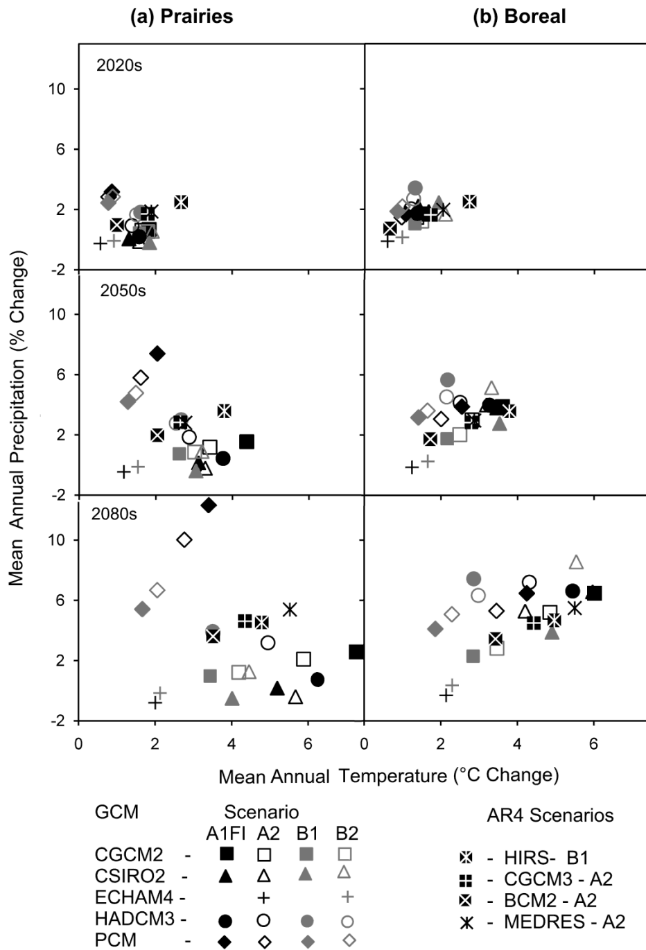
Figure 2-11. Relative change in projected mean annual temperature and mean annual precipitation for Prairies (A) and the southern Boreal (B) western Canada biomes based on ensemble runs of 4 SRES scenario families and 5 general circulation models, as well as 4 individual model runs selected from the IPCC's Fourth Assessment Report (AR4) for the 2020s, 2050s and the 2080s.
