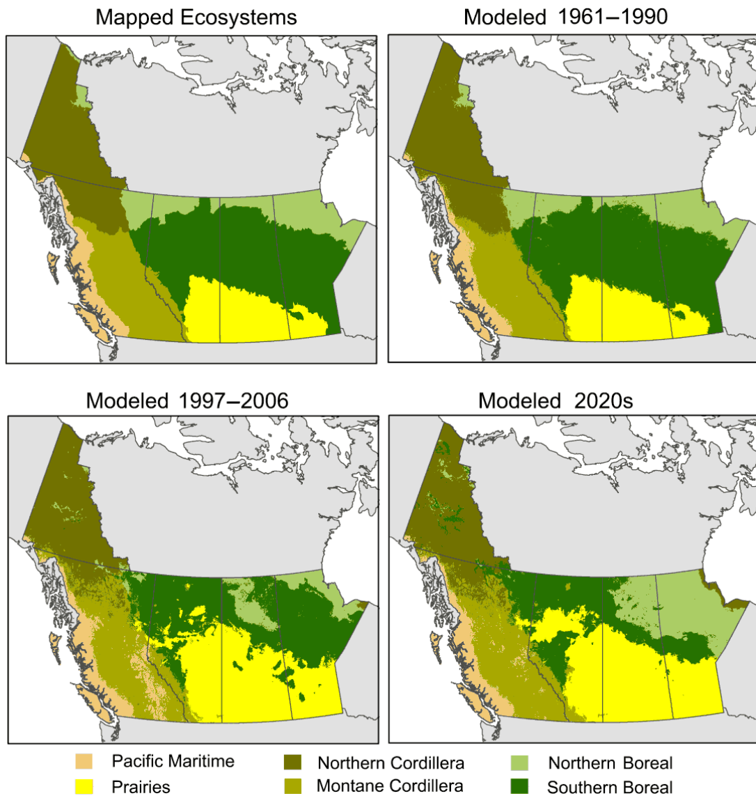
Figure 3-5. Mapped ecosystems and modeled ecosystem climate envelope based on baseline climate normals (1961 - 1990), a recent 10-year average (1997 - 2006) and projected climate for the 2020s based on the Canadian Global Circulation Model (CGCM2-B2).
