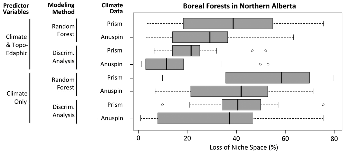
Figure 4-4. Variation in bioclimate envelope modeling results for different datasets and methods (left) and different climate change projections (boxplots). The measured variable is the area of projected boreal forest ecosystems, reported as percent loss relative to the 1960-1990 reference climate projection.
