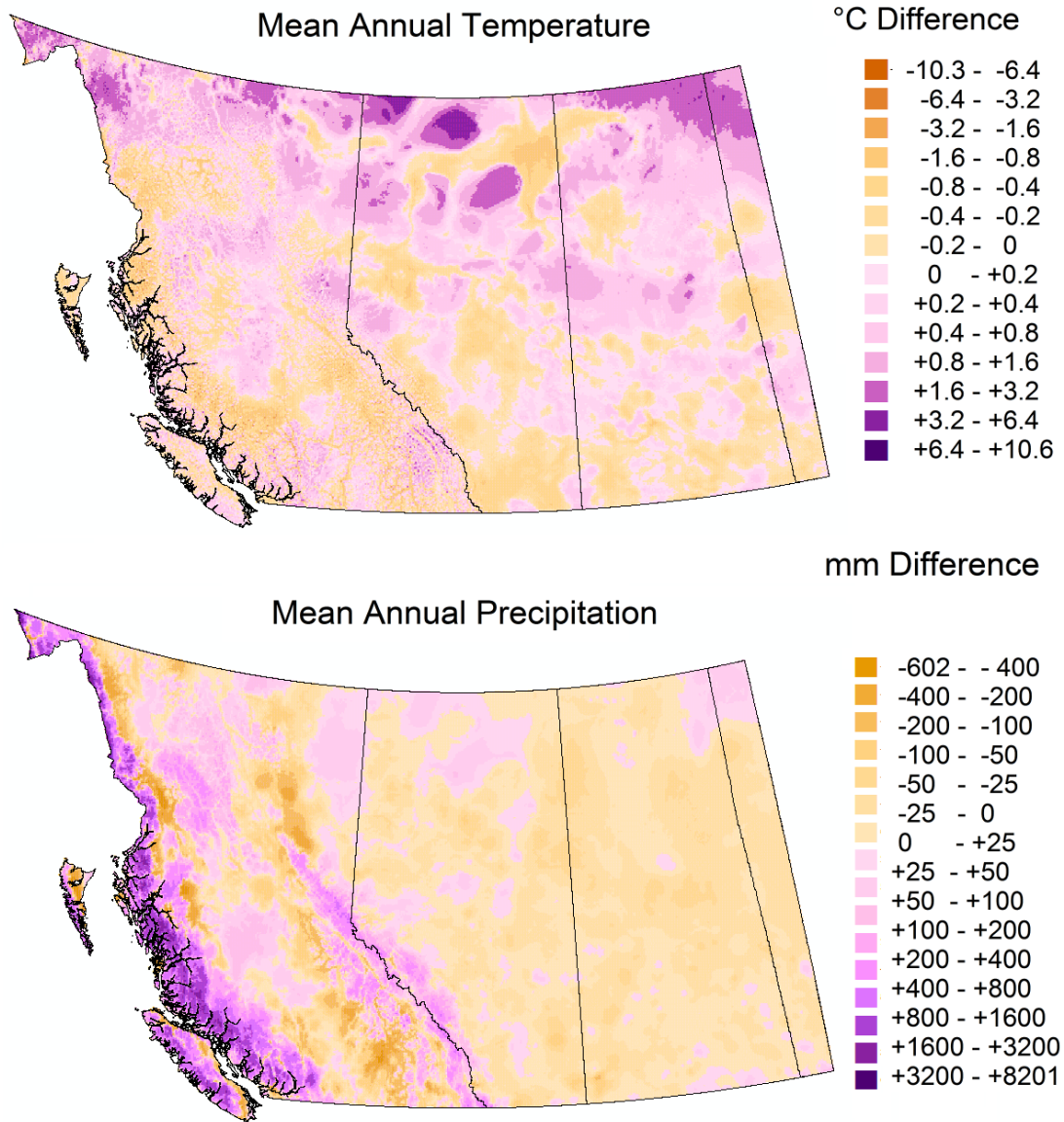
Figure 2-4. Difference between ANUSPLIN and PRISM 1961-1990 normals for western Canada for mean annual temperature and mean annual precipitation.
