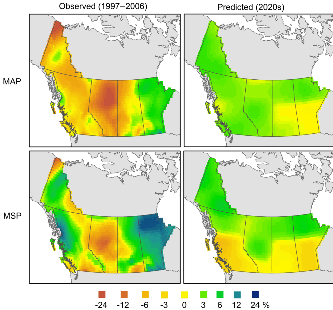
Figure 3-4. Maps of anomalies (deviations from 1961 - 1990 normals expressed as percentage) of a recent 10-year average (1997 - 2006) and predicted by CGCM2-B2 for the 2020s for mean annual precipitation (MAP) and mean summer precipitation (MSP).
