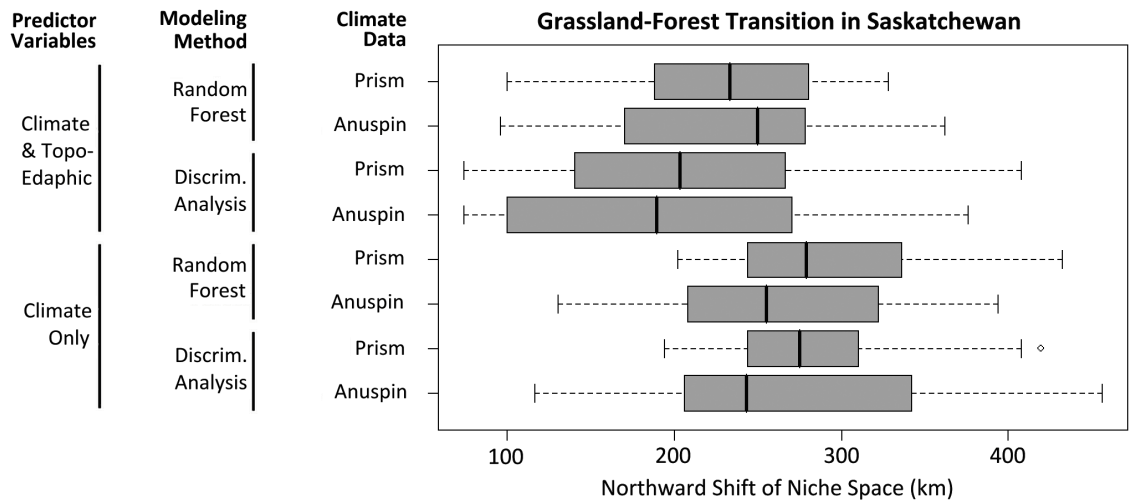
Figure 4-2. Variation in bioclimate envelope modeling results for different datasets and methods (left) and different climate change projections (boxplots). The measured variable is the 90 th percentile of latitude of projected grassland ecosystems, reported as northward shift in kilometer relative to the 1960-1990 reference climate projection.
