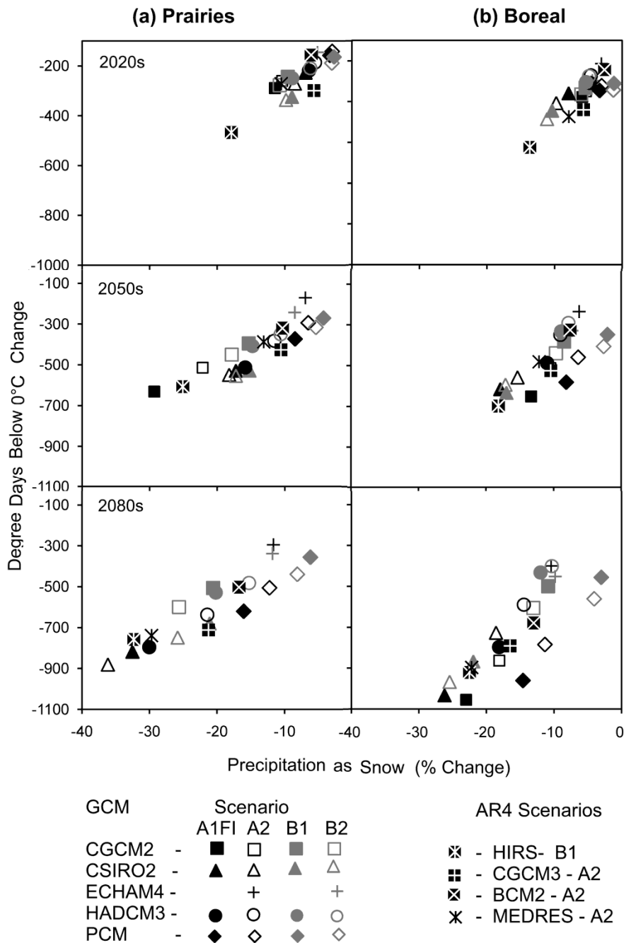
Figure 2-13. Relative change in projected precipitation as snow and degree days below 0°C for Prairies (A) and the southern Boreal (B) western Canada biomes based on ensemble runs of 4 SRES scenario families and 5 general circulation models, as well as 4 individual model runs selected from the IPCC's Fourth assessment Report (AR4) for the 2020s, 2050s and the 2080s.
